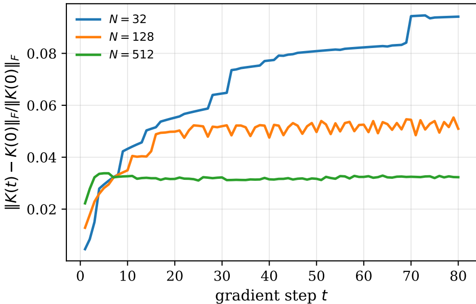
NTK motion vs width ( \gamma_0 = 0.15 )
