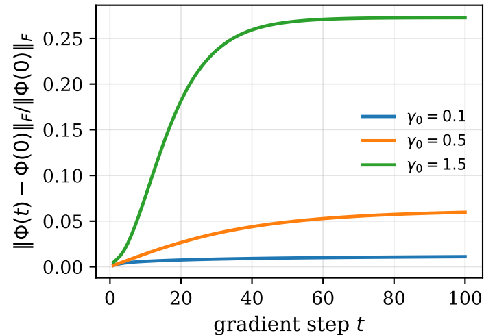
feature-kernel drift
