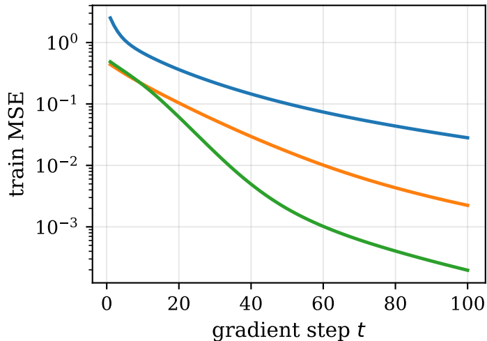
training loss
