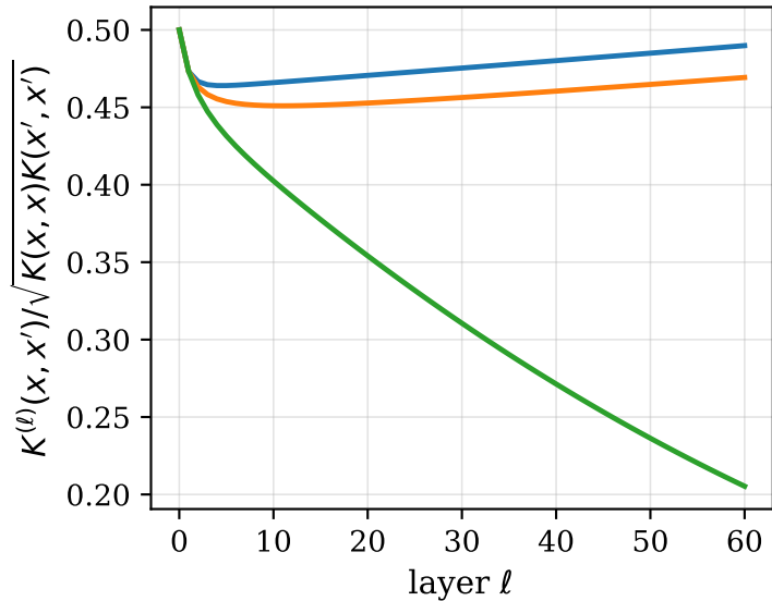
kernel cosine, init c = 0.5
