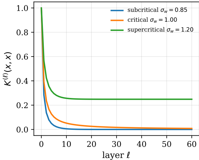
kernel variance, tanh
