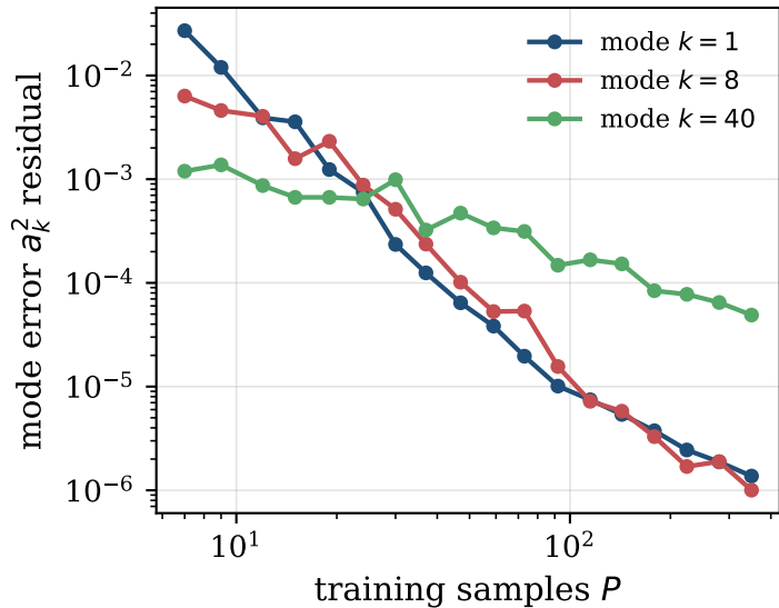
spectral bias
