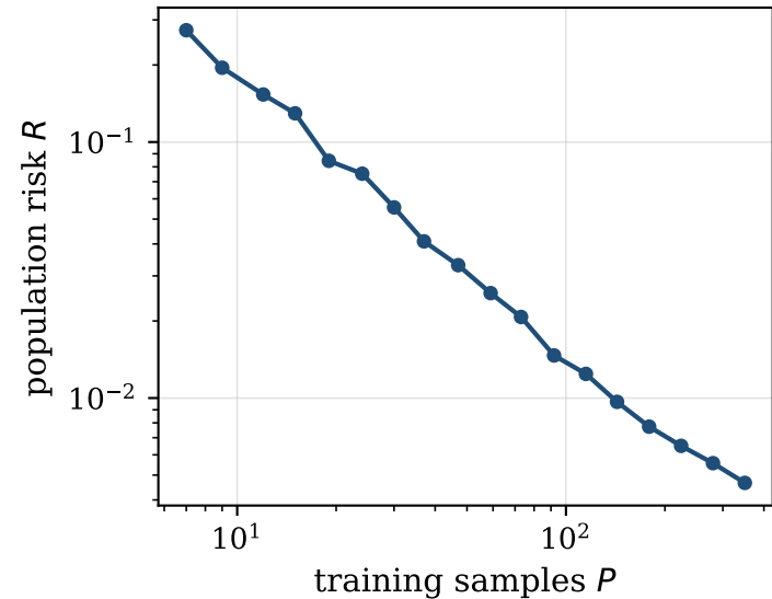
kernel ridge, \lambda_k \propto k^{-3/2}
