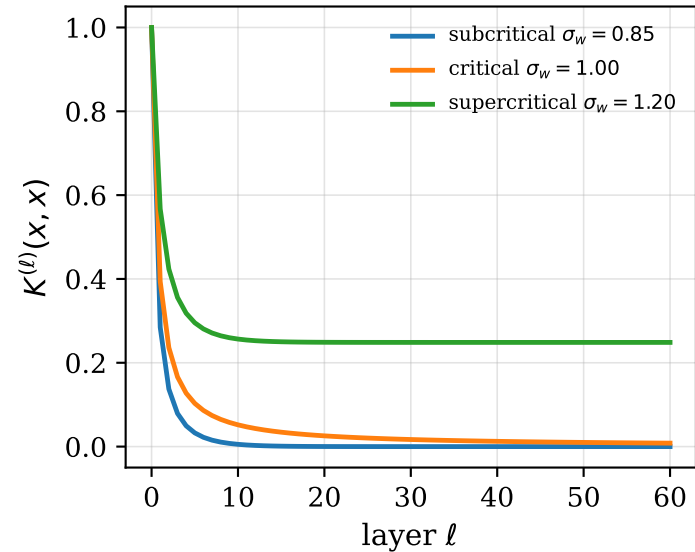
kernel variance, tanh
