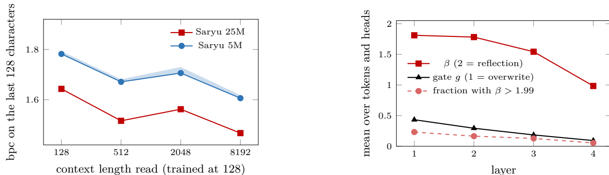
Figure 6: Left: bits per character as the model reads longer context than it was trained on; the shaded band is the three-seed spread of the 5M base recipe. Right: what the 25M model’s transports do on evaluation text (four windows of 1,024 characters): lower layers are close to exact reflections and rewrite often, the top layer uses softer transforms and rewrites rarely.
