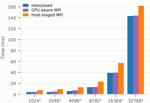
Stencil time (4 GPUs)
