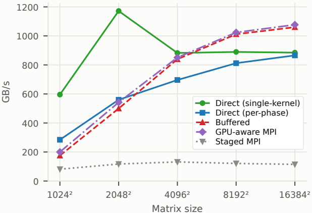
IPC — With Accumulation ( B += A^T )
