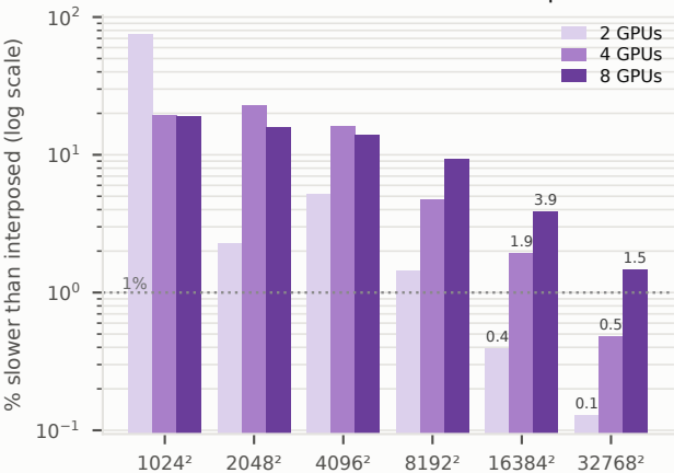
GPU-aware MPI overhead vs interposed
