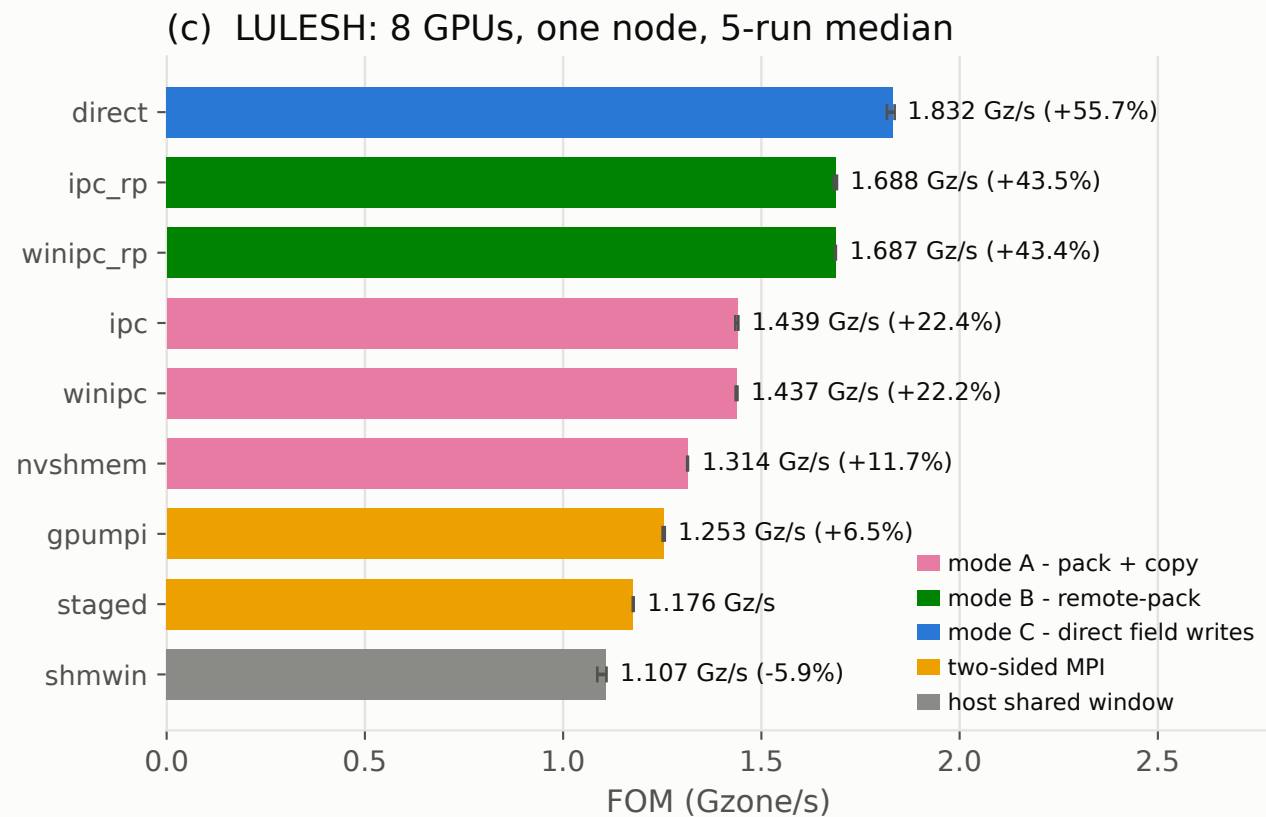
(a)-(c) H200 SXM (NVSwitch), single node. Transpose and stencil are Parallel Research Kernels benchmarks; (c) whiskers span min to max over the 5 runs.
