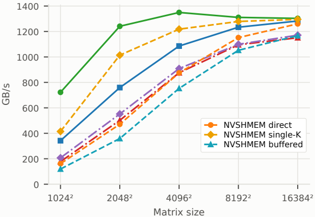
IPC vs NVSHMEM — No Accumulation
