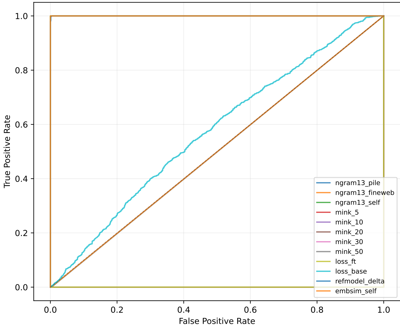
ROC — per detection method (GT variants A-C)
