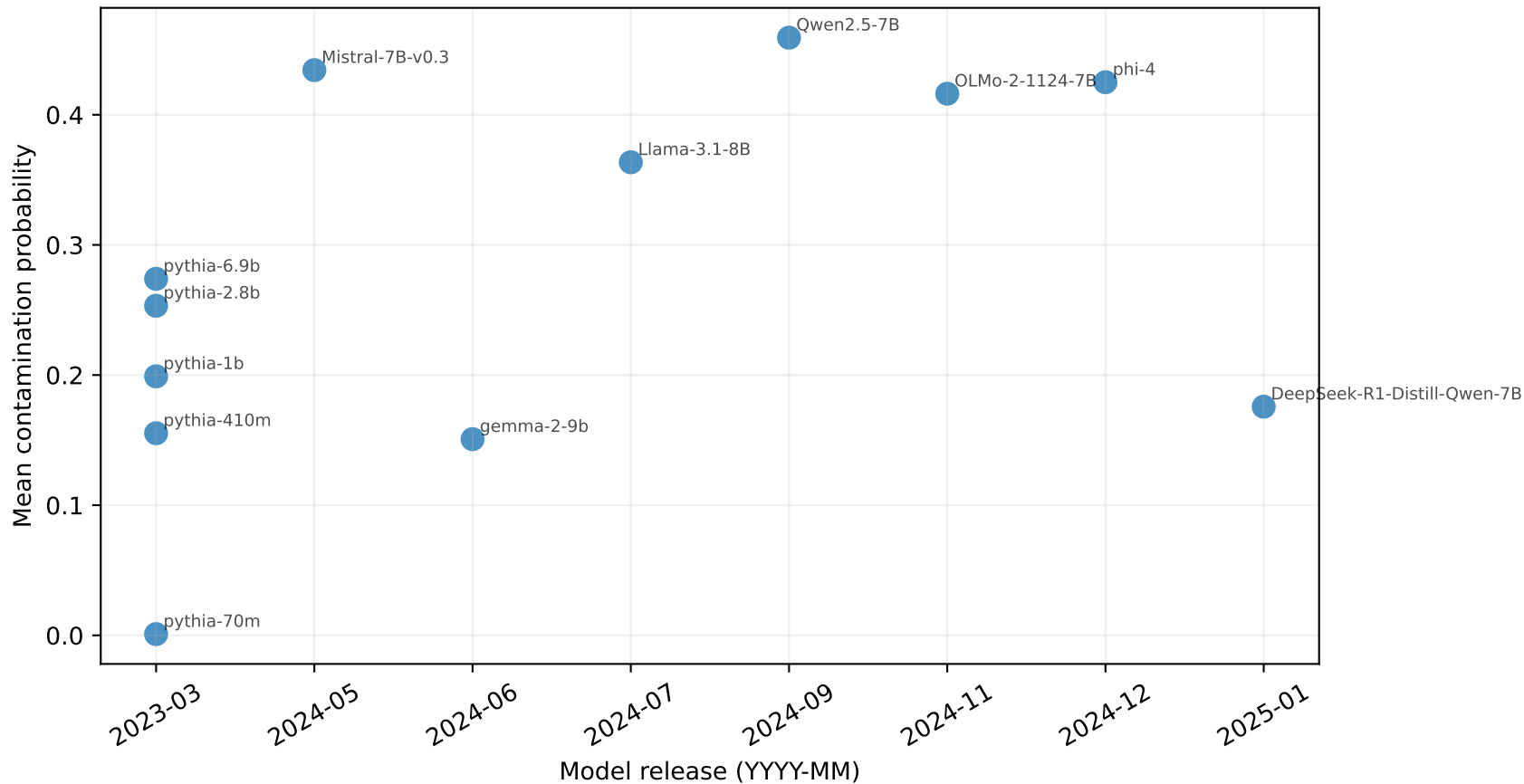
Benchmark contamination vs. model release date
