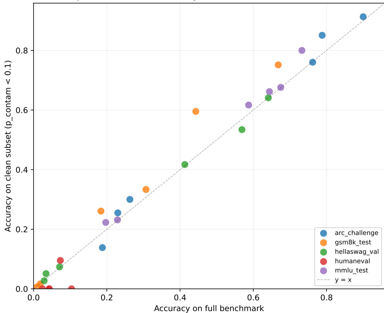
Reported vs. clean accuracy — contamination inflates scores
