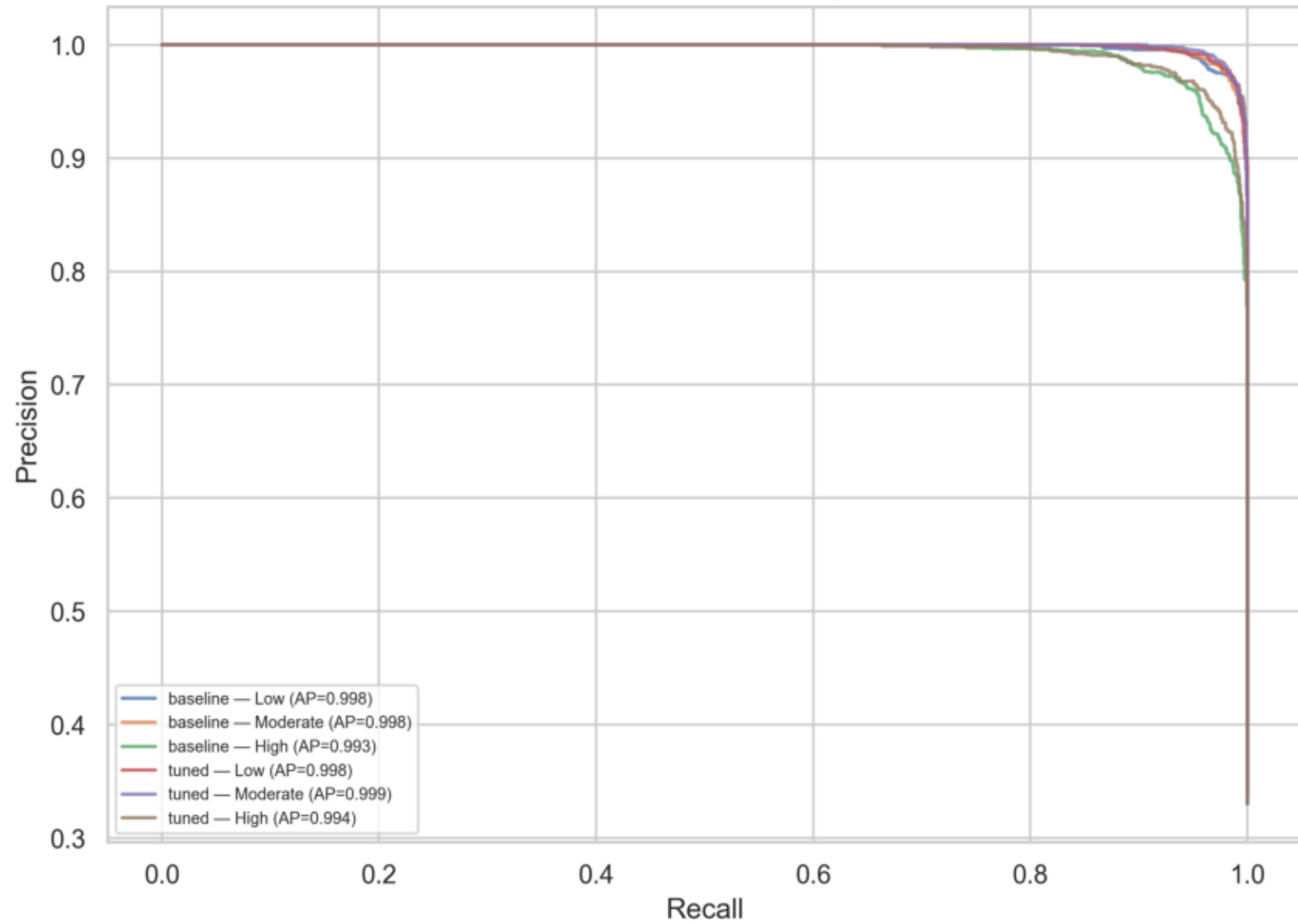
Precision-Recall Curves: xgboost
