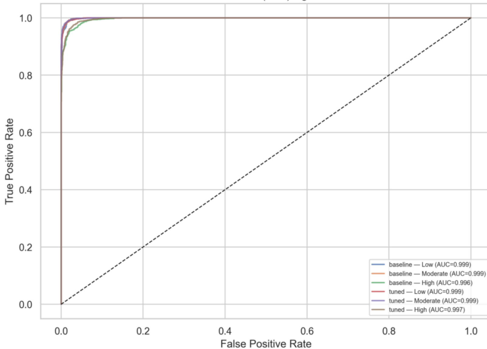
ROC Curves (OvR): xgboost
