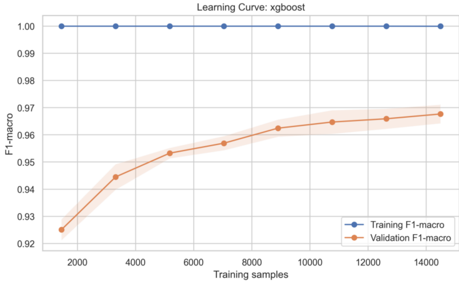
Learning Curve Xgboost
