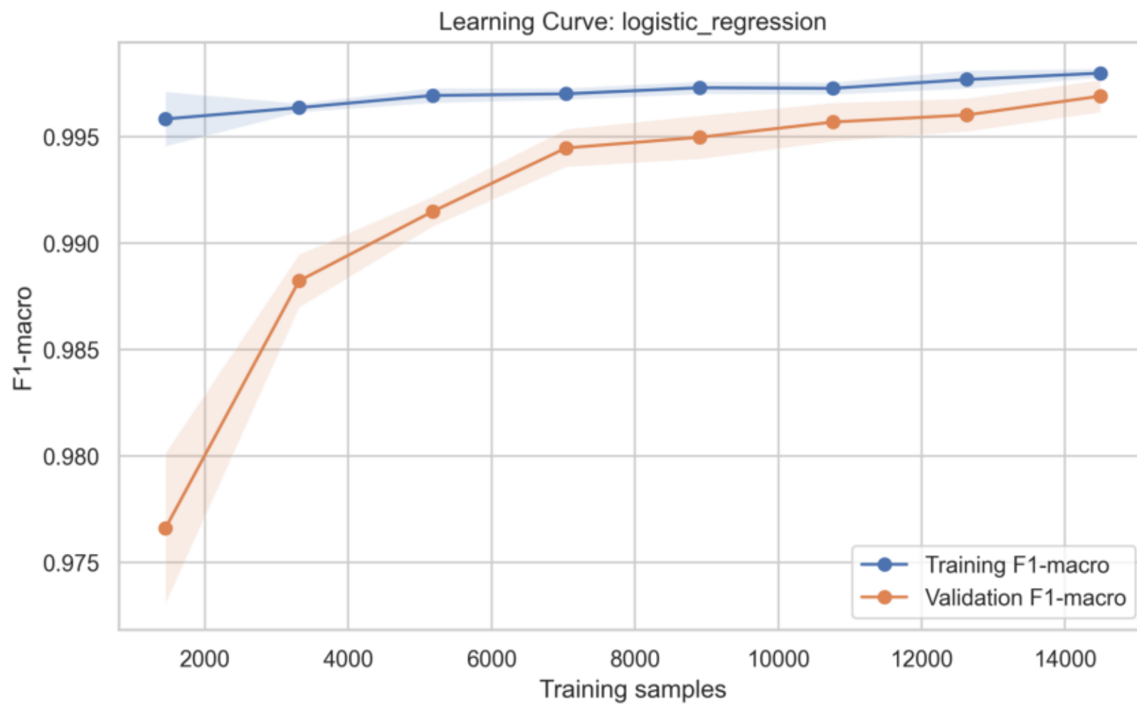
Learning Curve Logistic Regression
