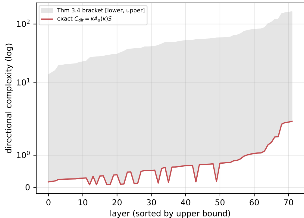
Thm 3.4: exact C_{\text{dir}} inside bracket (MNLI/DoRA; 0/2592 violations overall)
