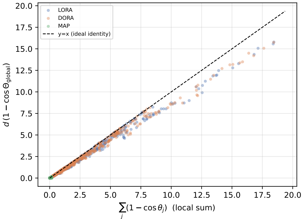
Thm 3.10: local sum vs scaled global angle (2592 layers, R^2=0.995 , slope=0.89)
