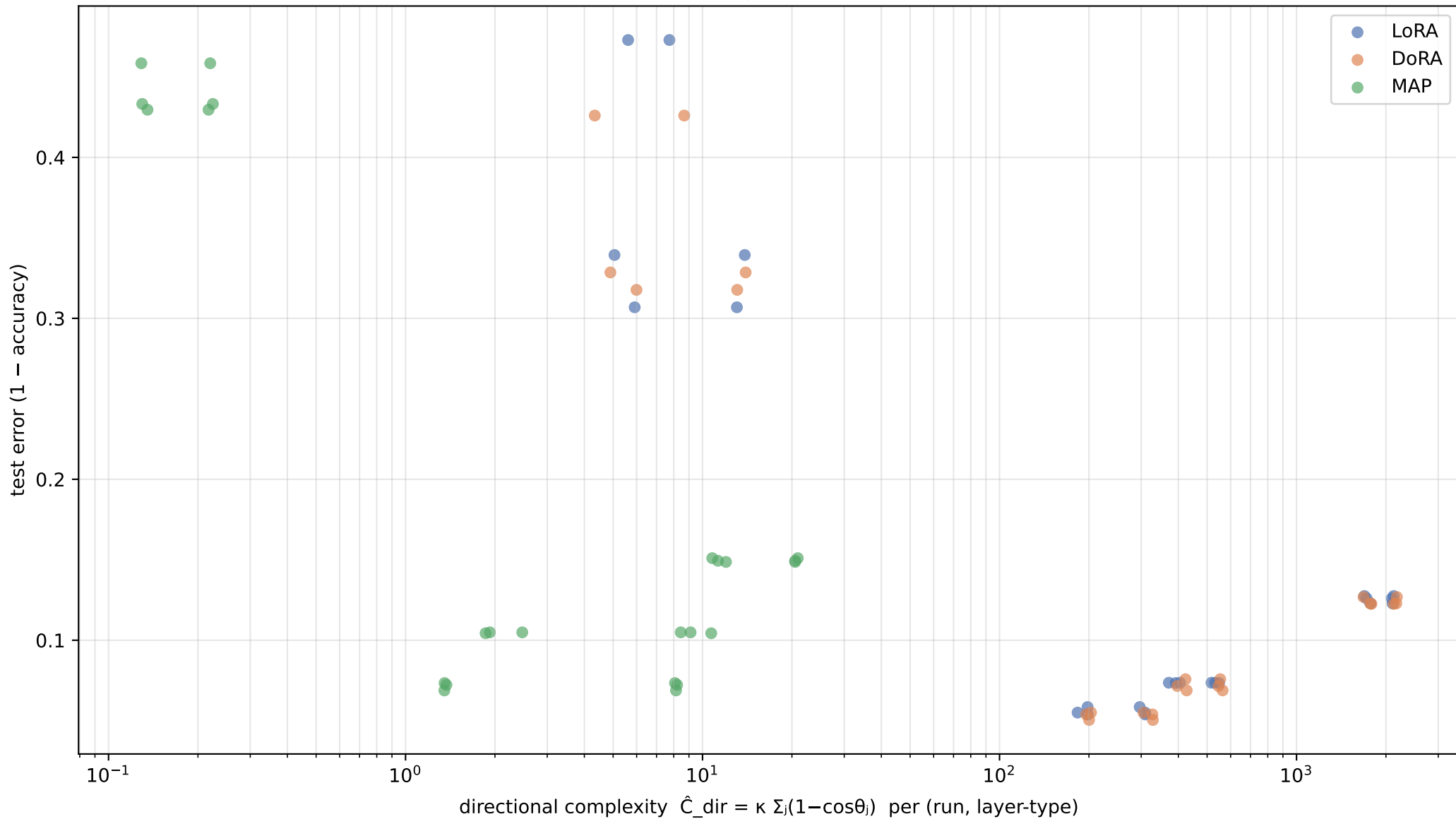
P1: directional complexity vs test error (pooled, n=72 points) Spearman \rho = -0.366 ( p=0.0016 ) | Pearson( \ln \hat{C} ) \rho = -0.639 ( p=1.6e-09 )
