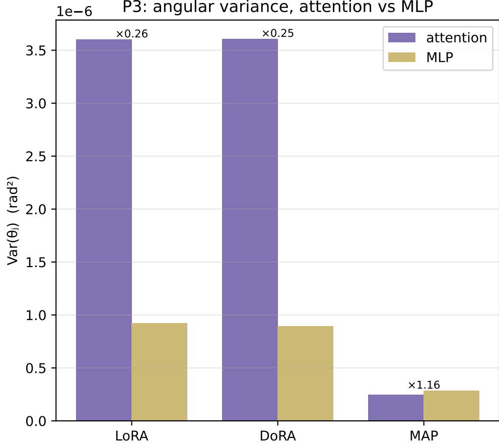
P3: angular variance, attention vs MLP
