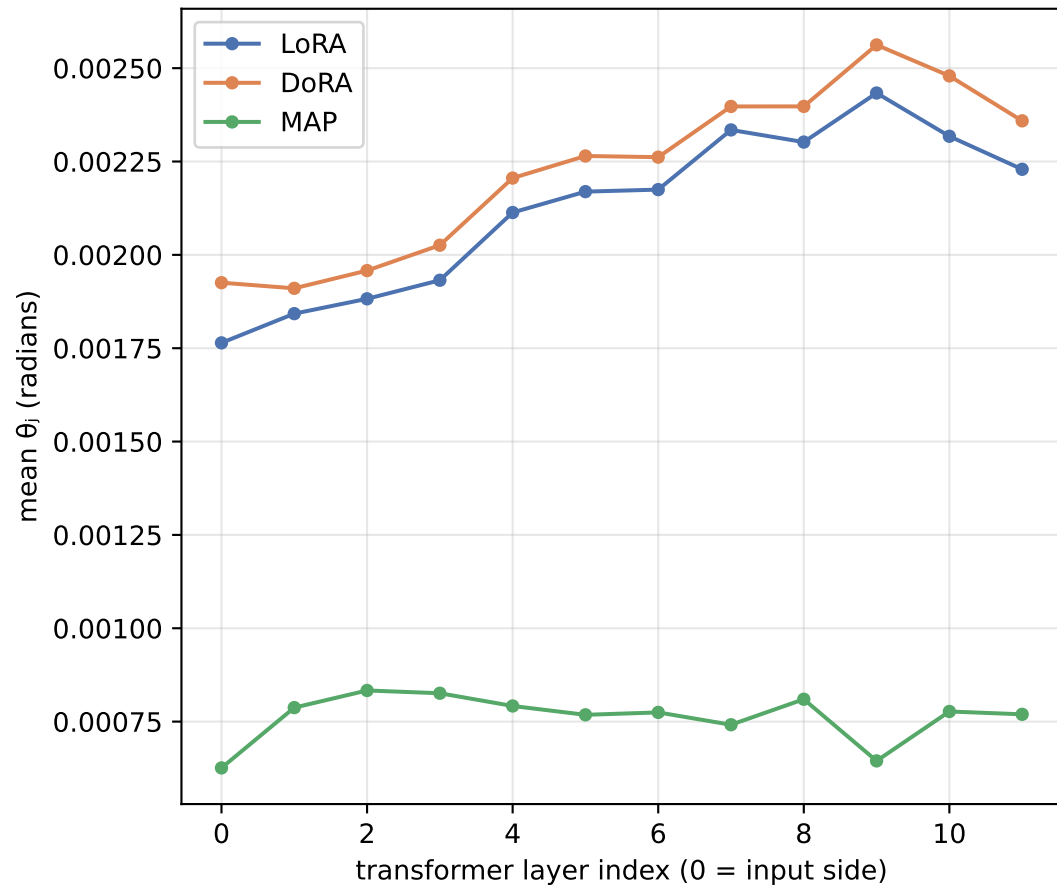
Mean per-column angle across depth
