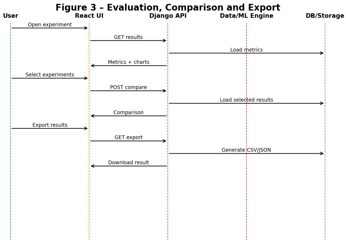
Figure 3. Evaluation, comparison and result export sequence.
