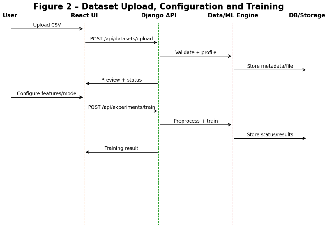
Figure 2. Dataset upload, configuration and training sequence.
