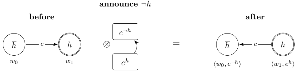
Figure 4: Alice’s lie, worked through. Only the two designated events survive at each world, since pre(e^{\neg h}) = \neg h holds only at w_0 and pre(e^h) = h only at w_1 . The event arrow is the FPN edge of Figure 3, which for Carol makes e^{\neg h} strictly the more plausible event. Carol’s world arrow has consequently reversed : she now finds the \neg h world the more plausible, so B_{carol} \neg h holds. Her knowledge is untouched—both worlds are still present and still comparable—which is why peek_c() can later restore the truth.
