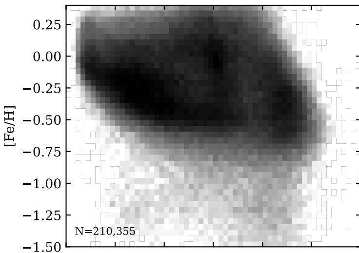
XD model, convolved with errors
