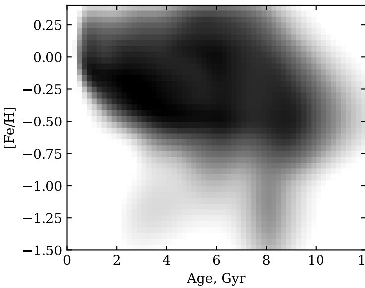
XD model, convolved with errors
