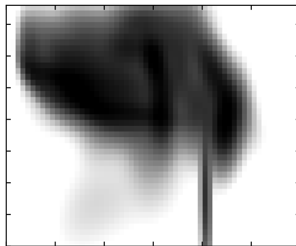
Data - convolved model, \chi^2/N_{\text{bin}} = 3.82 ( N_{\text{model}} > 5 )
