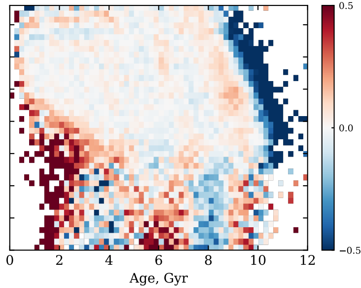
Data - convolved model, \chi^2/N_{\text{bin}} = 3.82 ( N_{\text{model}} > 5 )
