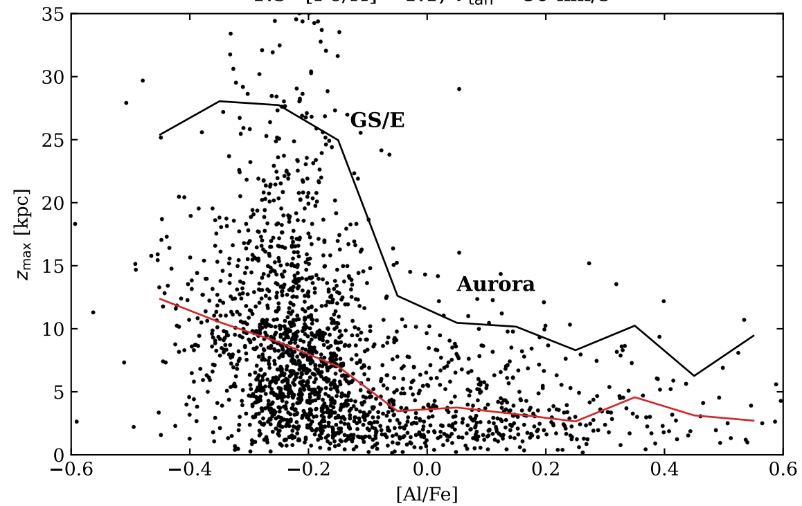
-1.5 < [\text{Fe}/\text{H}] < -1.1 , V_{\text{tan}} < 80 km/s
