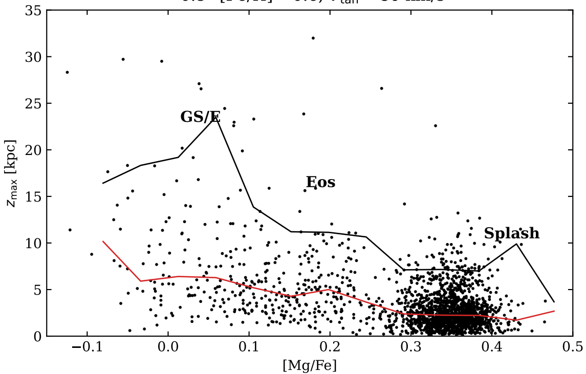
-0.8 < [\text{Fe}/\text{H}] < -0.6 , V_{\text{tan}} < 80 km/s
