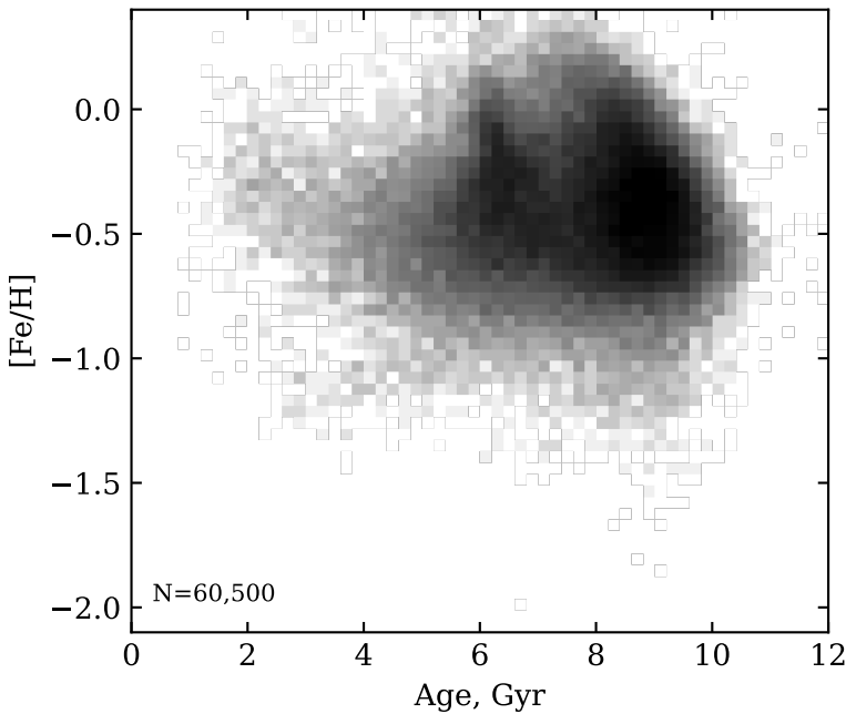
high- \alpha
