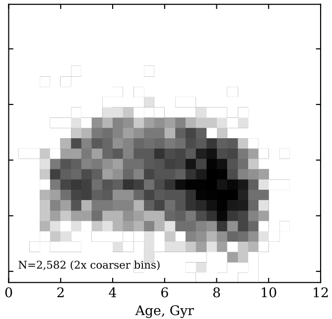
accreted (GS/E)
