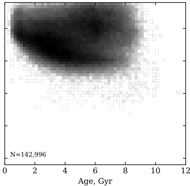
low- \alpha
