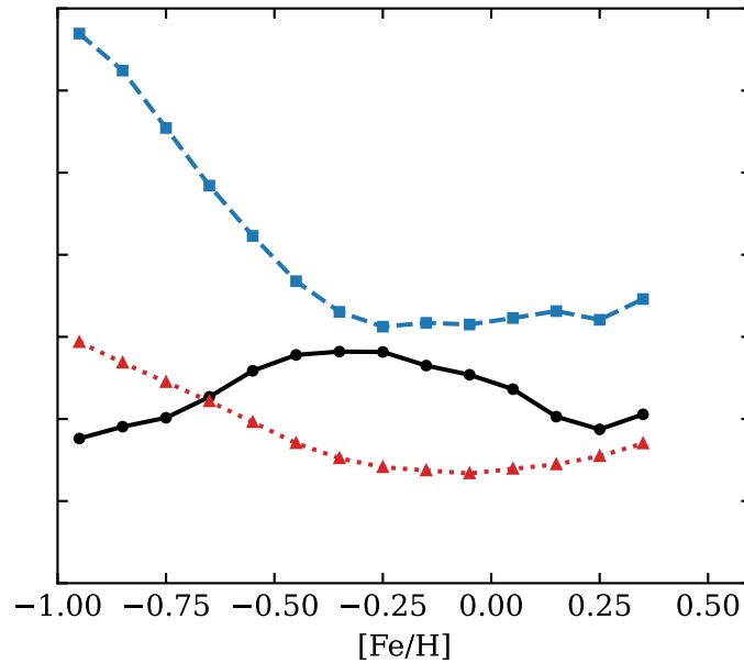
high- \alpha
