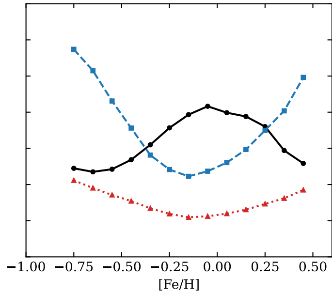
low- \alpha
