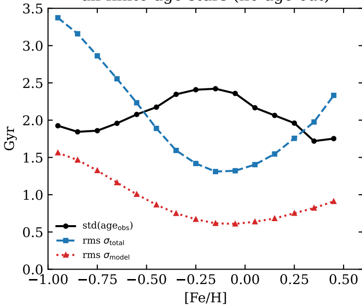
all finite-age stars (no age cut)
