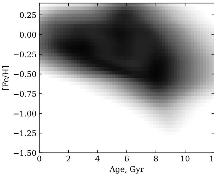
XD model, convolved with errors
