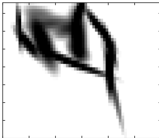
XD model, deconvolved ( K=20 )
