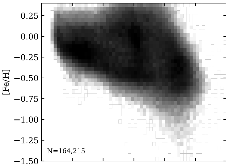
XD model, convolved with errors
