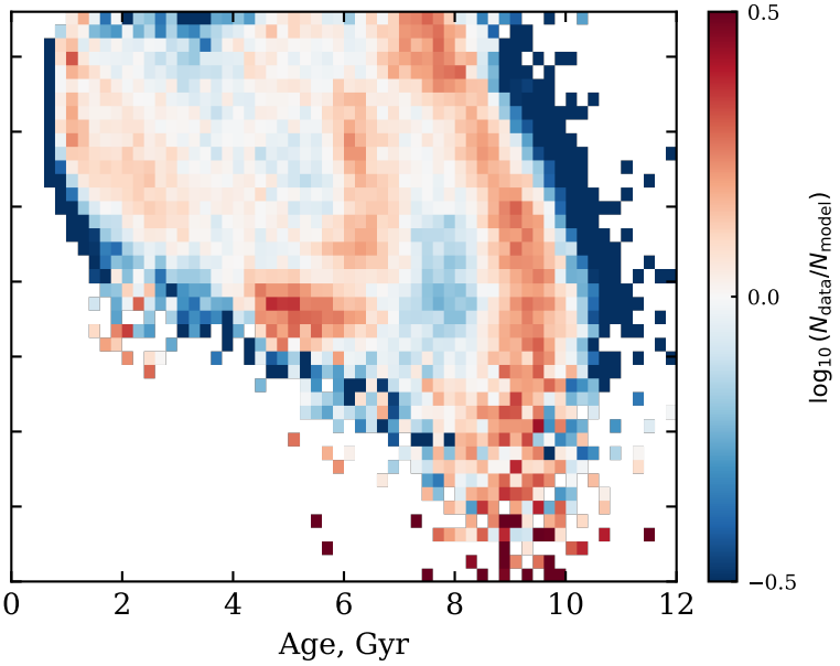
Data – convolved model, \chi^2/N_{\text{bin}} = 12.92 ( N_{\text{model}} > 5 )
