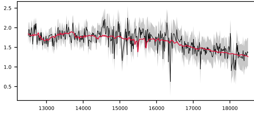
-619306399478533831, 7.3' S/N 16, LSF 16 Å, GALAXY, z = 0.408 , \Delta\chi^2=6 , \chi^2_r=0.9
