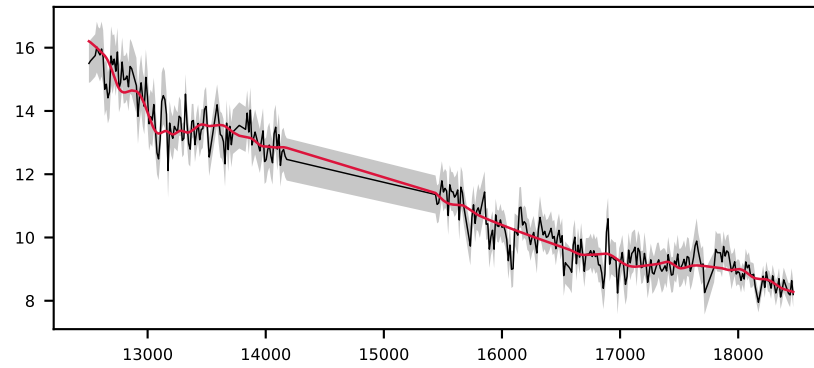
-618712980478566332, 9.5' S/N 31, LSF 19 Å, GALAXY, z = 0.104 , \Delta\chi^2=2 , \chi^2_r=0.1
