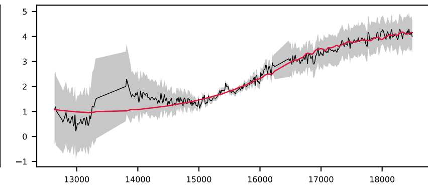
-620487523478800504, 2.3' S/N 16, LSF 22 Å, STAR, v = -600 km/s, \Delta\chi^2=\text{inf} , \chi^2_r=0.4
