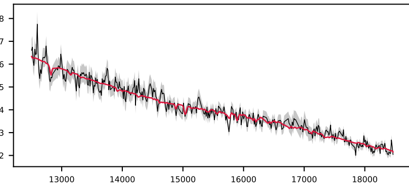
-622414746479163550, 5.8' S/N 37, LSF 12 Å, STAR, v = +0 km/s, \Delta\chi^2=\text{inf} , \chi^2_{\text{r}}=0.8
