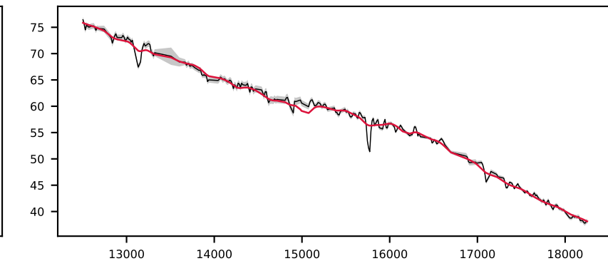
-619631044477912093, 8.4' S/N 226, LSF 48 Å, STAR, v = +150 km/s, \Delta\chi^2=\text{inf} , \chi^2_r=2.1
