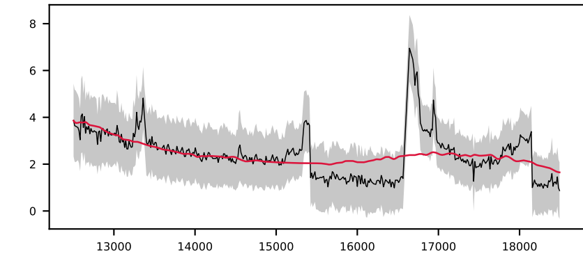
-622174637479100238, 4.8' S/N 19, LSF 12 Å, GALAXY, z = 0.953 , \Delta\chi^2=4 , \chi^2_r=0.4
