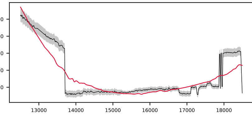
-620813322478693900, 1.8' S/N 62, LSF 14 Å, GALAXY, z = 0.112 , \Delta\chi^2=51 , \chi^2_r=9.3
