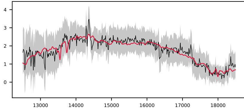
-619979314478539513, 4.9' S/N 16, LSF 12 Å, STAR, v = -150 \text{ km/s} , \Delta\chi^2=\text{inf} , \chi^2_r=1.0
