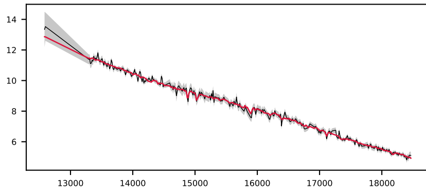
-622660498478729582, 6.8' S/N 61, LSF 12 Å, STAR, v = +0 km/s, \Delta\chi^2=\text{inf} , \chi^2_r=0.7
