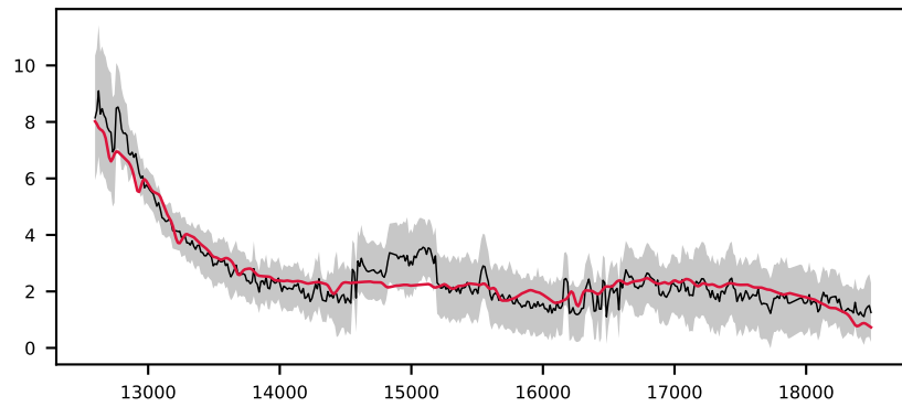
-621534683479076819, 2.2' S/N 19, LSF 14 Å, GALAXY, z = 0.734 , \Delta\chi^2=2 , \chi^2_r=0.1
