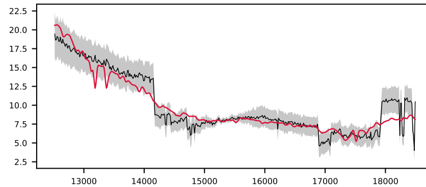
-621531101477739161, 7.7' S/N 59, LSF 12 Å, STAR, v = +0 km/s, \Delta\chi^2=\text{inf} , \chi^2_r=1.0
