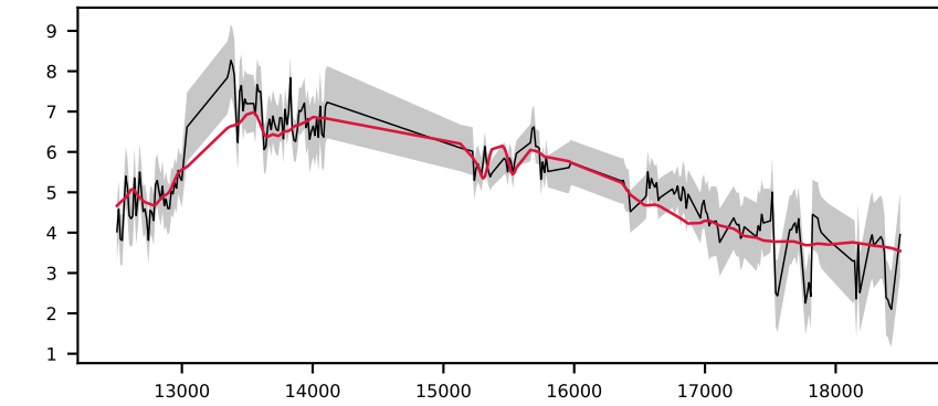
-619818404477602351, 9.5' S/N 20, LSF 12 Å, GALAXY, z = 0.277 , \Delta\chi^2=6 , \chi^2_r=0.3
