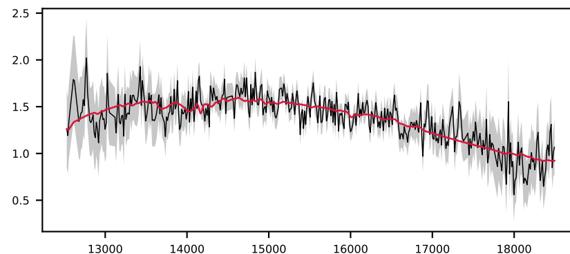
-621618592478981956, 2.5' S/N 12, LSF 19 Å, GALAXY, z = 0.249 , \Delta\chi^2=1 , \chi^2_r=0.6
