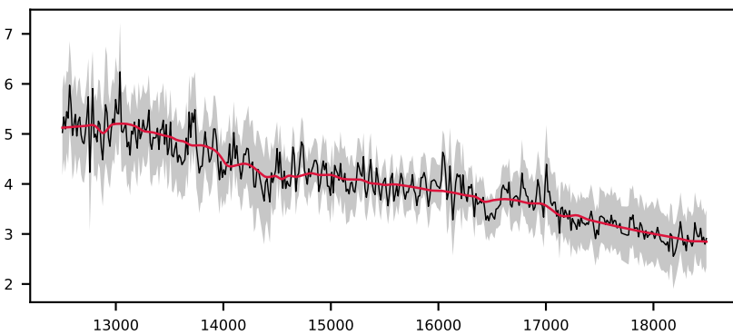
-619097308477976281, 9.7' S/N 23, LSF 35 Å, GALAXY, z = 0.022 , \Delta\chi^2=6 , \chi^2_r=1.3
