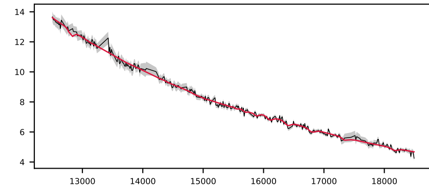
-620971747479254571, 1.7' S/N 58, LSF 14 Å, STAR, v = -600 km/s, \Delta\chi^2=\text{inf} , \chi^2_r=2.4
