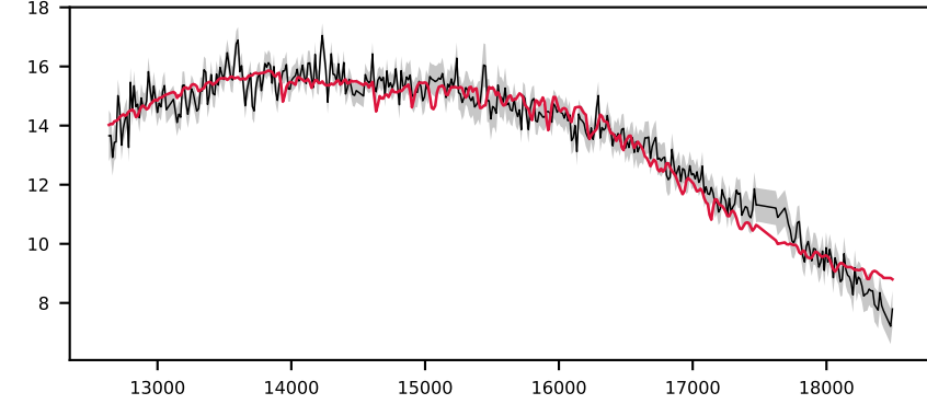
-622414746479163550, 5.8' S/N 37, LSF 12 Å, STAR, v = +0 km/s, \Delta\chi^2=\text{inf} , \chi^2_{\text{r}}=0.8
