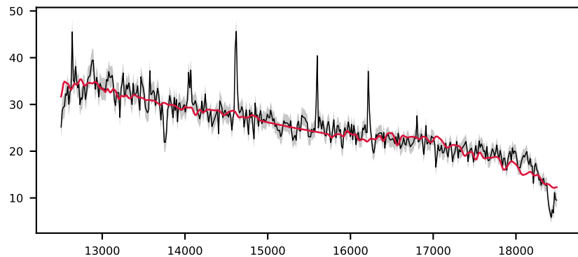
-620770055478797973, 1.4' S/N 127, LSF 18 Å, STAR, v = +150 km/s, \Delta\chi^2=\text{inf} , \chi^2_r=4.5
