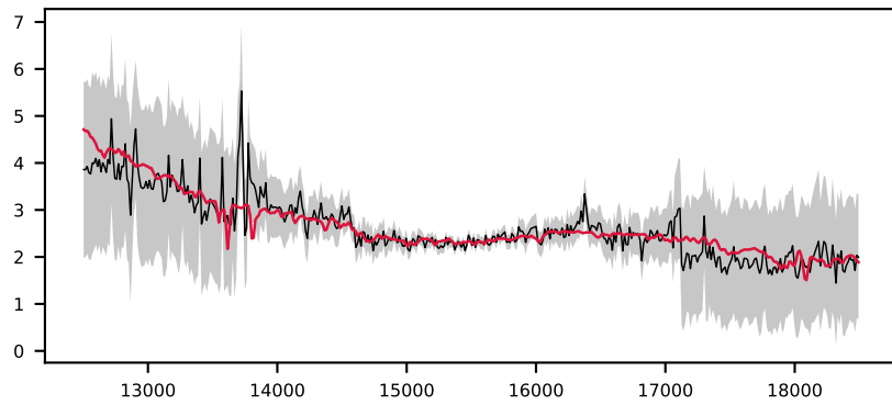
-619347635478453361, 7.4' S/N 22, LSF 18 Å, GALAXY, z = 0.260 , \Delta\chi^2=1 , \chi^2_{\text{r}}=0.1
