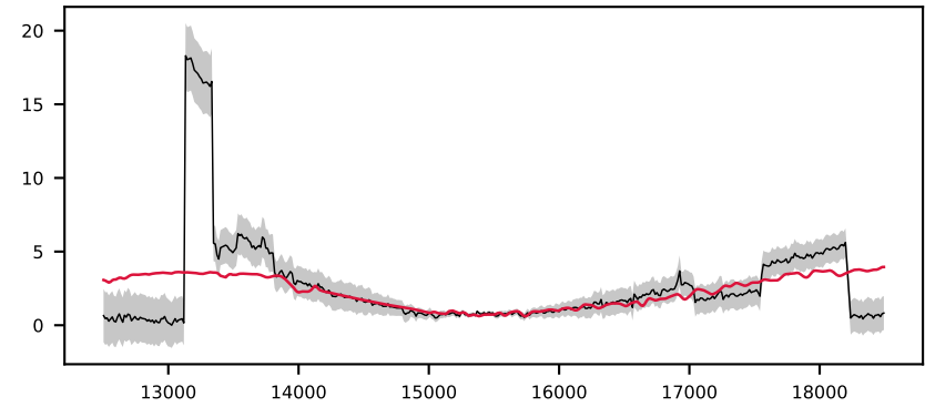
-620713897478690701, 2.0' S/N 15, LSF 18 Å, STAR, v = -600 km/s, \Delta\chi^2=\text{inf} , \chi^2_{\text{r}}=0.6
