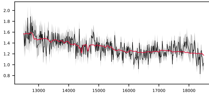
-619756067479868658, 7.4' S/N 12, LSF 40 Å, GALAXY, z = 0.368 , \Delta\chi^2=1 , \chi^2_r=0.6
