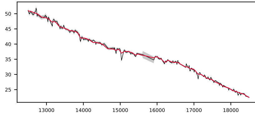
-621211920478703554, 1.8' S/N 161, LSF 24 Å, GALAXY, z = 0.029 , \Delta\chi^2=104 , \chi^2_r=1.3
