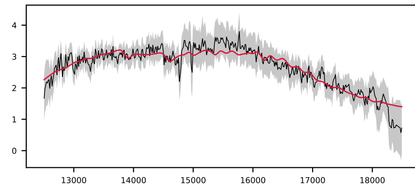
-621206313478639176, 2.1' S/N 21, LSF 15 Å, GALAXY, z = 0.905 , \Delta\chi^2=66 , \chi^2_r=8.0
