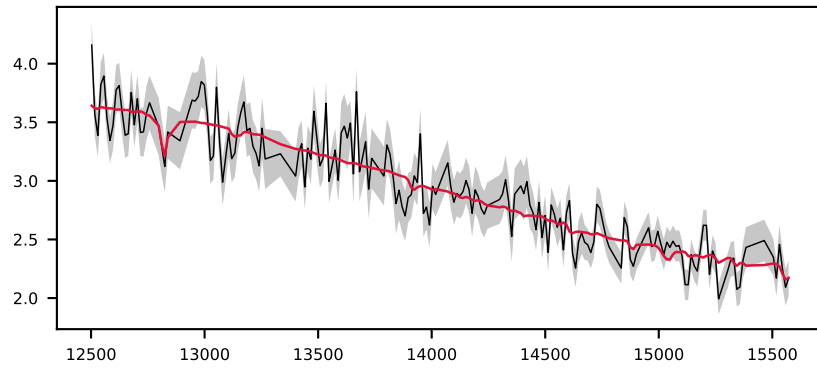
-621622776478577292, 3.4' S/N 19, LSF 27 Å, GALAXY, z = 0.190 , \Delta\chi^2=1 , \chi^2_r=0.1
