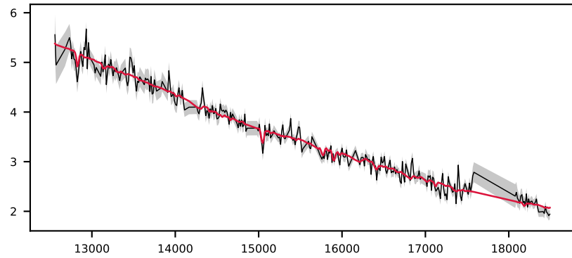
-620943516478649602, 1.9' S/N 32, LSF 12 Å, GALAXY, z = 0.892 , \Delta\chi^2=30 , \chi^2_r=20.3 ✗ unfittable
