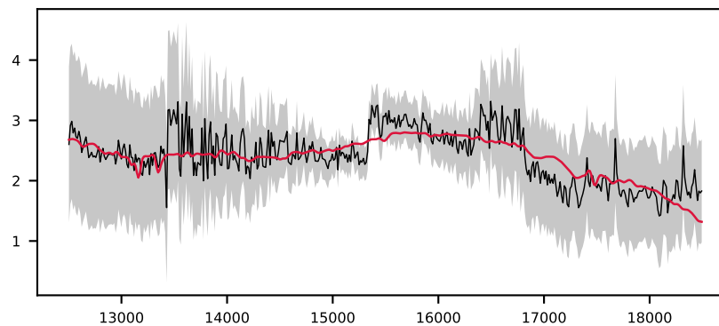
-620634222478648082, 2.4' S/N 22, LSF 14 Å, GALAXY, z = 0.149 , \Delta\chi^2=3 , \chi^2_r=0.3
