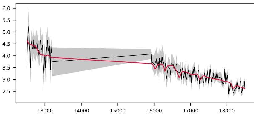
-621046139479621596, 3.9' S/N 16, LSF 18 Å, GALAXY, z = 0.040 , \Delta\chi^2=5 , \chi^2_r=0.1
