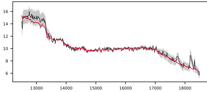
-620853207479275734, 1.9' S/N 62, LSF 13 Å, STAR, v = +600 km/s, \Delta\chi^2=\text{inf} , \chi^2_r=1.6
