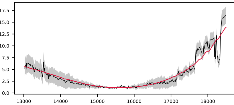
-621742842479729392, 5.4' S/N 18, LSF 12 Å, STAR, v = +150 km/s, \Delta\chi^2=\text{inf} , \chi^2_r=1.3
