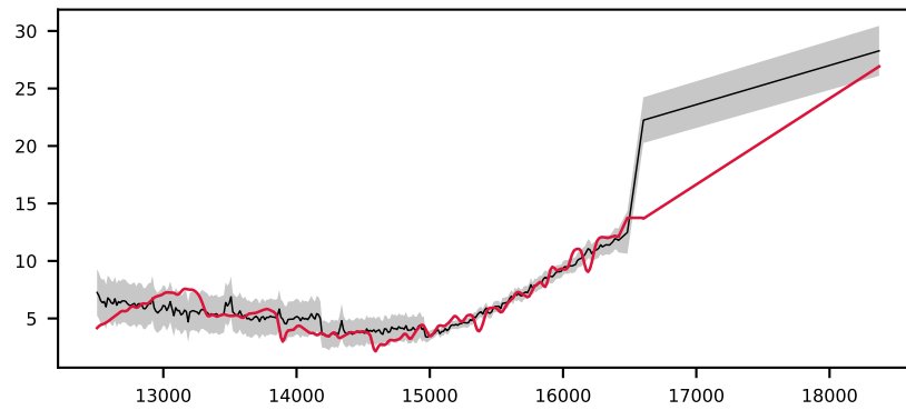
-620599741478205358, 4.9' S/N 33, LSF 12 Å, STAR, v = +150 km/s, \Delta\chi^2=\text{inf} , \chi^2_r=1.0
