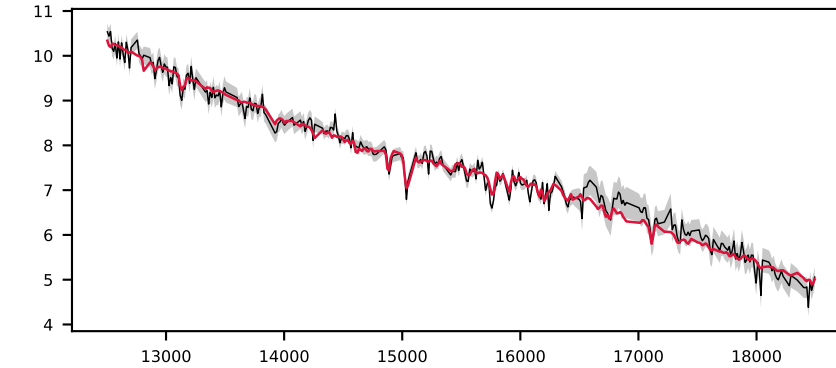
-622441419480150783, 9.1' S/N 58, LSF 13 Å, STAR, v = -150 km/s, \Delta\chi^2=\text{inf} , \chi^2_r=0.4
