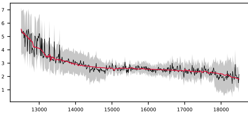
-622939837479010546, 7.8' S/N 24, LSF 24 Å, STAR, v = +450 km/s, \Delta\chi^2=\text{inf} , \chi^2_r=0.4
