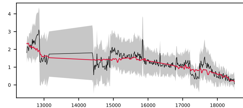
-620512848479501378, 3.8' S/N 12, LSF 12 Å, GALAXY, z = 0.899 , \Delta\chi^2=1 , \chi^2_r=0.5
