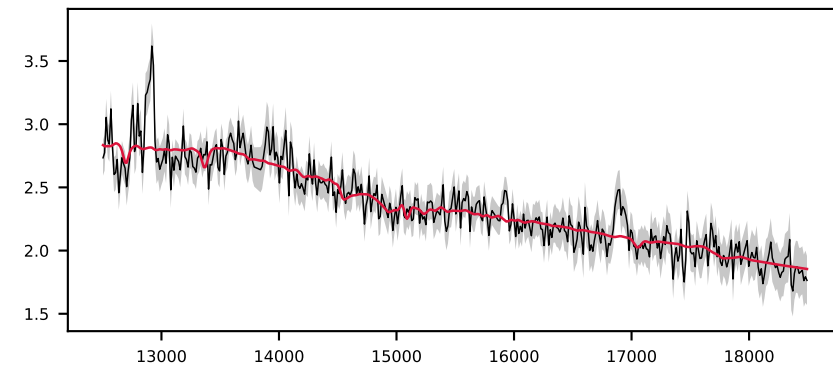
-622013802478949361, 4.1' S/N 24, LSF 22 Å, GALAXY, z = 0.196 , \Delta\chi^2=1 , \chi^2_r=0.1
