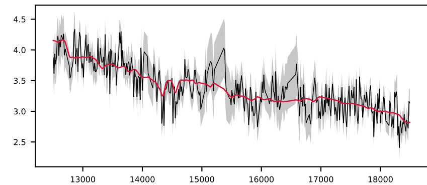
-619150751479423807, 7.9' S/N 20, LSF 28 Å, GALAXY, z = 0.679 , \Delta\chi^2=6 , \chi^2_r=0.9
