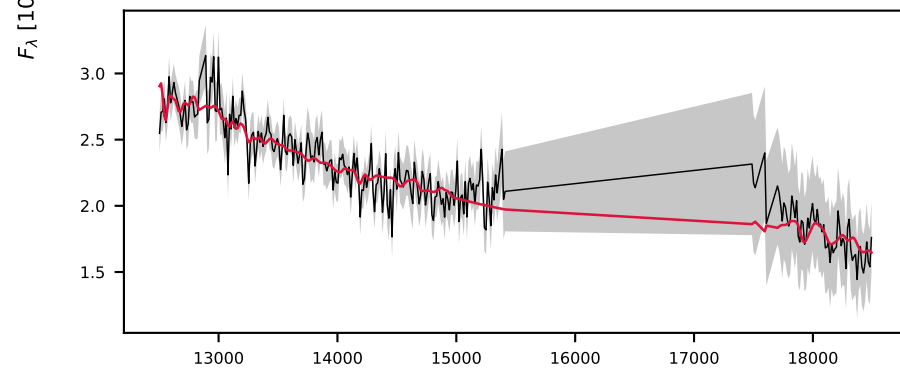
-620308533479025574, 2.8' S/N 16, LSF 13 Å, STAR, v = +150 km/s, \Delta\chi^2=\text{inf} , \chi^2_r=1.0
