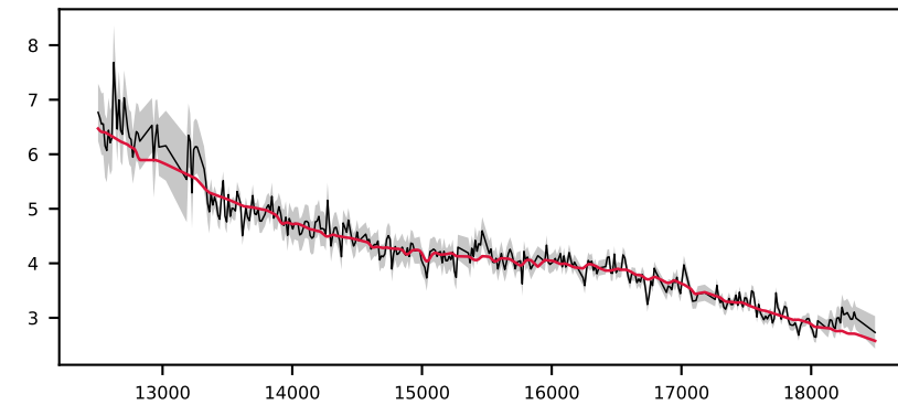
-619820919478543555, 5.4' S/N 31, LSF 16 Å, STAR, v = +0 km/s, \Delta\chi^2=\text{inf} , \chi^2_r=1.1
