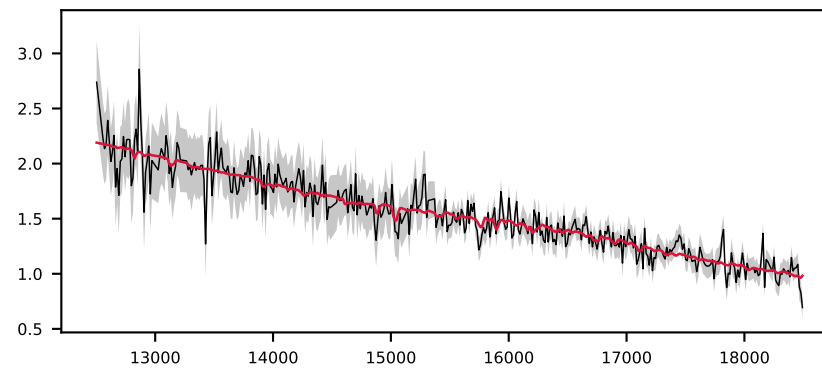
-621828742479520817, 4.7' S/N 16, LSF 12 Å, STAR, v = +150 km/s, \Delta\chi^2=\text{inf} , \chi^2_r=1.2
