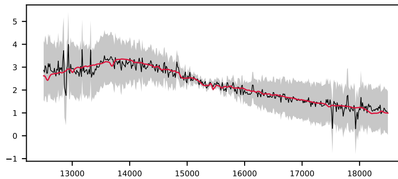
-621454814478653984, 2.6' S/N 21, LSF 16 Å, STAR, v = +300 km/s, \Delta\chi^2=\text{inf} , \chi^2_r=0.5
