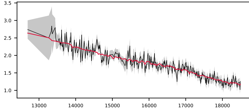
-622849900479329738, 7.7' S/N 16, LSF 19 Å, GALAXY, z = 0.618 , \Delta\chi^2=0 , \chi^2_r=0.7
