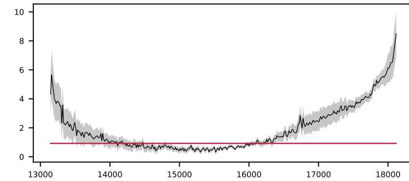
-619359929478797464, 6.7' S/N 12, LSF 15 Å, GALAXY, z = 0.875 , \Delta\chi^2=1 , \chi^2_r=0.5
