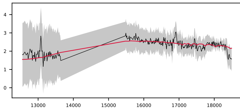
-623379823478654393, 9.7' S/N 18, LSF 17 Å, GALAXY, z = 1.001 , \Delta\chi^2=1 , \chi^2_r=0.1
