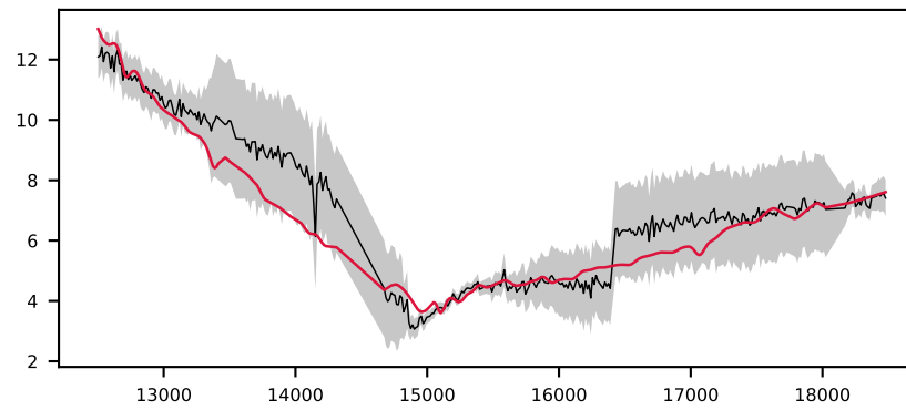
-622032035479474411, 5.1' S/N 43, LSF 31 Å, STAR, v = -600 km/s, \Delta\chi^2=\text{inf} , \chi^2_r=0.5
