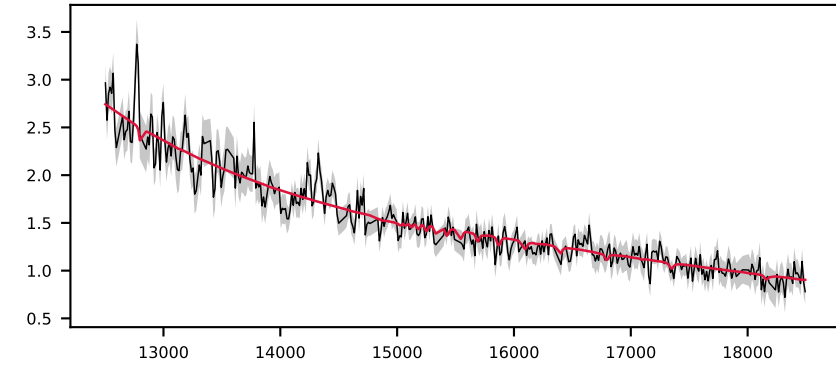
-620408699478923683, 2.4' S/N 13, LSF 13 Å, GALAXY, z = 0.482 , \Delta\chi^2=1 , \chi^2_r=0.1
