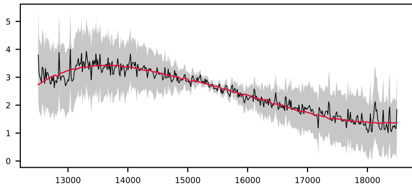
-619658068479189682, 5.6' S/N 23, LSF 21 Å, GALAXY, z = 0.686 , \Delta\chi^2=0 , \chi^2_r=0.5
