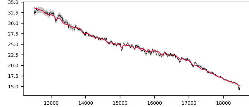
-621953533478944550, 3.8' S/N 109, LSF 30 Å, STAR, v = +150 km/s, \Delta\chi^2=\text{inf} , \chi^2_r=1.3
