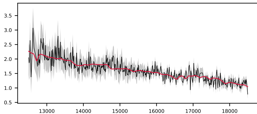
-621073271479629718, 4.0' S/N 12, LSF 23 Å, GALAXY, z = 0.030 , \Delta\chi^2=0 , \chi^2_r=0.2
