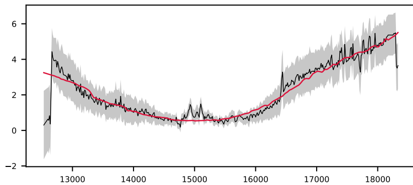
-620559511479273930, 2.6' S/N 16, LSF 18 Å, GALAXY, z = 0.282 , \Delta\chi^2=5 , \chi^2_r=0.1
