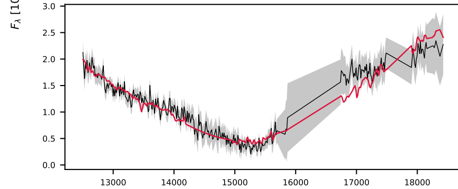
-618732774478693226, 9.3' S/N 12, LSF 17 Å, STAR, v = -600 km/s, \Delta\chi^2=\text{inf} , \chi^2_r=0.2
