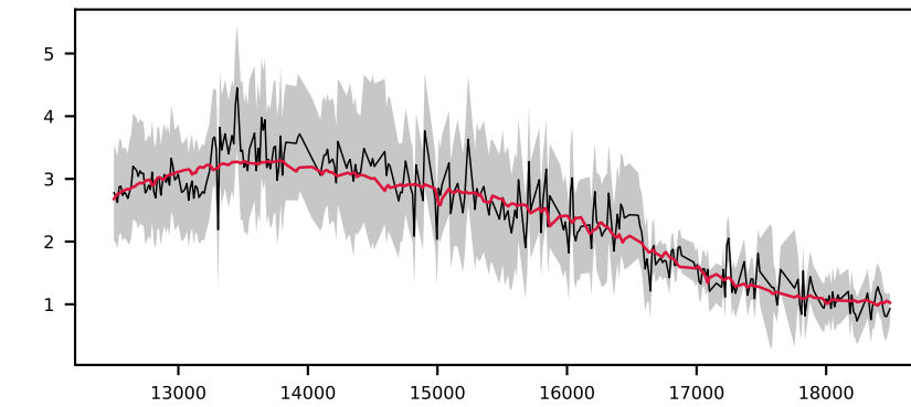
-620543831479647235, 4.5' S/N 18, LSF 13 Å, GALAXY, z = 0.288 , \Delta\chi^2=1 , \chi^2_r=0.2
