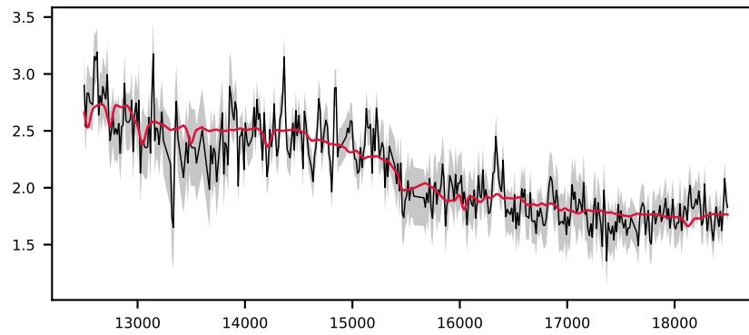
-620447112478897412, 2.3' S/N 15, LSF 13 Å, GALAXY, v = +0 km/s, \Delta\chi^2=0 , \chi^2_r=0.5
