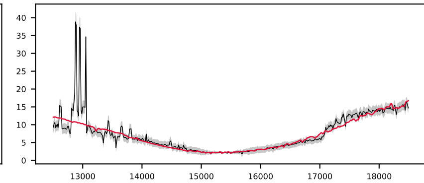
-622175078478213803, 6.5' S/N 54, LSF 13 Å, STAR, v = +150 km/s, \Delta\chi^2=\text{inf} , \chi^2_r=0.4
