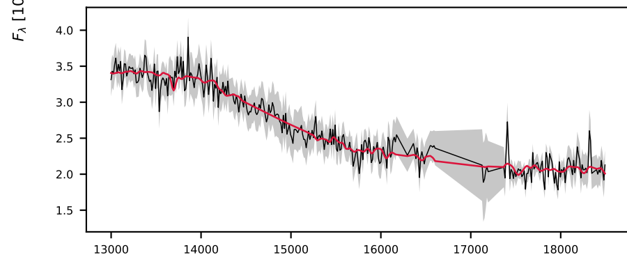
-620893614478413240, 3.4' S/N 24, LSF 27 Å, GALAXY, z = 1.001 , \Delta\chi^2=2 , \chi^2_r=0.1
