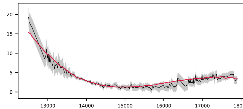
-620406281478436772, 4.0' S/N 16, LSF 12 Å, GALAXY, z = 0.376 , \Delta\chi^2=14 , \chi^2_r=0.7
