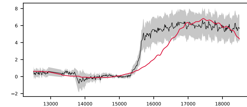
-621482089479311002, 2.8' S/N 16, LSF 9 Å, GALAXY, z = 0.589 , \Delta\chi^2=1 , \chi^2_r=0.3
