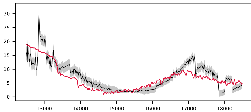
-620952016478658285, 1.9' S/N 42, LSF 14 Å, STAR, v = +600 km/s, \Delta\chi^2=\text{inf} , \chi^2_r=3.5
