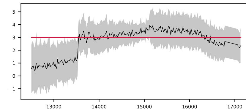
-620485820478910343, 2.1' S/N 24, LSF 20 Å, GALAXY, v = +0 km/s, \Delta\chi^2=0 , \chi^2_r=0.5
