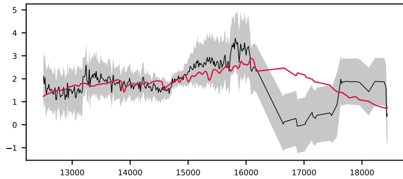
-619565020478014765, 8.1' S/N 15, LSF 12 Å, GALAXY, z = 0.445 , \Delta\chi^2=1 , \chi^2_r=1.1
