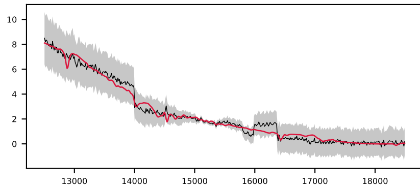
-623290721478629101, 9.4' S/N 16, LSF 23 Å, GALAXY, z = 0.808 , \Delta\chi^2=1 , \chi^2_r=0.6
