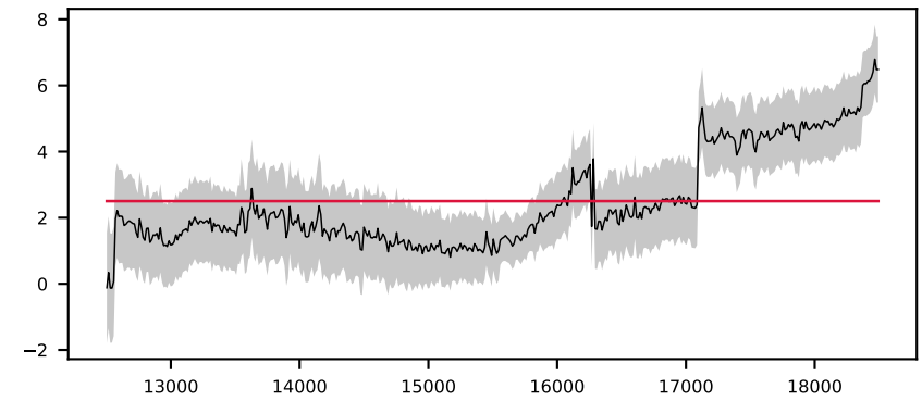
-620515876479249318, 2.6' S/N 15, LSF 25 Å, GALAXY, v = +0 km/s, \Delta\chi^2=0 , \chi^2_r=0.2
