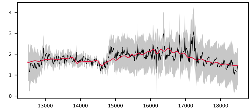
-619843510478118932, 6.9' S/N 15, LSF 47 Å, STAR, v = -600 km/s, \Delta\chi^2=\text{inf} , \chi^2_{\text{r}}=0.2
