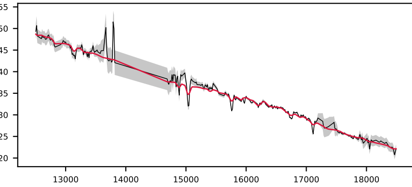
-620828930478794044, 1.3' S/N 149, LSF 12 Å, STAR, v = -600 km/s, \Delta\chi^2=\text{inf} , \chi^2_r=16.3
