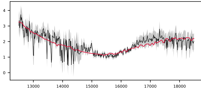
-619661186479345578, 5.9' S/N 16, LSF 25 Å, GALAXY, z = 0.586 , \Delta\chi^2=4 , \chi^2_r=0.1
