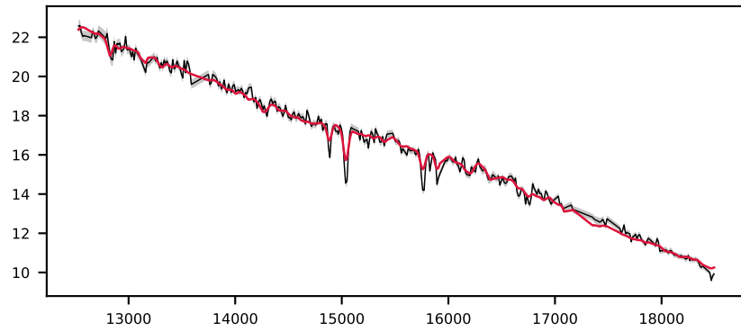
-620837920478728431, 1.6' S/N 86, LSF 23 Å, STAR, v = +600 km/s, \Delta\chi^2=\text{inf} , \chi^2_r=1.3
