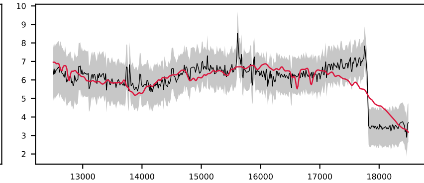
-619727943478828503, 5.2' S/N 53, LSF 15 Å, STAR, v = +0 km/s, \Delta\chi^2=\text{inf} , \chi^2_r=0.8
