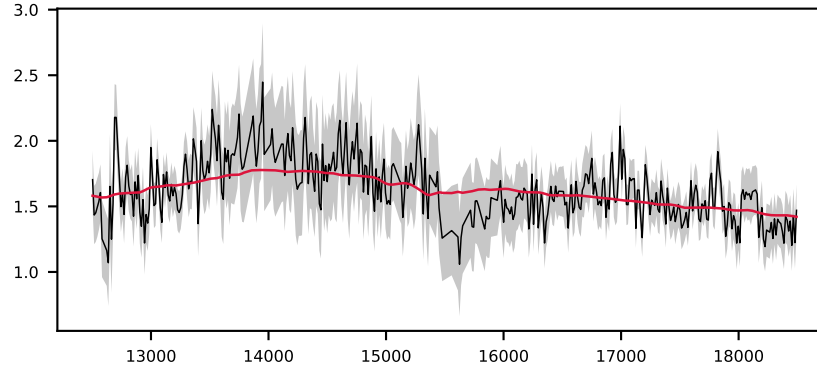
-620255421479309667, 3.6' S/N 12, LSF 13 Å, GALAXY, z = 0.203 , \Delta\chi^2=4 , \chi^2_r=1.1
