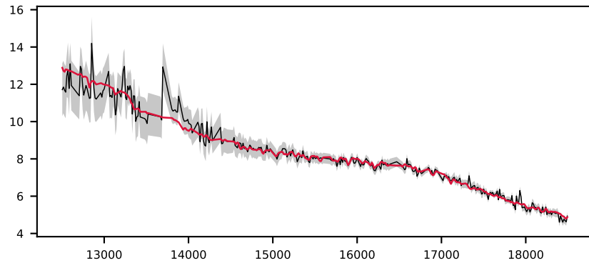
-620501291479703609, 4.8' S/N 58, LSF 12 Å, STAR, v = -150 km/s, \Delta\chi^2=\text{inf} , \chi^2_r=0.5
