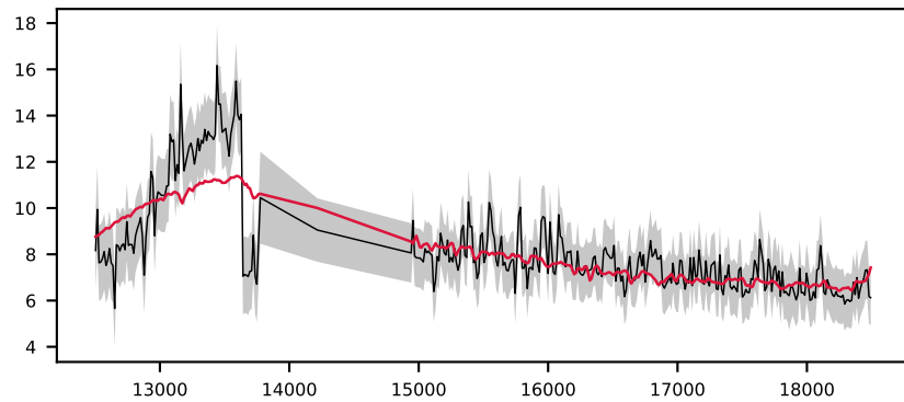
-620892754480403263, 8.6' S/N 59, LSF 12 Å, STAR, v = +0 km/s, \Delta\chi^2=\text{inf} , \chi^2_r=0.5
