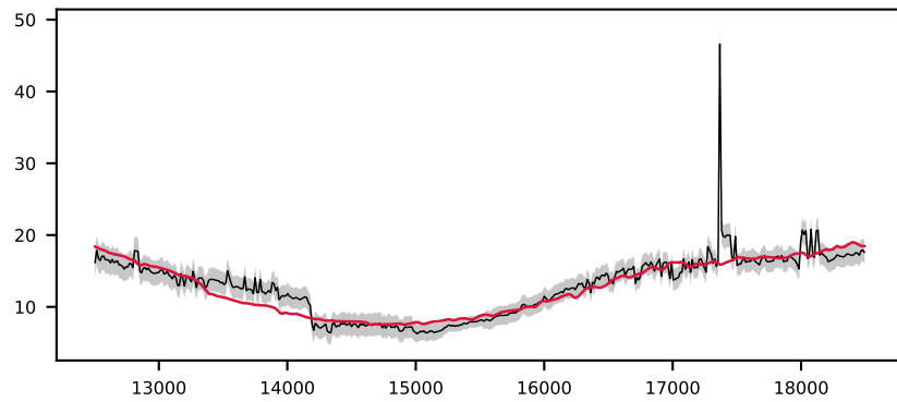
-620691186478799263, 1.6' S/N 84, LSF 19 Å, STAR, v = +0 km/s, \Delta\chi^2=\text{inf} , \chi^2_r=2.2
