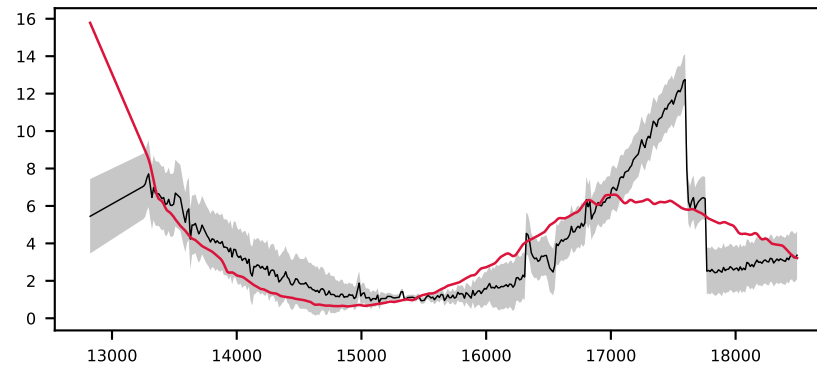
-620206426479071332, 3.3' S/N 23, LSF 26 Å, GALAXY, z = 0.799 , \Delta\chi^2=1 , \chi^2_r=0.7
