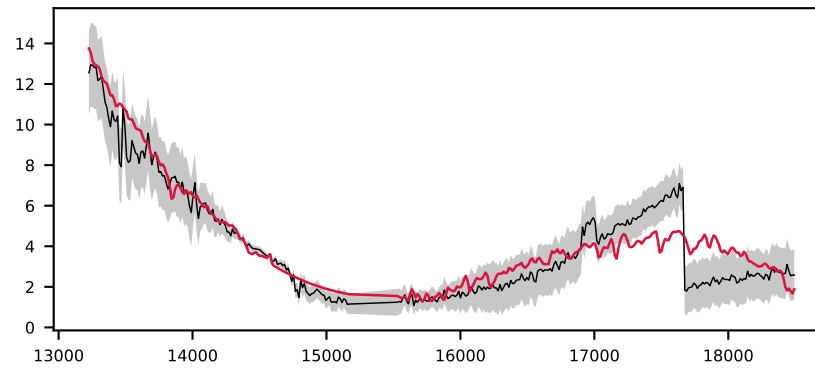
-621363607478609701, 2.6' S/N 22, LSF 14 Å, GALAXY, z = 0.093 , \Delta\chi^2=2 , \chi^2_{\text{r}}=0.4
