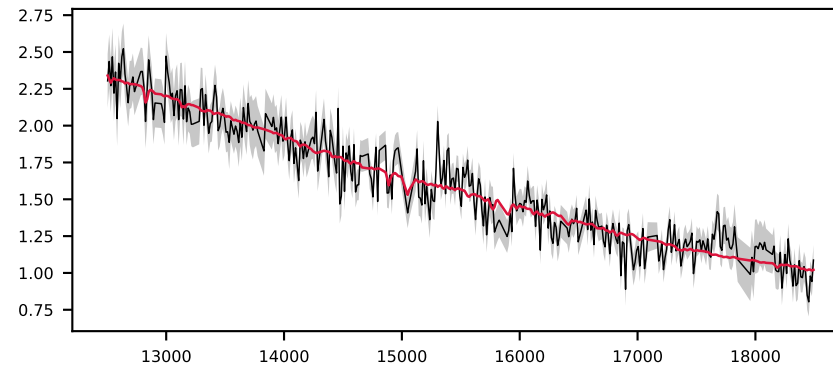
-620755132478634258, 2.3' S/N 16, LSF 18 Å, GALAXY, z = 0.073 , \Delta\chi^2=3 , \chi^2_r=0.4
