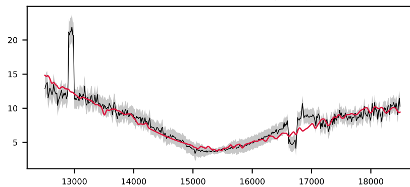
-618987366478081806, 9.7' S/N 73, LSF 12 Å, STAR, v = +150 km/s, \Delta\chi^2=\text{inf} , \chi^2_r=1.2
