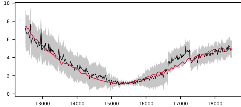
-621441518479877346, 5.7' S/N 28, LSF 16 Å, STAR, v = -600 km/s, \Delta\chi^2=\text{inf} , \chi^2_r=0.3
