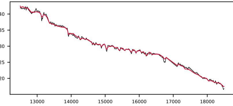
-621339078479795092, 5.1' S/N 159, LSF 52 Å, STAR, v = -150 km/s, \Delta\chi^2=\text{inf} , \chi^2_r=1.3
