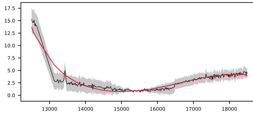
-620535315479379235, 3.1' S/N 19, LSF 12 Å, GALAXY, z = 0.066 , \Delta\chi^2=7 , \chi^2_r=0.4
