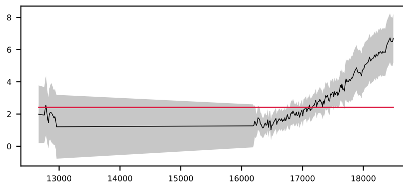
-620574815478659196, 2.5' S/N 22, LSF 22 Å, GALAXY, v = +0 km/s, \Delta\chi^2=0 , \chi^2_r=2.0
