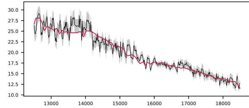
-619208419479975843, 9.4' S/N 117, LSF 29 Å, STAR, v = +150 km/s, \Delta\chi^2=\text{inf} , \chi^2_r=1.1
