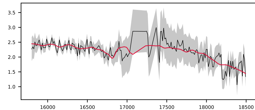
-621534765478525288, 3.4' S/N 18, LSF 26 Å, STAR, v = +600 km/s, \Delta\chi^2=\text{inf} , \chi^2_r=0.7
