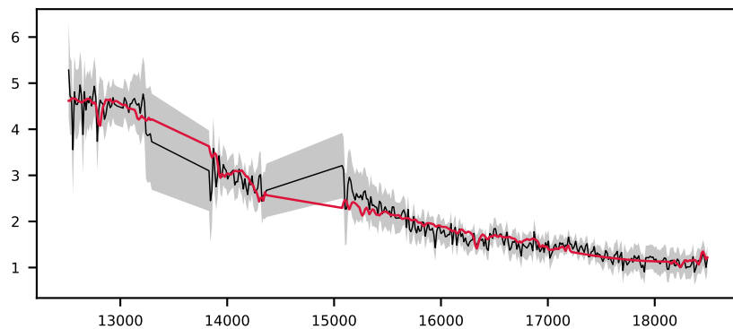
-619408499478806647, 6.5' S/N 18, LSF 11 Å, STAR, v = +0 km/s, \Delta\chi^2=\text{inf} , \chi^2_r=1.0
