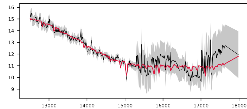
-620774866478715362, 1.8' S/N 77, LSF 30 Å, GALAXY, z = 1.001 , \Delta\chi^2=41 , \chi^2_r=4.9
