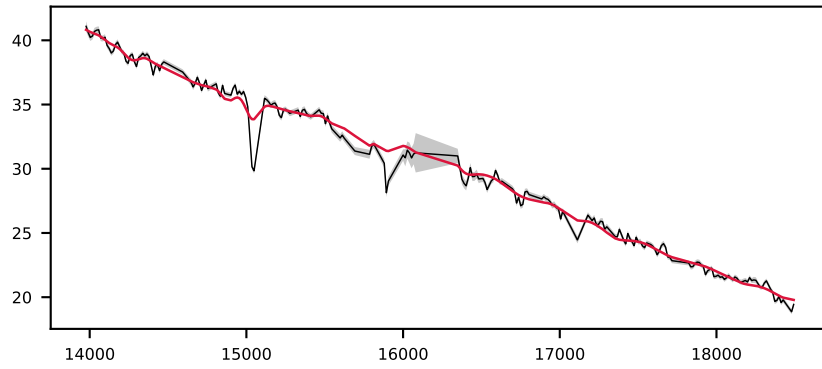
-620936482478743871, 1.4' S/N 151, LSF 13 Å, STAR, v = -450 km/s, \Delta\chi^2=\text{inf} , \chi^2_r=5.5
