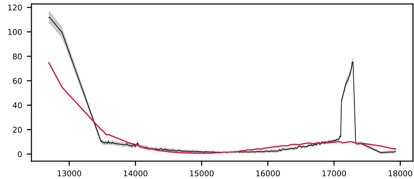
-618988267479412522, 8.5' S/N 28, LSF 35 Å, GALAXY, z = 0.133 , \Delta\chi^2=6 , \chi^2_r=0.6
