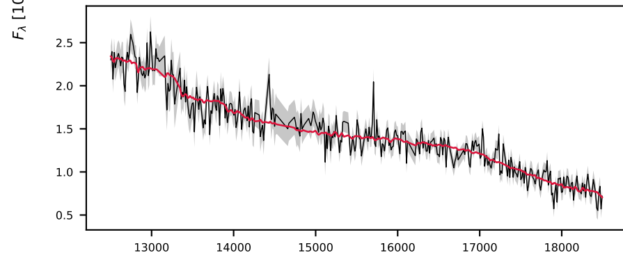
-620954485479420402, 2.7' S/N 14, LSF 14 Å, GALAXY, v = +0 km/s, \Delta\chi^2=0 , \chi^2_{\text{r}}=4.6
