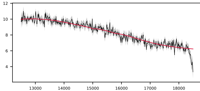
-621598390478403614, 4.2' S/N 30, LSF 58 Å, STAR, v = -600 km/s, \Delta\chi^2=\text{inf} , \chi^2_r=1.0
