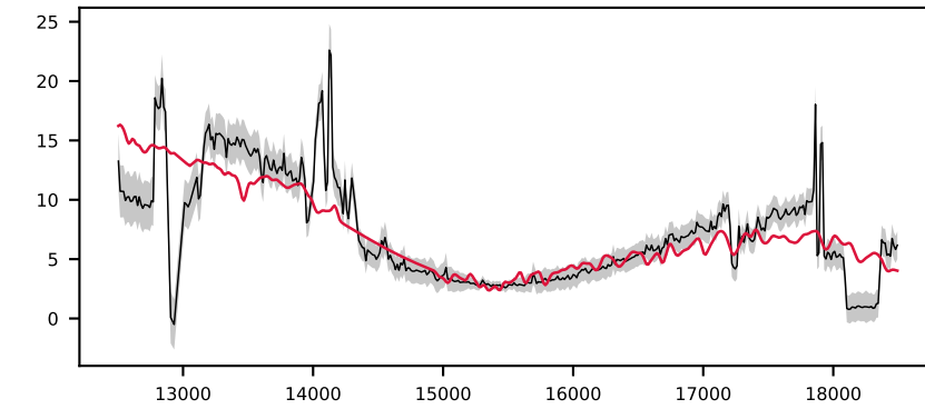
-620955862478659047, 1.9' S/N 50, LSF 16 Å, STAR, v = +600 km/s, \Delta\chi^2=\text{inf} , \chi^2_r=2.9
