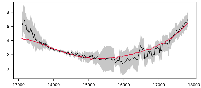
-623017038478369755, 8.9' S/N 20, LSF 12 Å, STAR, v = +0 km/s, \Delta\chi^2=\text{inf} , \chi^2_r=1.4
