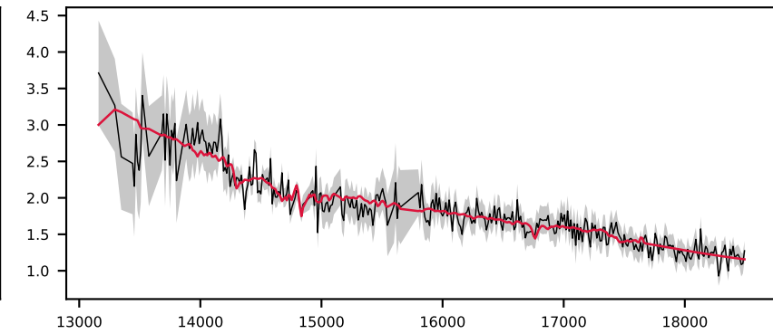
-621487728478644403, 2.8' S/N 17, LSF 13 Å, GALAXY, z = 0.103 , \Delta\chi^2=1 , \chi^2_r=0.3
