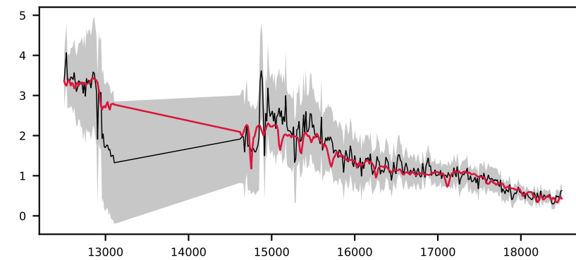
-621495416479238027, 2.5' S/N 14, LSF 11 Å, STAR, v = +150 km/s, \Delta\chi^2=\text{inf} , \chi^2_{\text{r}}=0.1
