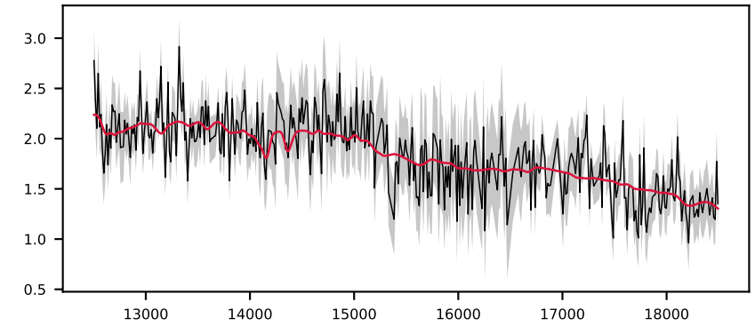
-620451183479247419, 2.8' S/N 13, LSF 12 Å, GALAXY, z = 0.185 , \Delta\chi^2=0 , \chi^2_r=0.1
