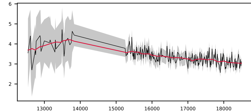
-623225026478671243, 9.1' S/N 13, LSF 33 Å, GALAXY, z = 0.335 , \Delta\chi^2=1 , \chi^2_r=0.6
