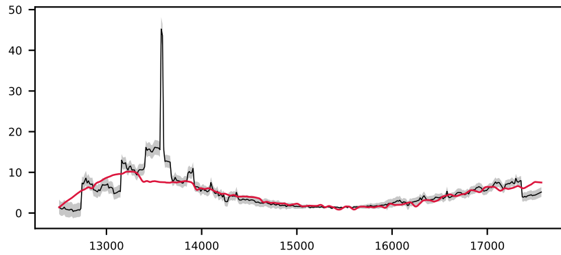
-620310020478222035, 5.3' S/N 31, LSF 13 Å, GALAXY, v = +0 km/s, \Delta\chi^2=0 , \chi^2_r=1.5
