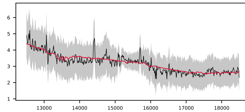
-619364414478834298, 6.6' S/N 30, LSF 25 Å, GALAXY, z = 0.243 , \Delta\chi^2=6 , \chi^2_r=0.6
