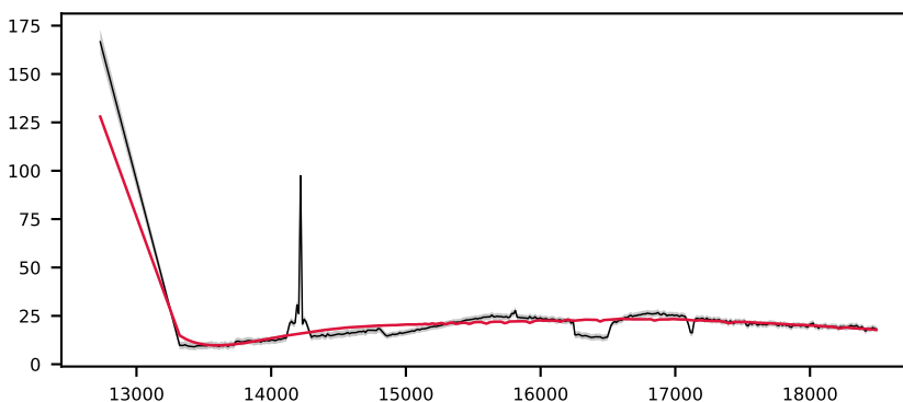
-621061637478732202, 1.4' S/N 125, LSF 14 Å, STAR, v = +600 km/s, \Delta\chi^2=\text{inf} , \chi^2_r=6.3
