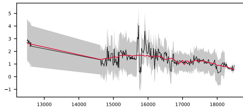
-620416465478910462, 2.4' S/N 12, LSF 18 Å, GALAXY, z = 0.530 , \Delta\chi^2=2 , \chi^2_r=0.2
