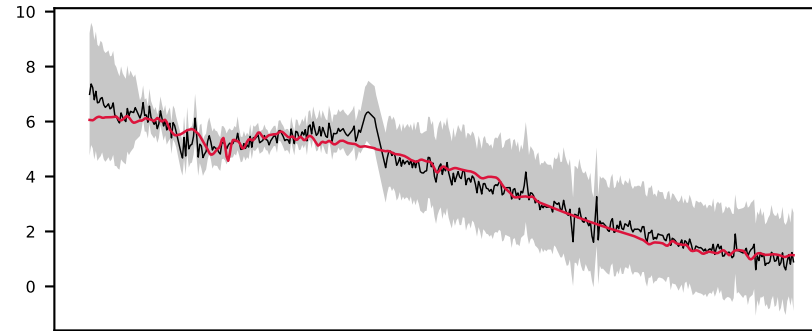
-620499921479146555, 2.3' S/N 25, LSF 18 Å, GALAXY, z = 0.206 , \Delta\chi^2=4 , \chi^2_r=0.1
