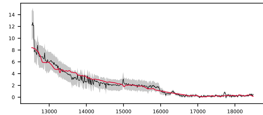
-620577433478660001, 2.5' S/N 20, LSF 20 Å, GALAXY, z = 0.115 , \Delta\chi^2=1 , \chi^2_r=0.3
