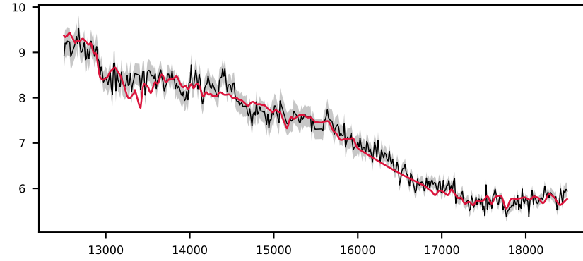
-620674519478799923, 1.7' S/N 61, LSF 18 Å, GALAXY, v = +0 km/s, \Delta\chi^2=0 , \chi^2_r=42.8 X unfittable
