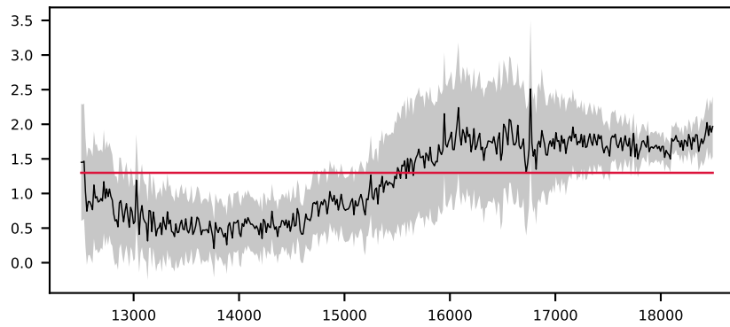
-621133280479452733, 2.9' S/N 16, LSF 12 Å, GALAXY, v = +0 \text{ km/s} , \Delta\chi^2=0 , \chi^2_r=1.6
