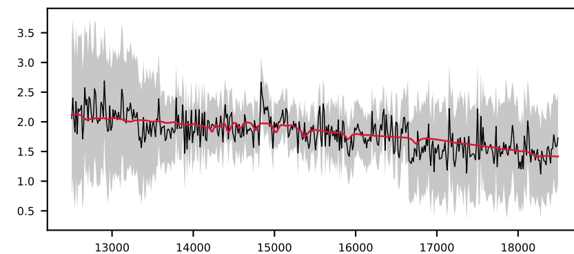
-620525143479318830, 2.8' S/N 13, LSF 23 Å, GALAXY, z = 0.066 , \Delta\chi^2=1 , \chi^2_r=0.2
