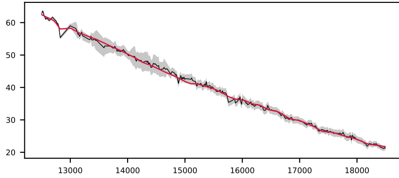
-619773769478221774, 6.7' S/N 157, LSF 41 Å, STAR, v = +0 km/s, \Delta\chi^2=\text{inf} , \chi^2_r=9.0
