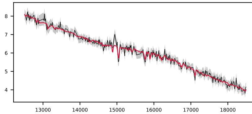
-621217271479233254, 1.8' S/N 54, LSF 15 Å, GALAXY, z = 0.053 , \Delta\chi^2=10 , \chi^2_r=0.2
