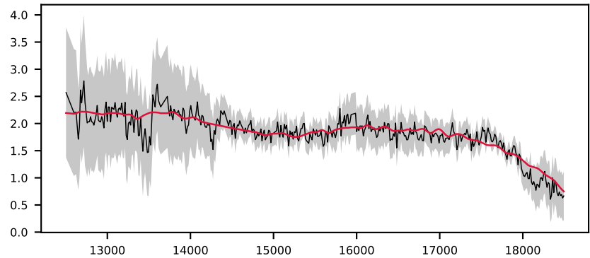
-619843510478118932, 6.9' S/N 15, LSF 47 Å, STAR, v = -600 km/s, \Delta\chi^2=\text{inf} , \chi^2_{\text{r}}=0.2
