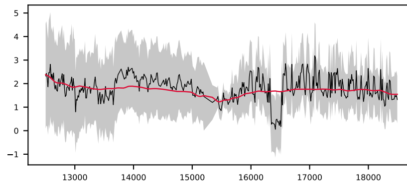
-620884781479489061, 3.2' S/N 14, LSF 19 Å, GALAXY, v = +0 km/s, \Delta\chi^2=0 , \chi^2_{\text{r}}=0.9
