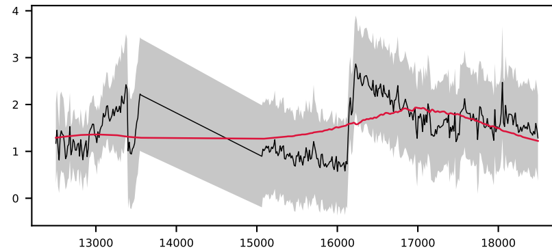
-619726937478315961, 6.5' S/N 13, LSF 19 Å, GALAXY, z = 0.689 , \Delta\chi^2=8 , \chi^2_r=0.8
