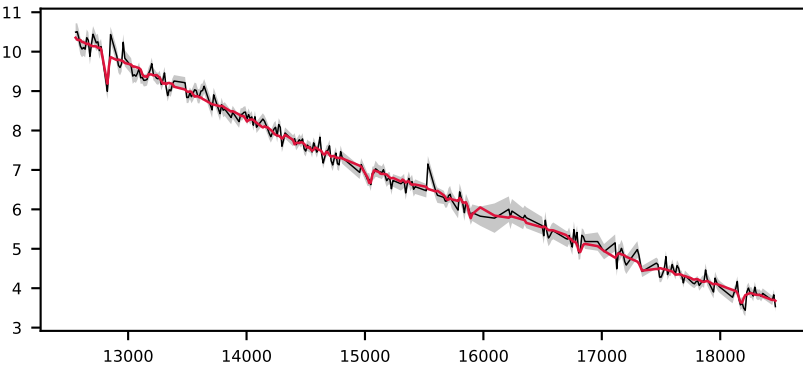
-623149680478206119, 9.8' S/N 50, LSF 12 Å, STAR, v = +0 km/s, \Delta\chi^2=\text{inf} , \chi^2_r=0.7
