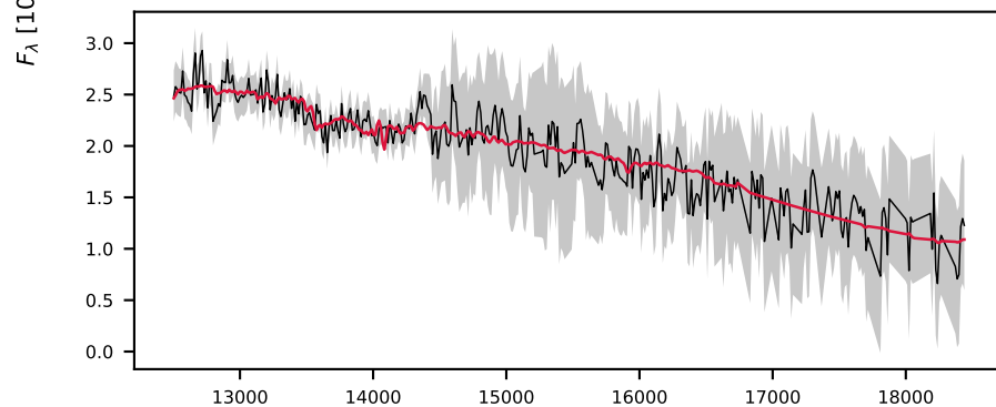
-623379823478654393, 9.7' S/N 18, LSF 17 Å, GALAXY, z = 1.001 , \Delta\chi^2=1 , \chi^2_r=0.1
