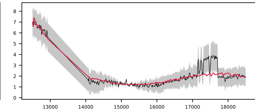
-621094315479404759, 2.6' S/N 17, LSF 12 Å, GALAXY, v = +0 km/s, \Delta\chi^2=0 , \chi^2_r=4.5
