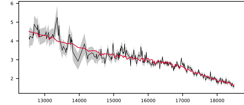
-620987817480235739, 7.6' S/N 26, LSF 12 Å, GALAXY, z = 0.273 , \Delta\chi^2=0 , \chi^2_r=0.1
