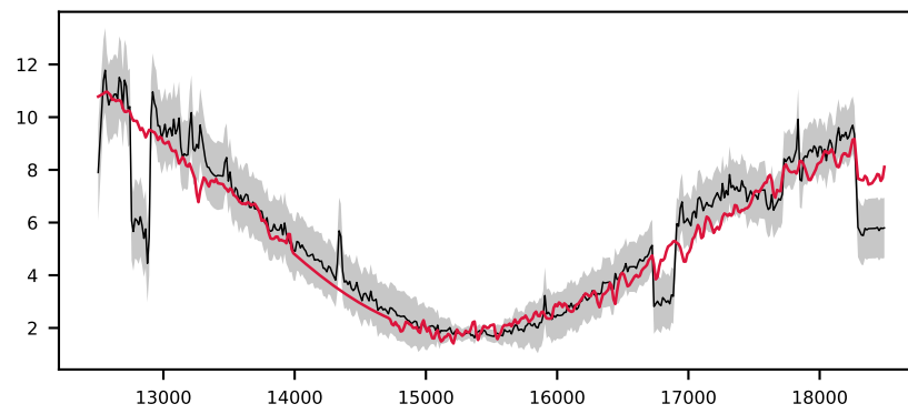
-623075421478341613, 9.1' S/N 45, LSF 12 Å, STAR, v = +0 km/s, \Delta\chi^2=\text{inf} , \chi^2_r=1.9
