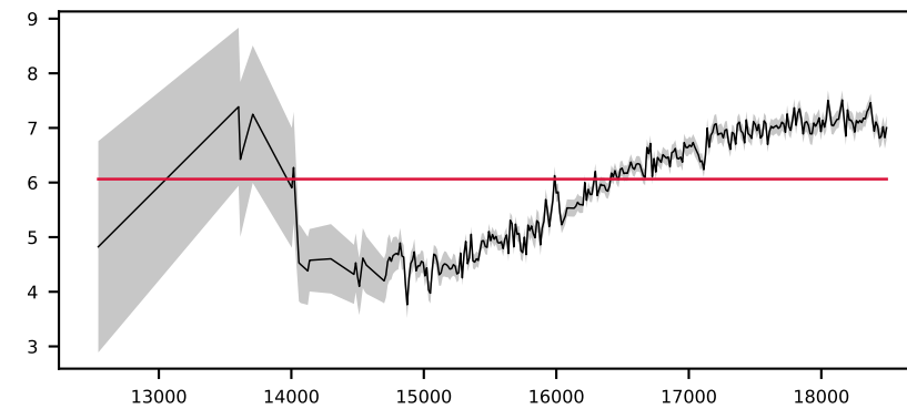
-620512763478787700, 2.3' S/N 42, LSF 12 Å, GALAXY, v = +0 km/s, \Delta\chi^2=0 , \chi^2_r=34.4 ✗ unfittable
