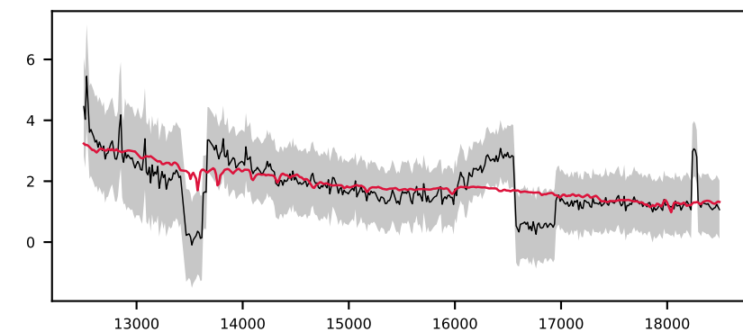
-621482089479311002, 2.8' S/N 16, LSF 9 Å, GALAXY, z = 0.589 , \Delta\chi^2=1 , \chi^2_r=0.3
