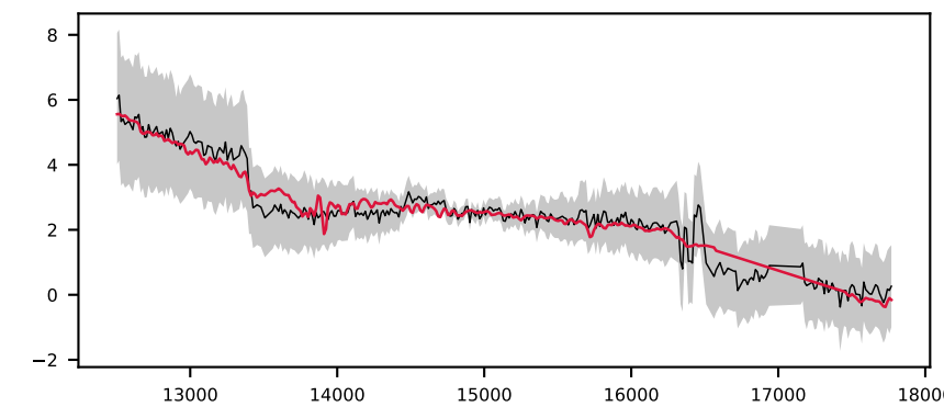
-620508753479238251, 2.6' S/N 21, LSF 13 Å, GALAXY, z = 0.226 , \Delta\chi^2=4 , \chi^2_{\text{r}}=0.1
