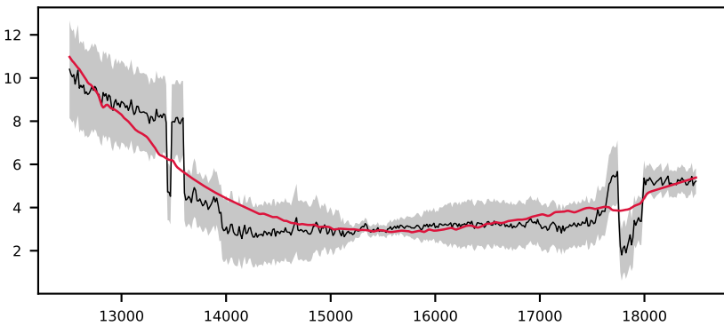
-621454655478706346, 2.4' S/N 31, LSF 20 Å, GALAXY, v = +0 km/s, \Delta\chi^2=11 , \chi^2_r=0.3
