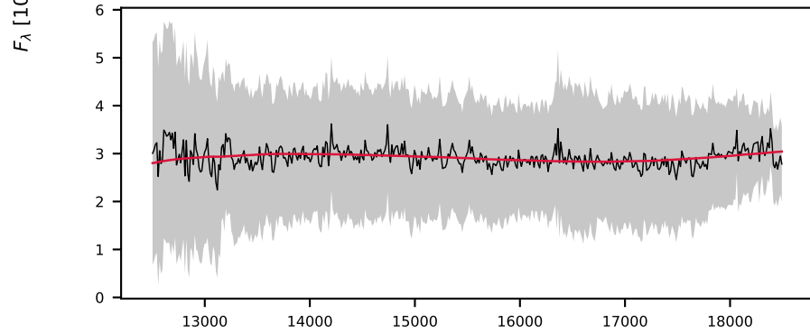
-622201980478806652, 4.9' S/N 19, LSF 15 Å, STAR, v = +300 km/s, \Delta\chi^2=\text{inf} , \chi^2_r=0.6
