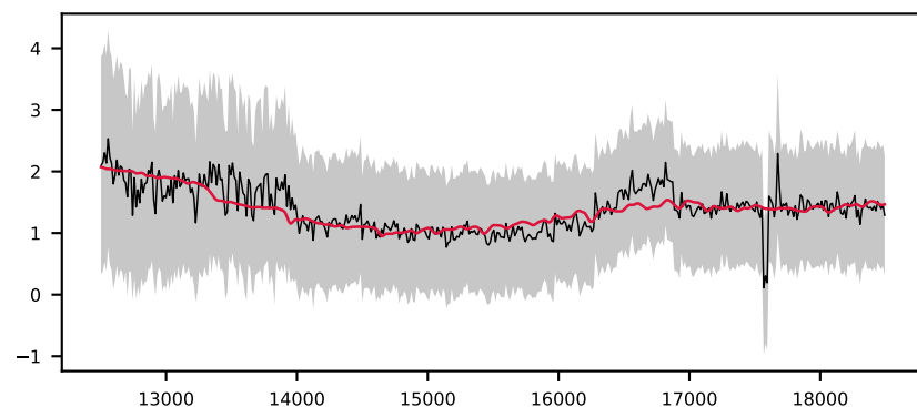
-622026941479284629, 4.5' S/N 12, LSF 16 Å, STAR, v = +600 km/s, \Delta\chi^2=\text{inf} , \chi^2_r=0.0
