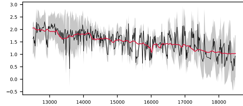
-620930042479507839, 3.2' S/N 12, LSF 16 Å, GALAXY, v = +0 km/s, \Delta\chi^2=0 , \chi^2_r=0.6
