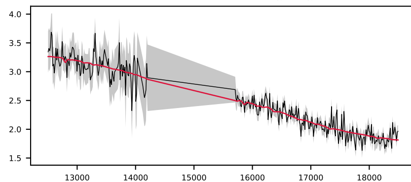
-622903155479285879, 7.9' S/N 21, LSF 12 Å, GALAXY, z = 0.841 , \Delta\chi^2=1 , \chi^2_r=0.2
