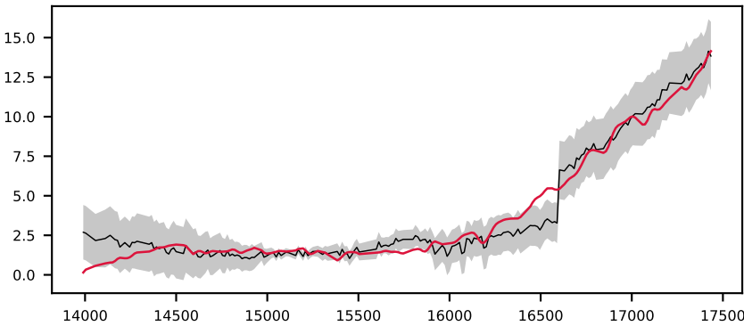
-619915769480038668, 7.8' S/N 15, LSF 37 Å, GALAXY, z = 0.042 , \Delta\chi^2=4 , \chi^2_{\text{r}}=0.2
