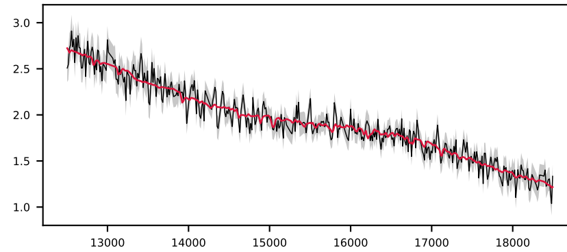
-619279156479357408, 7.3' S/N 20, LSF 16 Å, GALAXY, z = 0.296 , \Delta\chi^2=4 , \chi^2_r=0.2
