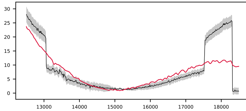
-620672091478777651, 1.8' S/N 34, LSF 16 Å, STAR, v = -600 km/s, \Delta\chi^2=\text{inf} , \chi^2_r=1.2
