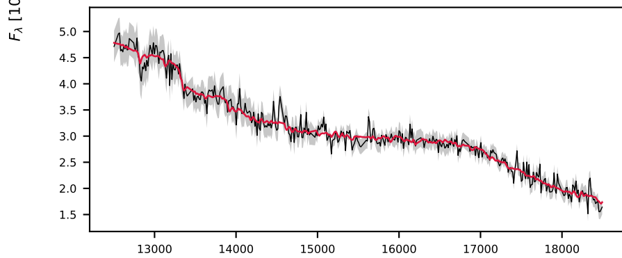
-621598390478403614, 4.2' S/N 30, LSF 58 Å, STAR, v = -600 km/s, \Delta\chi^2=\text{inf} , \chi^2_r=1.0
