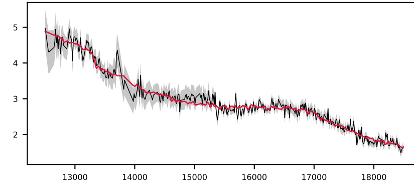
-620657653478318874, 4.1' S/N 26, LSF 24 Å, GALAXY, z = 0.963 , \Delta\chi^2=11 , \chi^2_r=1.1
