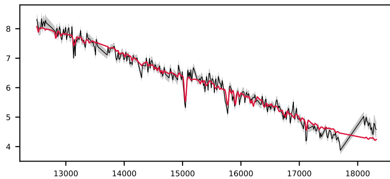
-622851958479341022, 7.8' S/N 40, LSF 12 Å, STAR, v = +0 km/s, \Delta\chi^2=\text{inf} , \chi^2_r=0.5
