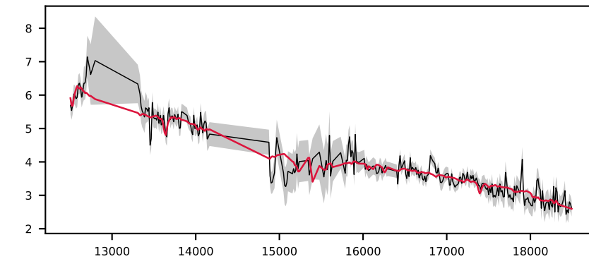
-623406451479254632, 9.8' S/N 27, LSF 13 Å, STAR, v = +0 km/s, \Delta\chi^2=\text{inf} , \chi^2_r=1.1
