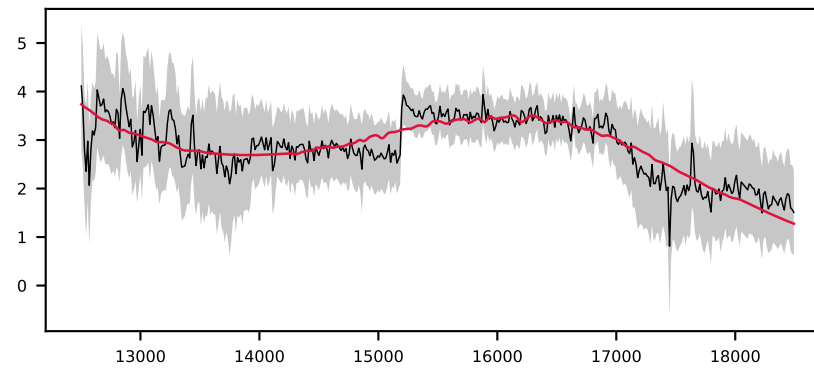
-621052334479447391, 2.9' S/N 20, LSF 13 Å, GALAXY, v = +0 km/s, \Delta\chi^2=0 , \chi^2_r=1.7
