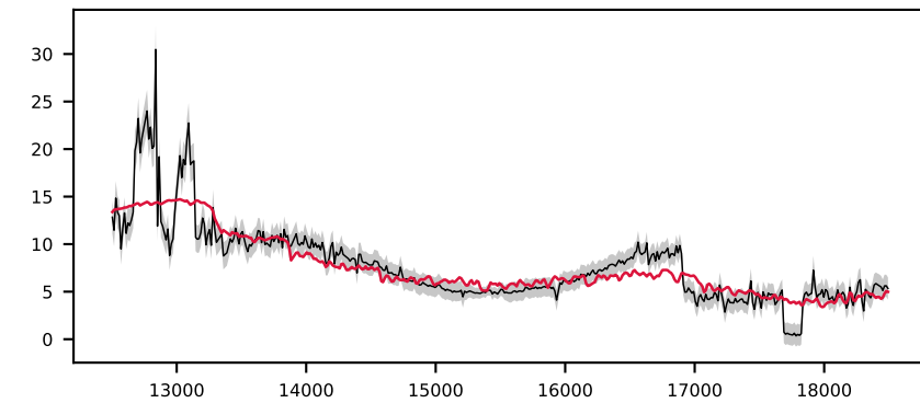
-620781865478730478, 1.7' S/N 58, LSF 21 Å, GALAXY, v = +0 km/s, \Delta\chi^2=0 , \chi^2_r=41.1 ✗ unfittable
