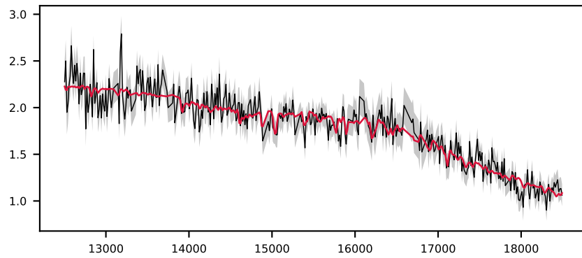
-620920159478324595, 3.9' S/N 17, LSF 12 Å, GALAXY, z = 0.260 , \Delta\chi^2=4 , \chi^2_r=0.3
