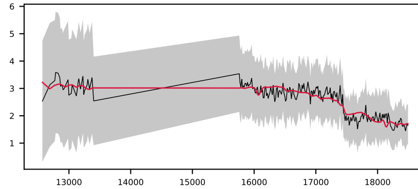
-622877489478245514, 8.7' S/N 17, LSF 13 Å, GALAXY, z = 0.905 , \Delta\chi^2=1 , \chi^2_r=0.6
