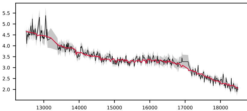
-623187011478236782, 9.8' S/N 33, LSF 13 Å, STAR, v = +0 km/s, \Delta\chi^2=\text{inf} , \chi^2_r=1.0
