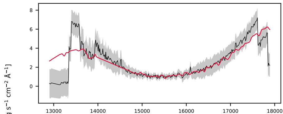
-623454186479039775, 9.9' S/N 21, LSF 26 Å, GALAXY, z = 0.073 , \Delta\chi^2=4 , \chi^2_r=0.2
