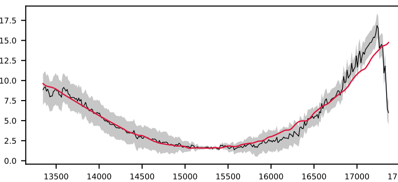
-620959431478643338, 2.0' S/N 30, LSF 35 Å, GALAXY, v = +300 km/s, \Delta\chi^2=18 , \chi^2_r=0.6
