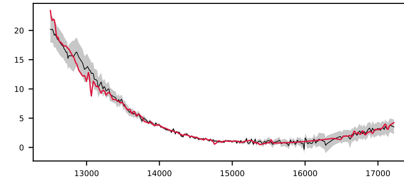
-618760603478861522, 9.1' S/N 13, LSF 12 Å, STAR, v = -150 km/s, \Delta\chi^2=\text{inf} , \chi^2_r=0.5
