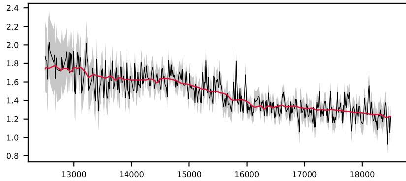
-621026009479629169, 4.0' S/N 13, LSF 13 Å, GALAXY, z = 0.807 , \Delta\chi^2=1 , \chi^2_r=0.1
