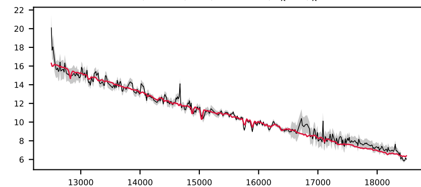
-620096817480256406, 8.5' S/N 70, LSF 13 Å, STAR, v = +0 km/s, \Delta\chi^2=\text{inf} , \chi^2_r=1.0
