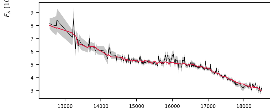
-620952016478658285, 1.9' S/N 42, LSF 14 Å, STAR, v = +600 km/s, \Delta\chi^2=\text{inf} , \chi^2_r=3.5
