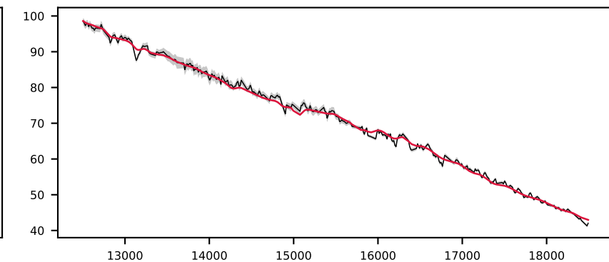
-620600383479092111, 1.8' S/N 196, LSF 15 Å, STAR, v = +600 km/s, \Delta\chi^2=\text{inf} , \chi^2_r=0.5
