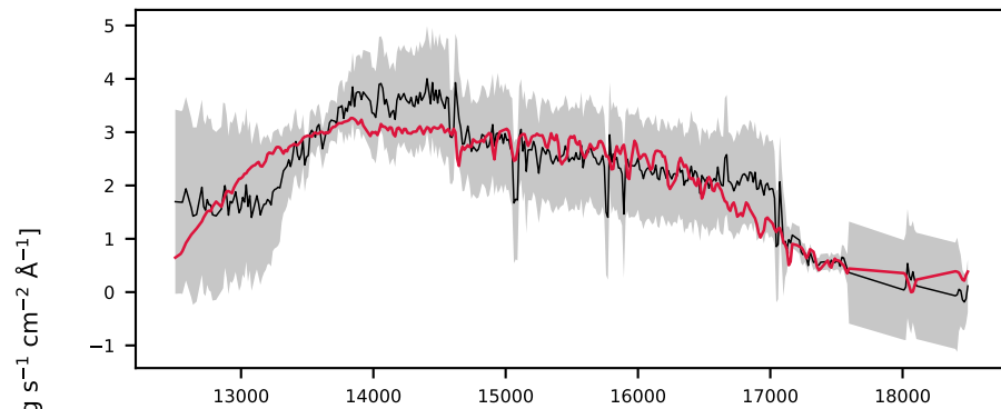
-620561718478715002, 2.3' S/N 20, LSF 20 Å, STAR, v = +150 km/s, \Delta\chi^2=\text{inf} , \chi^2_r=2.0
