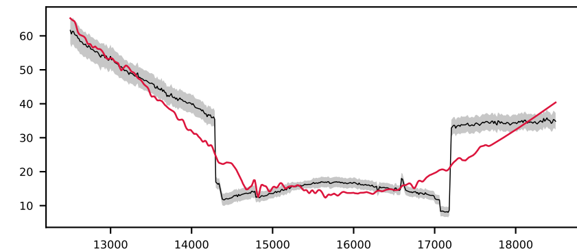
-619312452478546960, 7.3' S/N 134, LSF 26 Å, STAR, v = +150 km/s, \Delta\chi^2=\text{inf} , \chi^2_r=1.7
