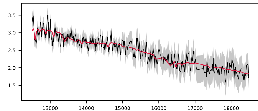
-619657546479169825, 5.6' S/N 22, LSF 13 Å, GALAXY, z = 0.314 , \Delta\chi^2=2 , \chi^2_r=0.2
