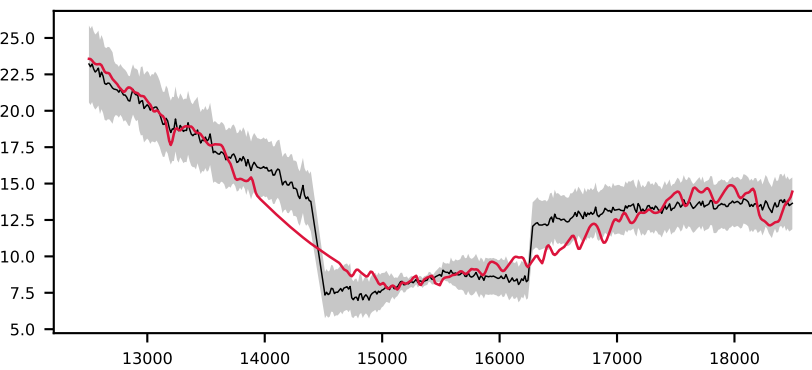
-620948243479268014, 1.8' S/N 75, LSF 18 Å, GALAXY, z = 0.053 , \Delta\chi^2=53 , \chi^2_r=0.8
