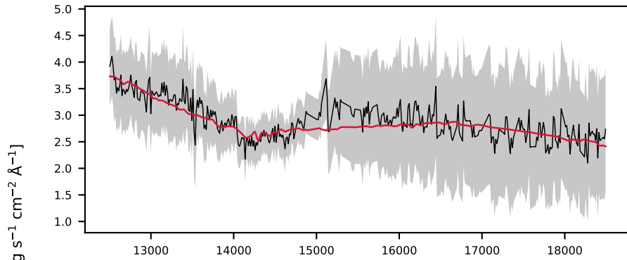
-618727676478541333, 9.5' S/N 22, LSF 17 Å, GALAXY, z = 0.325 , \Delta\chi^2=3 , \chi^2_{\text{r}}=0.2
