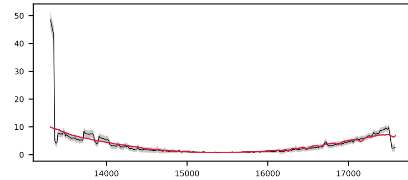
-619185778479281456, 7.6' S/N 25, LSF 22 Å, GALAXY, z = 0.330 , \Delta\chi^2=6 , \chi^2_r=0.8
