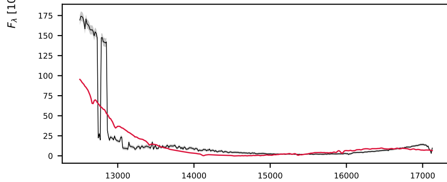
-620702263478765420, 1.7' S/N 54, LSF 21 Å, STAR, v = +600 km/s, \Delta\chi^2=\text{inf} , \chi^2_r=1.0
