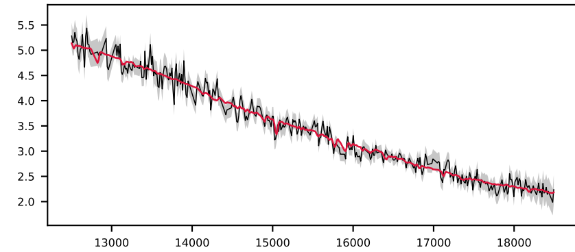
-619553023480043381, 8.7' S/N 34, LSF 11 Å, STAR, v = +150 km/s, \Delta\chi^2=\text{inf} , \chi^2_r=0.8
