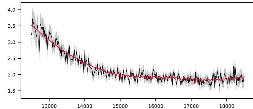
-620149441477545546, 9.2' S/N 22, LSF 21 Å, GALAXY, z = 0.452 , \Delta\chi^2=11 , \chi^2_r=0.4
