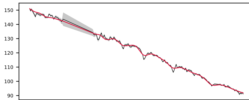
-620333176479824074, 5.8' S/N 277, LSF 50 Å, STAR, v = -150 km/s, \Delta\chi^2=\text{inf} , \chi^2_r=4.0
