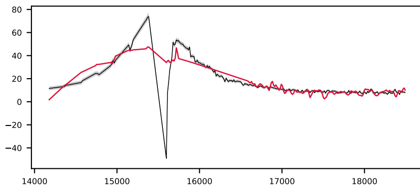
-621005200479207510, 1.4' S/N 78, LSF 18 Å, STAR, v = -600 km/s, \Delta\chi^2=\text{inf} , \chi^2_r=20.0 ✗ unfittable
