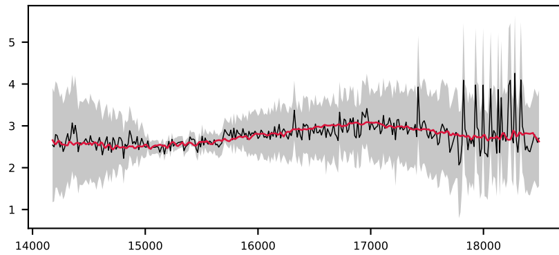
-619274277479497483, 7.6' S/N 25, LSF 13 Å, GALAXY, z = 0.314 , \Delta\chi^2=2 , \chi^2_r=0.1
