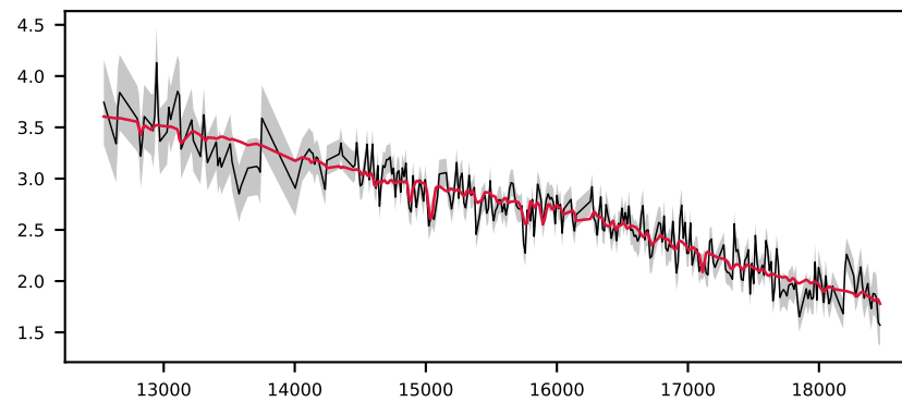
-622195259478769735, 4.9' S/N 20, LSF 20 Å, GALAXY, v = +0 km/s, \Delta\chi^2=1 , \chi^2_r=0.2
