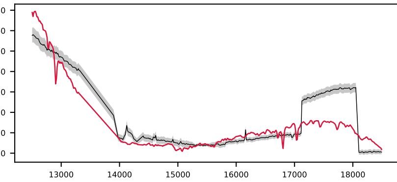
-621179152478672221, 1.9' S/N 60, LSF 9 Å, GALAXY, z = 0.967 , \Delta\chi^2=71 , \chi^2_r=15.0
