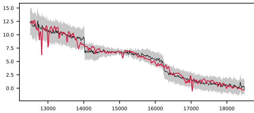
-620864431479311085, 2.1' S/N 45, LSF 18 Å, GALAXY, z = 0.027 , \Delta\chi^2=33 , \chi^2_r=0.6
