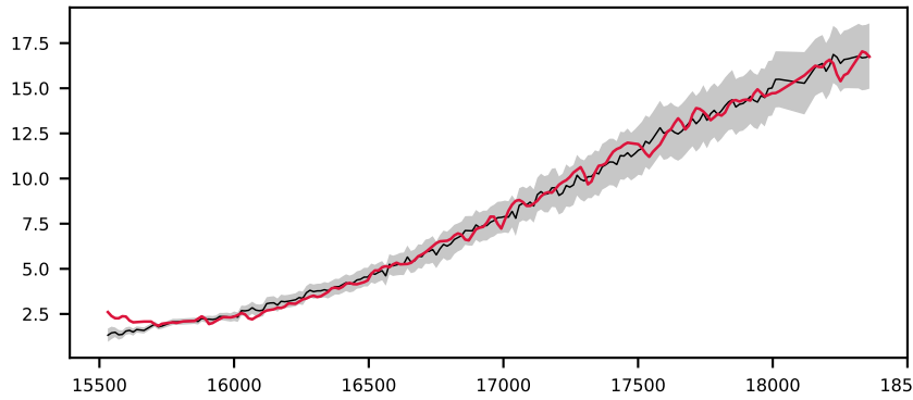
-621629259480426258, 9.1' S/N 50, LSF 12 Å, STAR, v = +0 km/s, \Delta\chi^2=\text{inf} , \chi^2_r=1.2
