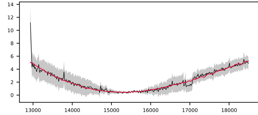
-620091529478376794, 5.1' S/N 13, LSF 12 Å, STAR, v = -300 km/s, \Delta\chi^2=\text{inf} , \chi^2_r=0.9
