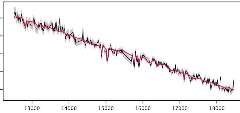
-621368604480501686, 9.3' S/N 38, LSF 12 Å, STAR, v = +150 km/s, \Delta\chi^2=\text{inf} , \chi^2_{\text{r}}=1.0
