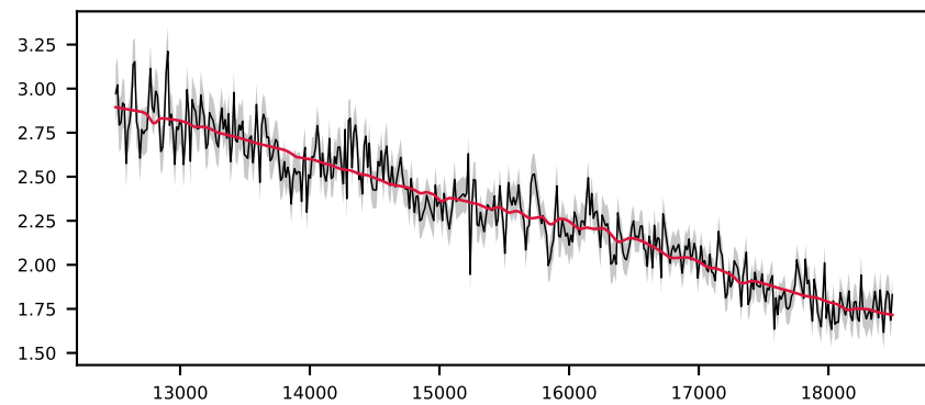
-622640430479504555, 7.3' S/N 23, LSF 28 Å, STAR, v = -600 km/s, \Delta\chi^2=\text{inf} , \chi^2_r=1.3
