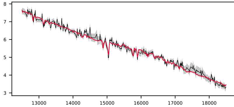
-621384170478388770, 3.8' S/N 50, LSF 13 Å, STAR, v = +0 km/s, \Delta\chi^2=\text{inf} , \chi^2_r=1.0
