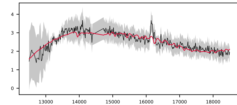
-623387224478699500, 9.7' S/N 18, LSF 21 Å, STAR, v = +600 km/s, \Delta\chi^2=\text{inf} , \chi^2_r=0.2
