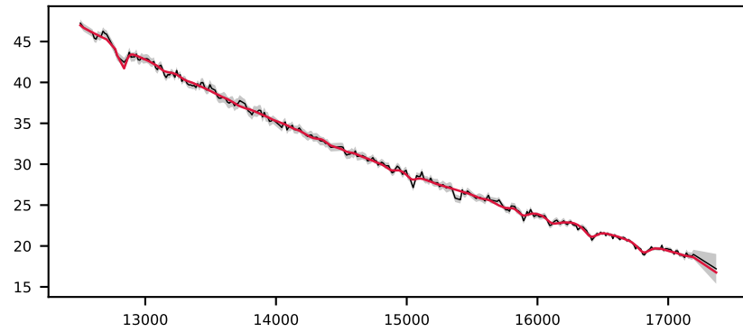
-620600449479164349, 2.0' S/N 111, LSF 25 Å, STAR, v = +150 km/s, \Delta\chi^2=\text{inf} , \chi^2_r=1.7
