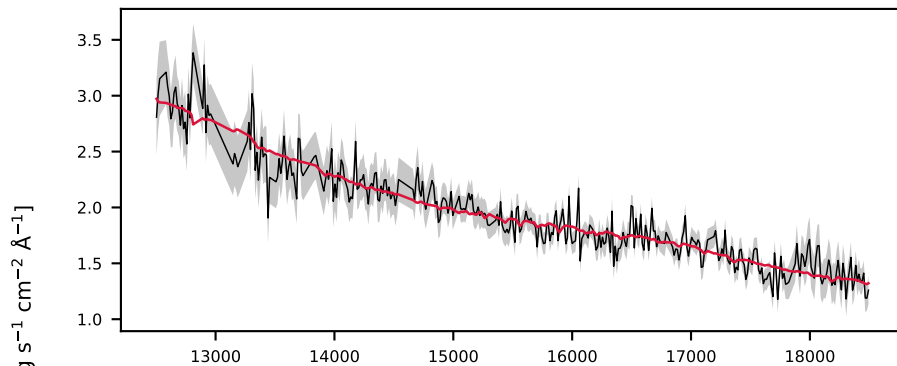
-619047756478254868, 9.0' S/N 18, LSF 13 Å, GALAXY, z = 0.241 , \Delta\chi^2=1 , \chi^2_r=0.3
