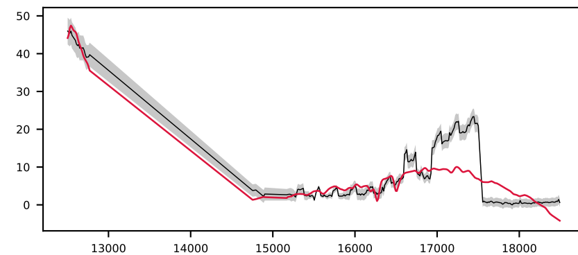
-619254687477821084, 9.9' S/N 21, LSF 19 Å, STAR, v = -600 km/s, \Delta\chi^2=\text{inf} , \chi^2_r=0.9
