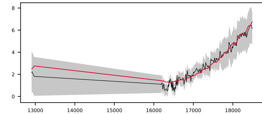
-620180038478795115, 3.5' S/N 20, LSF 24 Å, GALAXY, z = 0.357 , \Delta\chi^2=3 , \chi^2_r=0.7
