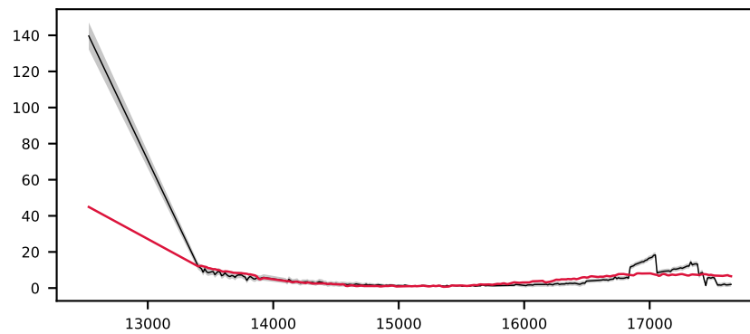
-620486456478879726, 2.2' S/N 24, LSF 21 Å, GALAXY, v = +0 km/s, \Delta\chi^2=0 , \chi^2_r=0.8
