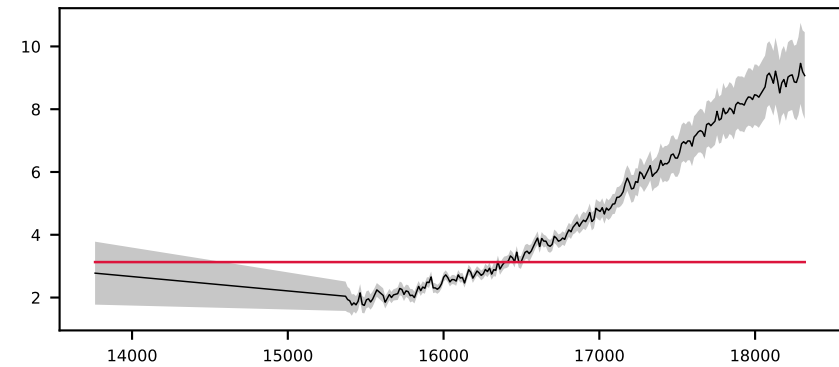
-620721242479412761, 2.9' S/N 28, LSF 22 Å, GALAXY, z = 0.767 , \Delta\chi^2=1 , \chi^2_r=0.2
