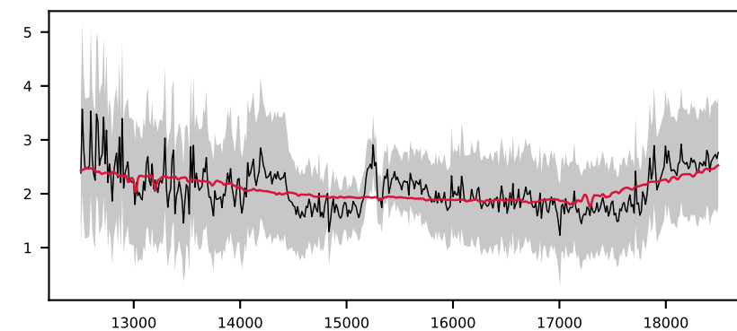
-620472826479254639, 2.7' S/N 21, LSF 13 Å, GALAXY, z = 0.524 , \Delta\chi^2=0 , \chi^2_r=0.1
