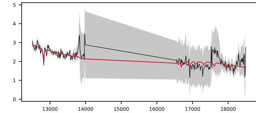
-618643337478894769, 9.5' S/N 19, LSF 34 Å, STAR, v = +600 km/s, \Delta\chi^2=\text{inf} , \chi^2_r=0.4
