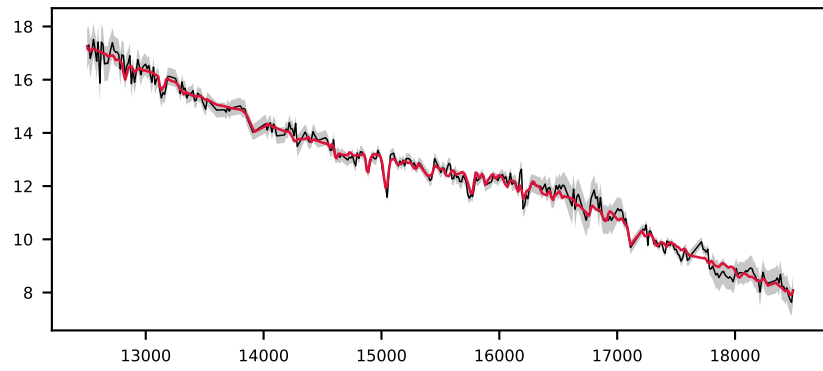
-622052430478594148, 4.8' S/N 91, LSF 16 Å, STAR, v = +0 km/s, \Delta\chi^2=\text{inf} , \chi^2_r=2.5
