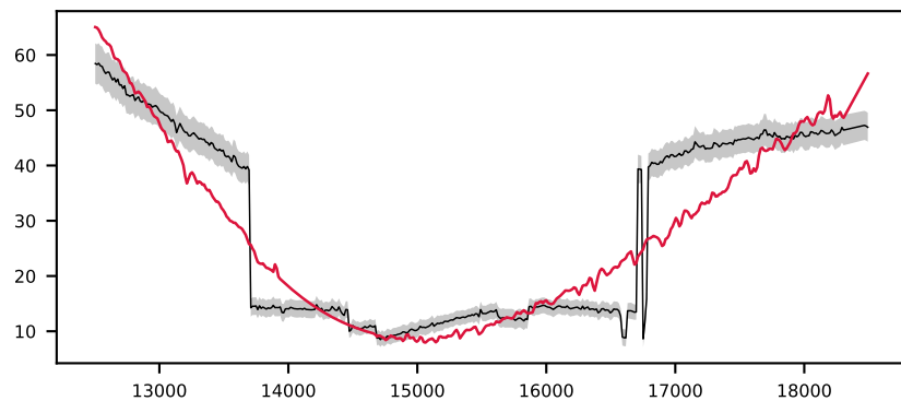
-619094773478718083, 7.8' S/N 139, LSF 34 Å, STAR, v = +0 km/s, \Delta\chi^2=\text{inf} , \chi^2_r=3.0
