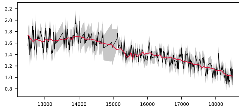
-619836598478207058, 6.6' S/N 13, LSF 17 Å, GALAXY, z = 0.372 , \Delta\chi^2=10 , \chi^2_r=0.7
