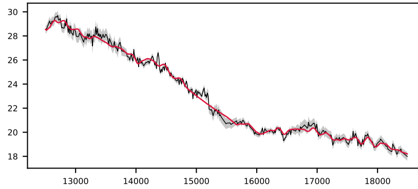
-620802079478719755, 1.7' S/N 119, LSF 22 Å, STAR, v = +600 km/s, \Delta\chi^2=\text{inf} , \chi^2_r=3.0
