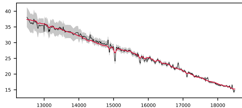
-623253409478283967, 9.9' S/N 134, LSF 19 Å, STAR, v = +0 km/s, \Delta\chi^2=\text{inf} , \chi^2_r=0.3
