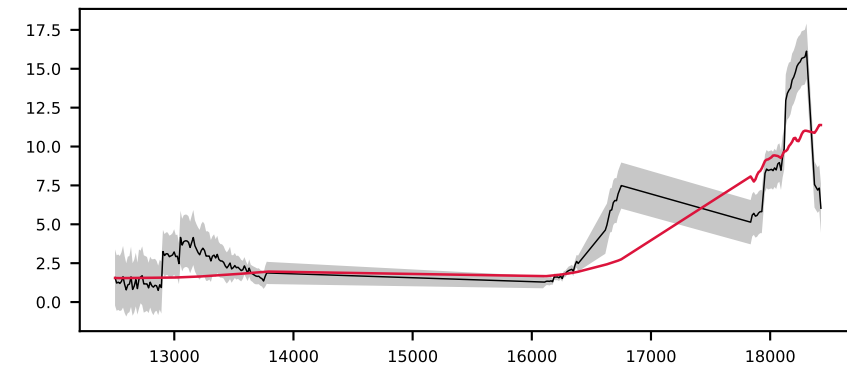
-620141096479765839, 5.9' S/N 16, LSF 25 Å, STAR, v = -600 km/s, \Delta\chi^2=\text{inf} , \chi^2_r=1.4
