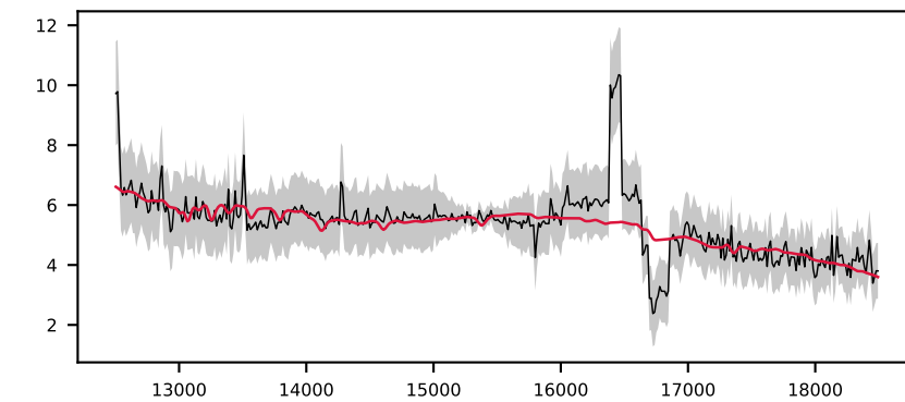
-621367244479134539, 1.8' S/N 49, LSF 17 Å, GALAXY, z = 0.530 , \Delta\chi^2=3 , \chi^2_r=0.4
