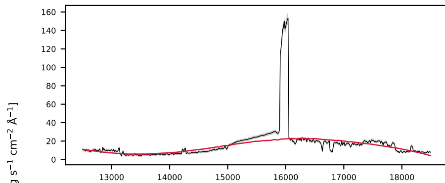
-621048223479225428, 1.5' S/N 76, LSF 20 Å, GALAXY, v = +0 km/s, \Delta\chi^2=0 , \chi^2_r=10.9
