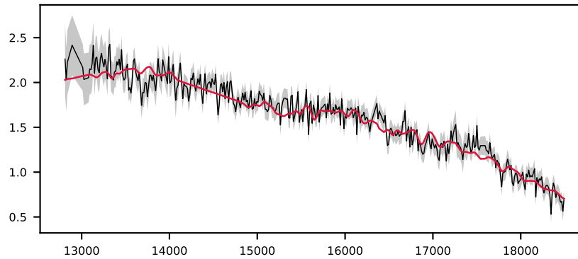
-619466239479155580, 6.3' S/N 15, LSF 11 Å, STAR, v = +150 km/s, \Delta\chi^2=\text{inf} , \chi^2_{\text{r}}=0.7
