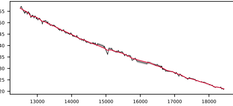
-620943141478143812, 5.0' S/N 155, LSF 34 Å, STAR, v = +0 km/s, \Delta\chi^2=\text{inf} , \chi^2_r=2.3
