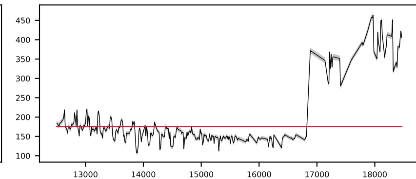
-618925920478984815, 8.4' S/N 245, LSF 56 Å, STAR, v = +0 km/s, \Delta\chi^2=\text{inf} , \chi^2_r=4.2
