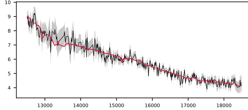
-619957794480072227, 7.8' S/N 26, LSF 13 Å, STAR, v = +0 km/s, \Delta\chi^2=\text{inf} , \chi^2_r=0.9
