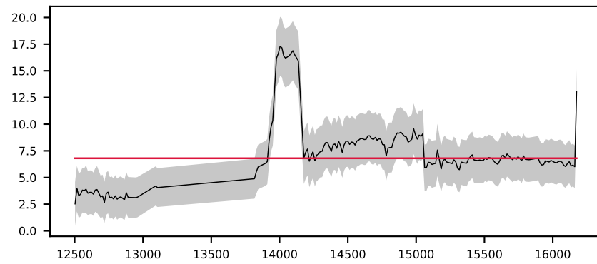
-622714088479517476, 7.6' S/N 30, LSF 12 Å, STAR, v = +0 km/s, \Delta\chi^2=\text{inf} , \chi^2_r=0.7
