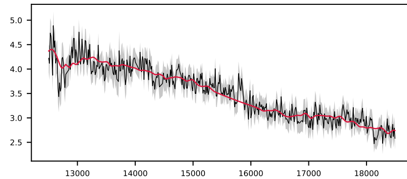
-620168394480000311, 7.0' S/N 28, LSF 12 Å, GALAXY, z = 0.357 , \Delta\chi^2=11 , \chi^2_r=0.8
