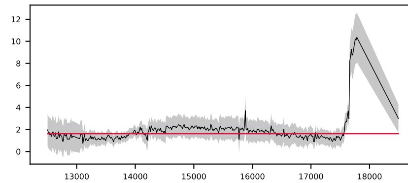
-620919617478411956, 3.4' S/N 16, LSF 10 Å, GALAXY, v = +0 km/s, \Delta\chi^2=0 , \chi^2_r=0.7
