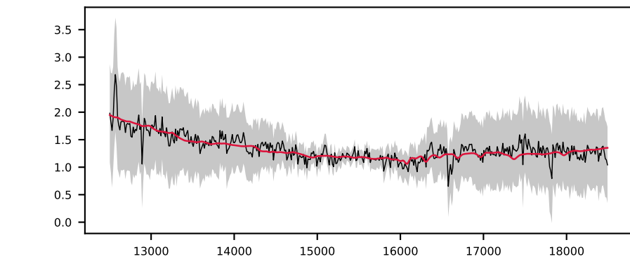
-621586259479105147, 2.5' S/N 15, LSF 17 Å, GALAXY, z = 0.882 , \Delta\chi^2=0 , \chi^2_r=0.1
