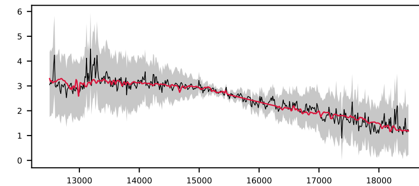
-620205501477925952, 7.0' S/N 23, LSF 12 Å, STAR, v = +150 km/s, \Delta\chi^2=\text{inf} , \chi^2_r=1.6
