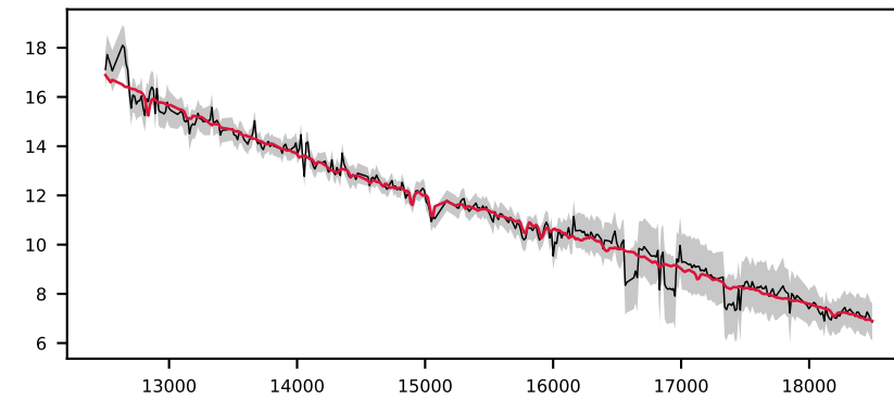
-620957009478310674, 4.0' S/N 83, LSF 12 Å, STAR, v = +0 km/s, \Delta\chi^2=\text{inf} , \chi^2_r=0.2
