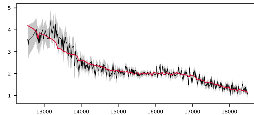
-619372075479072175, 6.6' S/N 22, LSF 37 Å, GALAXY, z = 0.333 , \Delta\chi^2=1 , \chi^2_{\text{r}}=0.3
