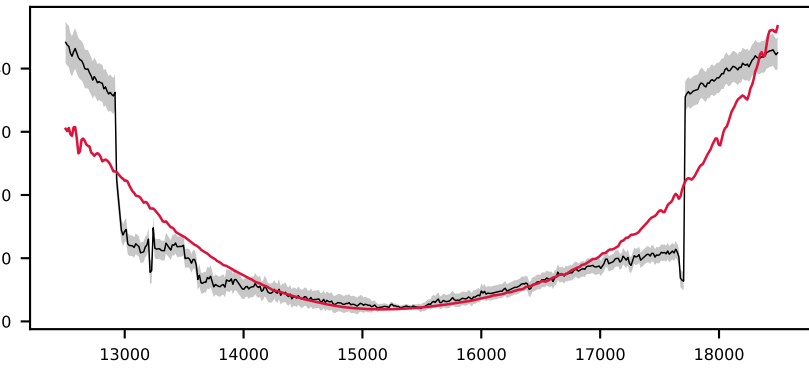
-622027475479693432, 6.0' S/N 61, LSF 18 Å, GALAXY, v = +0 km/s, \Delta\chi^2=0 , \chi^2_r=4.8
