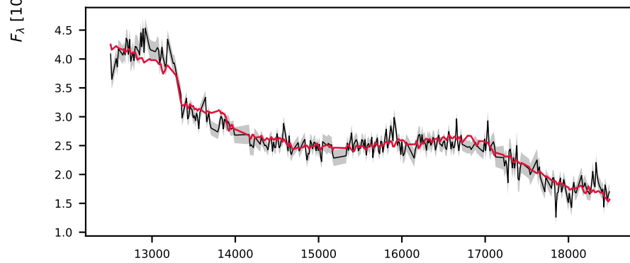
-623204666478810788, 8.9' S/N 24, LSF 32 Å, GALAXY, z = 0.048 , \Delta\chi^2=4 , \chi^2_r=1.1
