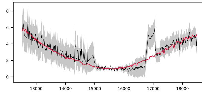
-621938801479377743, 4.5' S/N 22, LSF 13 Å, STAR, v = +300 km/s, \Delta\chi^2=\text{inf} , \chi^2_{\text{r}}=0.8
