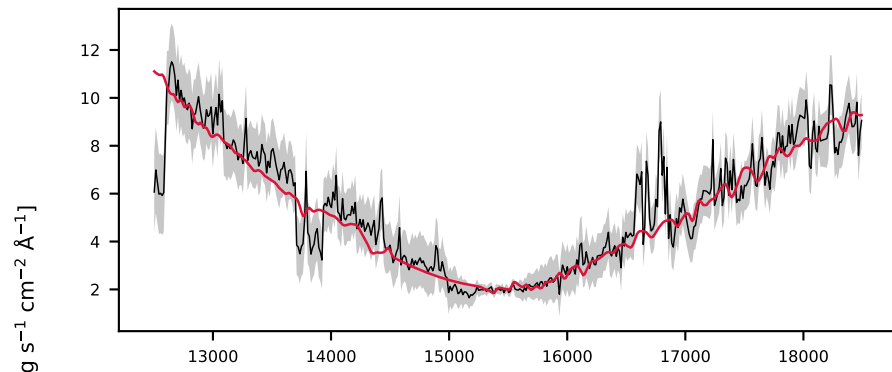
-620606161478747820, 2.1' S/N 46, LSF 15 Å, GALAXY, v = +0 km/s, \Delta\chi^2=0 , \chi^2_r=209.8 ✗ unfittable
