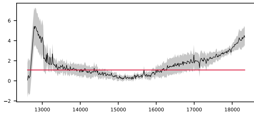
-620954485479420402, 2.7' S/N 14, LSF 14 Å, GALAXY, v = +0 km/s, \Delta\chi^2=0 , \chi^2_{\text{r}}=4.6
