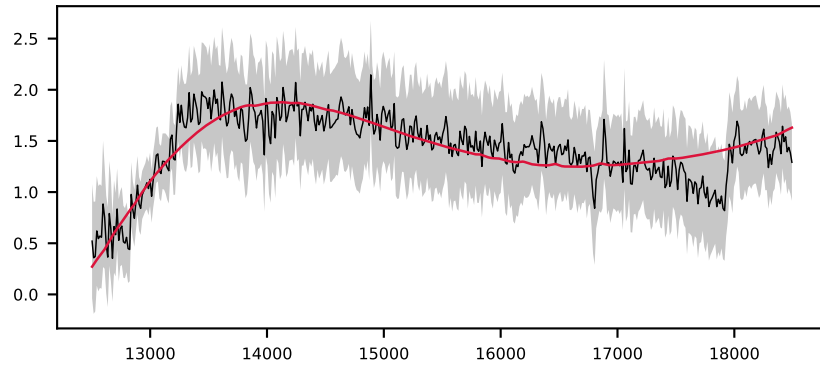
-620954736478214422, 4.5' S/N 13, LSF 17 Å, GALAXY, z = 0.102 , \Delta\chi^2=2 , \chi^2_r=0.5
