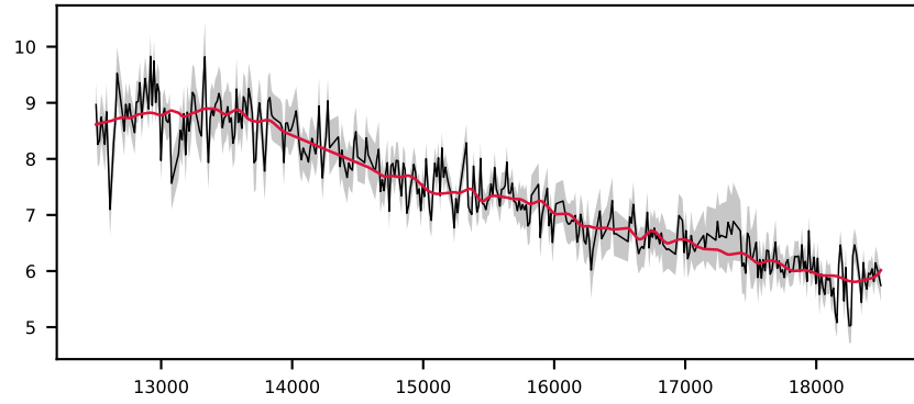
-619651484479164911, 5.6' S/N 26, LSF 16 Å, GALAXY, z = 0.383 , \Delta\chi^2=1 , \chi^2_r=0.2
