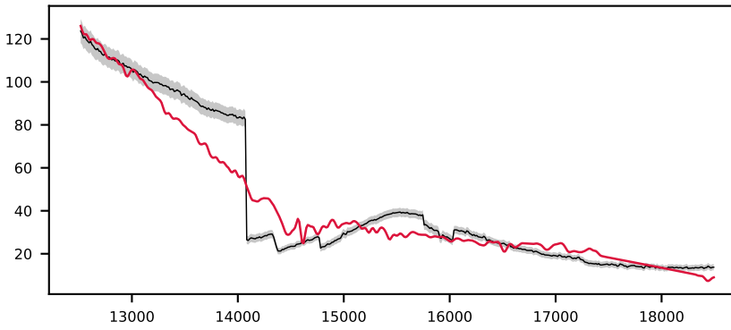
-620894087478693888, 1.7' S/N 149, LSF 14 Å, STAR, v = +600 km/s, \Delta\chi^2=\text{inf} , \chi^2_r=1.8
