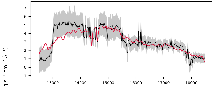
-621544140478794306, 2.4' S/N 23, LSF 20 Å, GALAXY, z = 0.417 , \Delta\chi^2=5 , \chi^2_r=0.2
