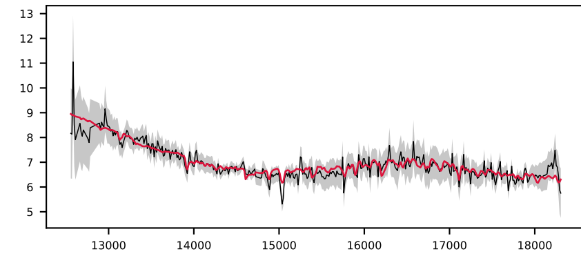
-619515577477930558, 8.6' S/N 44, LSF 12 Å, STAR, v = +0 km/s, \Delta\chi^2=\text{inf} , \chi^2_r=1.0
