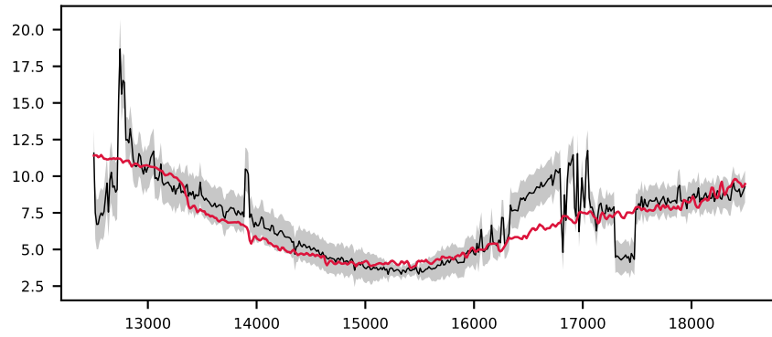
-622660498478729582, 6.8' S/N 61, LSF 12 Å, STAR, v = +0 km/s, \Delta\chi^2=\text{inf} , \chi^2_r=0.7
