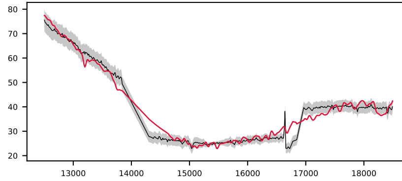
-621106124478760553, 1.3' S/N 157, LSF 19 Å, GALAXY, z = 0.288 , \Delta\chi^2=325 , \chi^2_r=15.3
