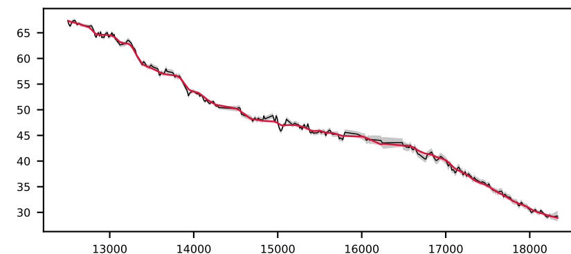
-619173573479720336, 8.6' S/N 202, LSF 50 Å, STAR, v = +150 km/s, \Delta\chi^2=\text{inf} , \chi^2_r=0.9
