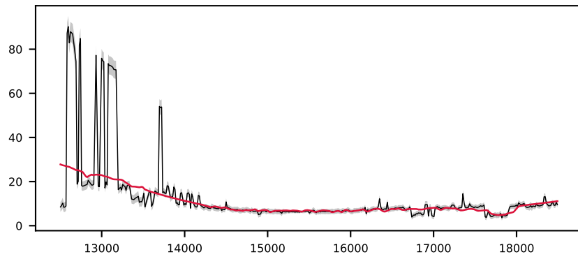
-619320205478547305, 7.2' S/N 62, LSF 14 Å, STAR, v = +150 km/s, \Delta\chi^2=\text{inf} , \chi^2_r=1.4
