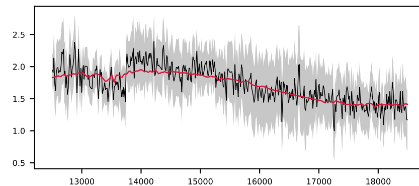
-620526528478624299, 2.8' S/N 13, LSF 17 Å, GALAXY, z = 0.983 , \Delta\chi^2=1 , \chi^2_r=0.2
