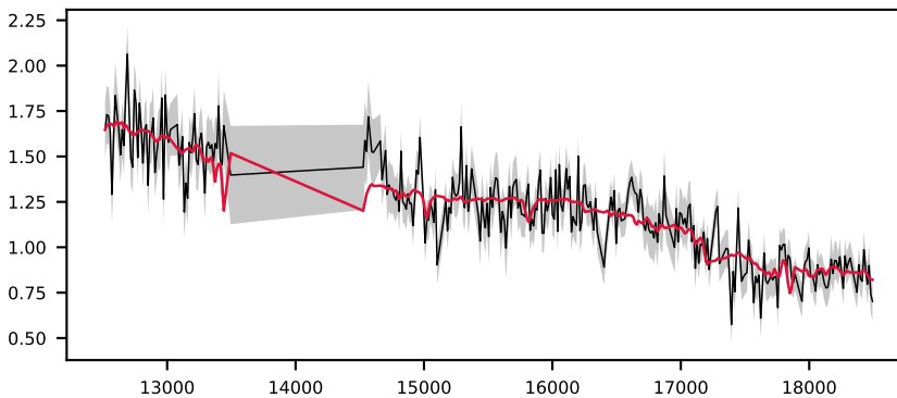
-619265292479313835, 7.3' S/N 12, LSF 20 Å, GALAXY, v = +0 km/s, \Delta\chi^2=0 , \chi^2_r=0.7
