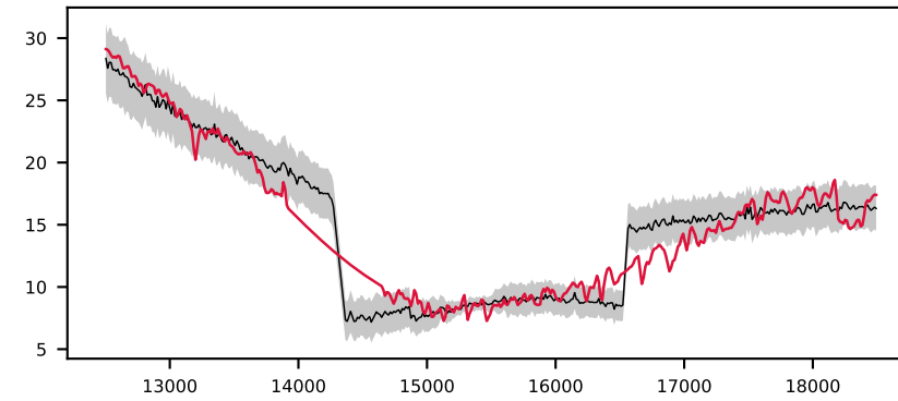
-621047771480124818, 6.9' S/N 86, LSF 13 Å, STAR, v = +300 km/s, \Delta\chi^2=\text{inf} , \chi^2_r=0.3
