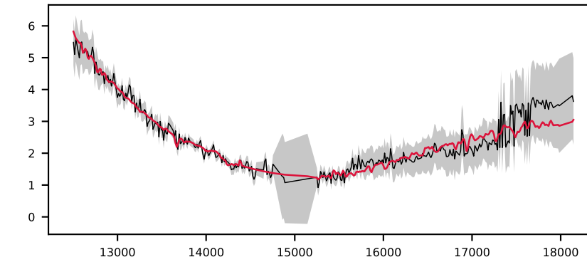
-621578083480547759, 9.7' S/N 19, LSF 13 Å, STAR, v = -450 km/s, \Delta\chi^2=\text{inf} , \chi^2_r=0.3
