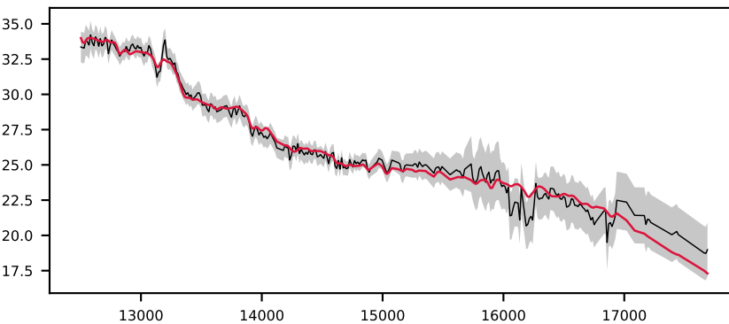
-620898741478742577, 1.4' S/N 131, LSF 13 Å, STAR, v = +300 km/s, \Delta\chi^2=\text{inf} , \chi^2_r=33.0 ✗ unfittable
