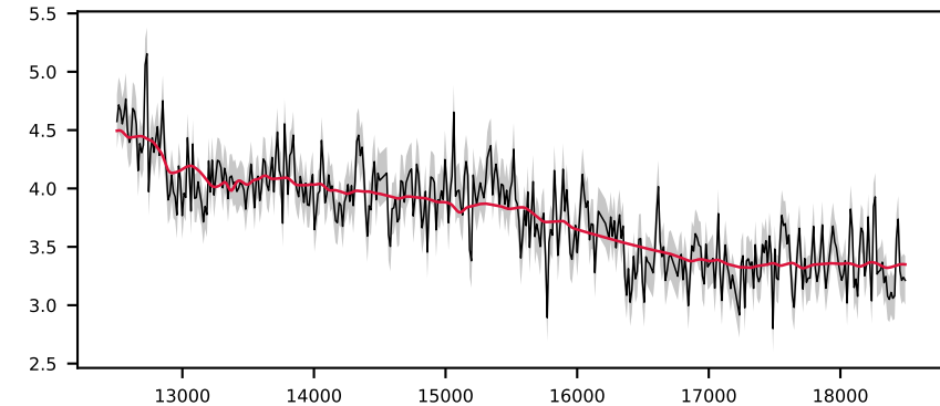
-622765871478705761, 7.3' S/N 18, LSF 33 Å, GALAXY, z = 0.178 , \Delta\chi^2=13 , \chi^2_r=1.1
