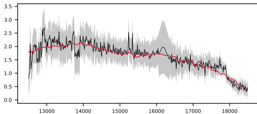
-620531179479394075, 3.2' S/N 13, LSF 16 Å, STAR, v = +150 km/s, \Delta\chi^2=\text{inf} , \chi^2_r=0.3
