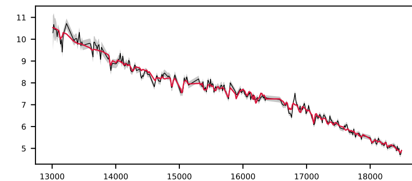
-620058808478431591, 5.0' S/N 57, LSF 12 Å, STAR, v = +0 km/s, \Delta\chi^2=\text{inf} , \chi^2_r=1.2
