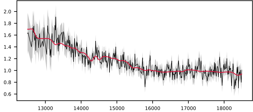
-622159530479386735, 5.3' S/N 12, LSF 46 Å, GALAXY, z = 0.674 , \Delta\chi^2=2 , \chi^2_r=0.7
