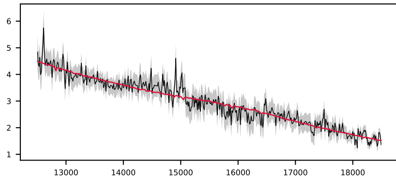
-621311139478620471, 2.4' S/N 28, LSF 20 Å, GALAXY, z = 0.057 , \Delta\chi^2=2 , \chi^2_r=0.2
