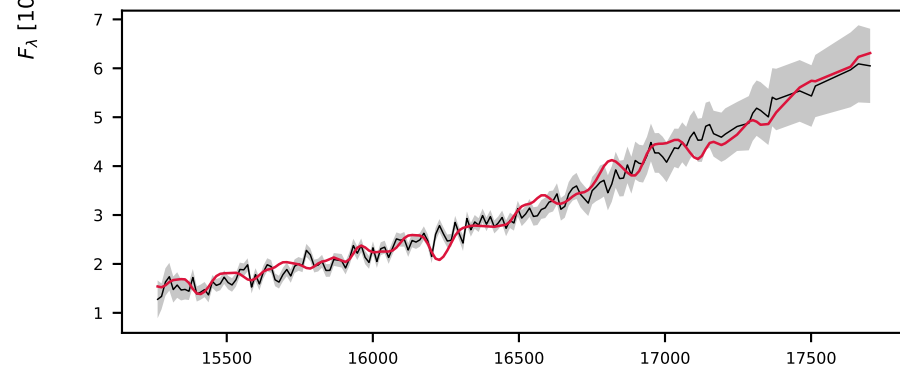
-621596416478346160, 4.4' S/N 20, LSF 19 Å, GALAXY, z = 0.664 , \Delta\chi^2=0 , \chi^2_r=0.7
