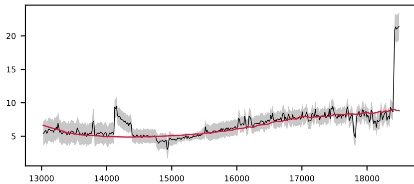
-620702263478765420, 1.7' S/N 54, LSF 21 Å, STAR, v = +600 km/s, \Delta\chi^2=\text{inf} , \chi^2_r=1.0
