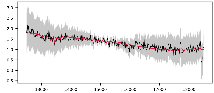
-620563456478388651, 3.9' S/N 13, LSF 27 Å, GALAXY, z = 0.510 , \Delta\chi^2=1 , \chi^2_r=0.8
