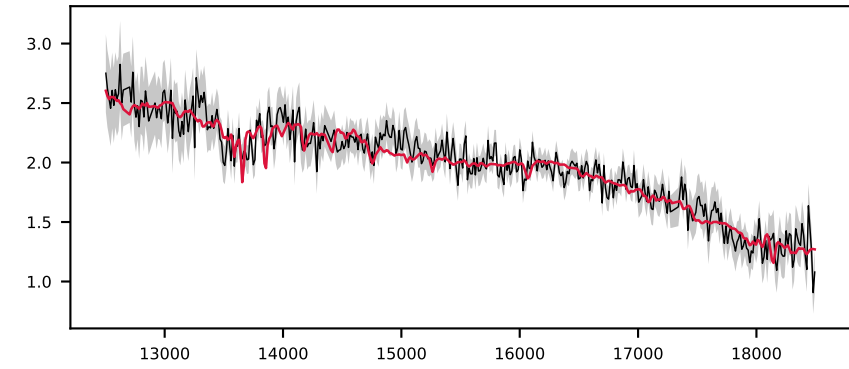
-618919719478751729, 8.5' S/N 20, LSF 30 Å, GALAXY, z = 0.792 , \Delta\chi^2=4 , \chi^2_r=0.7
