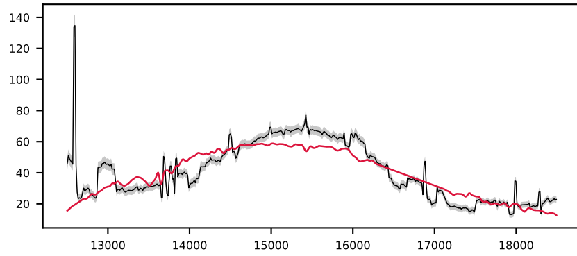
-620942895480507797, 9.2' S/N 121, LSF 35 Å, STAR, v = +0 km/s, \Delta\chi^2=\text{inf} , \chi^2_r=0.6
