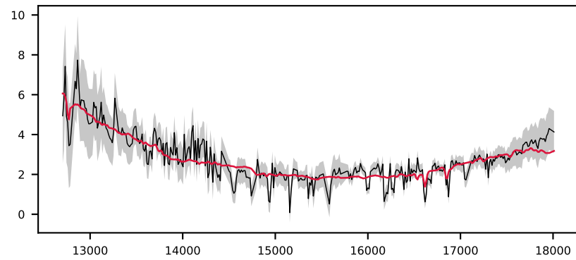
-621338271479840000, 5.4' S/N 20, LSF 22 Å, GALAXY, z = 0.971 , \Delta\chi^2=1 , \chi^2_r=0.8
