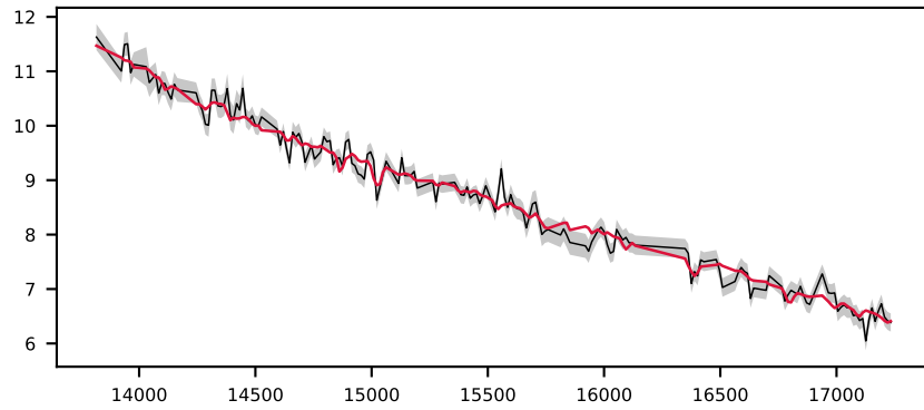
-620968018478659286, 1.9' S/N 54, LSF 10 Å, GALAXY, z = 0.405 , \Delta\chi^2=62 , \chi^2_r=30.7 ✗ unfittable
