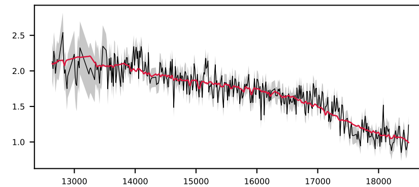
-620281274479082991, 3.0' S/N 13, LSF 11 Å, STAR, v = +300 km/s, \Delta\chi^2=\text{inf} , \chi^2_r=1.3
