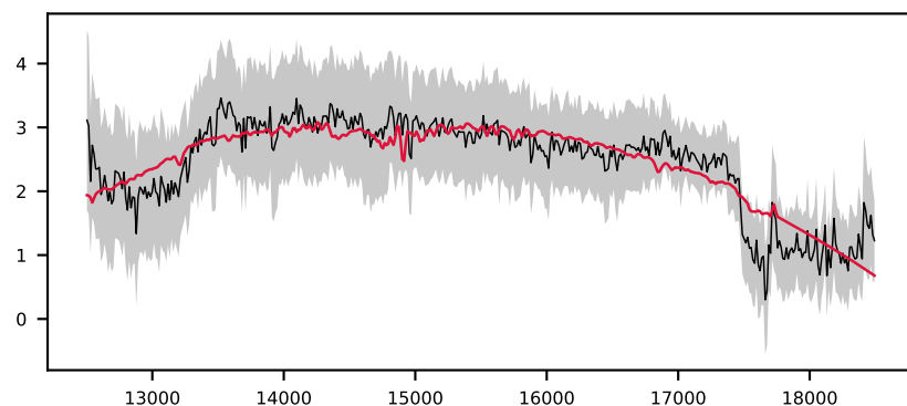
-619657546479169825, 5.6' S/N 22, LSF 13 Å, GALAXY, z = 0.314 , \Delta\chi^2=2 , \chi^2_r=0.2
