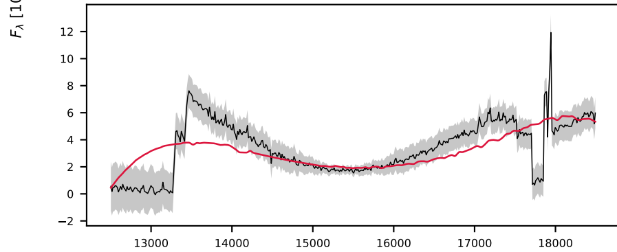
-621454655478706346, 2.4' S/N 31, LSF 20 Å, GALAXY, v = +0 km/s, \Delta\chi^2=11 , \chi^2_r=0.3
