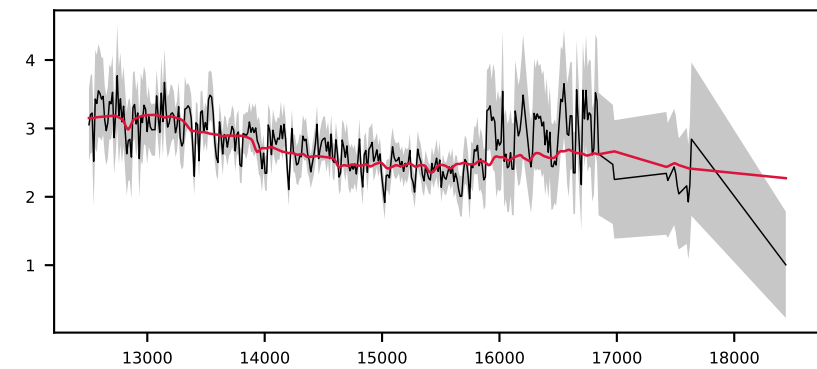
-622201980478806652, 4.9' S/N 19, LSF 15 Å, STAR, v = +300 km/s, \Delta\chi^2=\text{inf} , \chi^2_r=0.6
