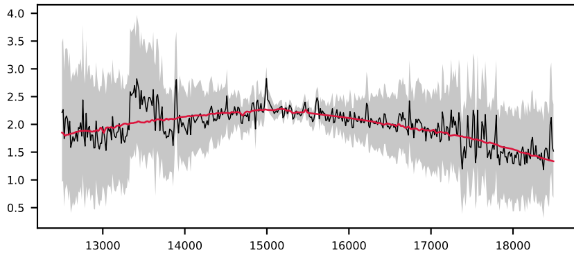
-621484351479752673, 5.1' S/N 20, LSF 35 Å, GALAXY, z = 0.613 , \Delta\chi^2=18 , \chi^2_r=0.7
