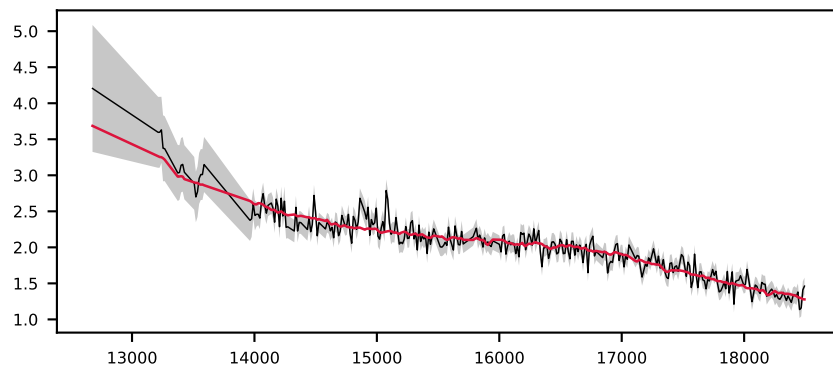
-620308533479025574, 2.8' S/N 16, LSF 13 Å, STAR, v = +150 km/s, \Delta\chi^2=\text{inf} , \chi^2_r=1.0
