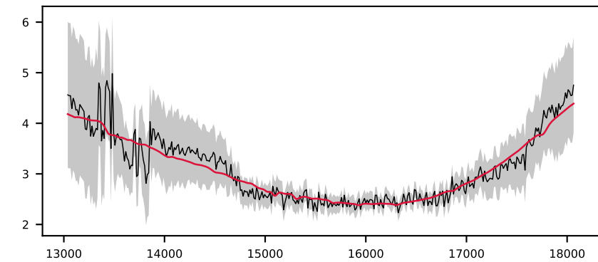
-620575361479251183, 2.4' S/N 28, LSF 17 Å, GALAXY, z = 0.447 , \Delta\chi^2=5 , \chi^2_r=0.3
