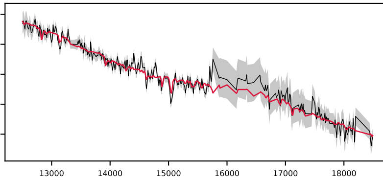
-621993491478657410, 4.4' S/N 38, LSF 15 Å, STAR, v = +600 km/s, \Delta\chi^2=\text{inf} , \chi^2_{\text{r}}=0.5
