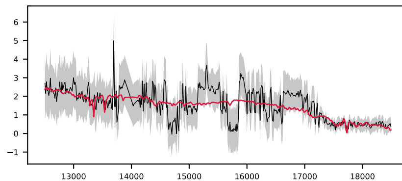
-621865367479591394, 5.1' S/N 13, LSF 12 Å, STAR, v = -450 km/s, \Delta\chi^2=\text{inf} , \chi^2_r=1.0
