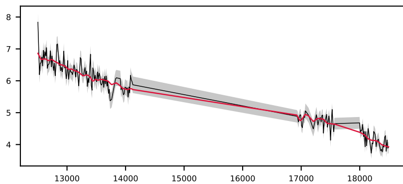
-623204666478810788, 8.9' S/N 24, LSF 32 Å, GALAXY, z = 0.048 , \Delta\chi^2=4 , \chi^2_r=1.1
