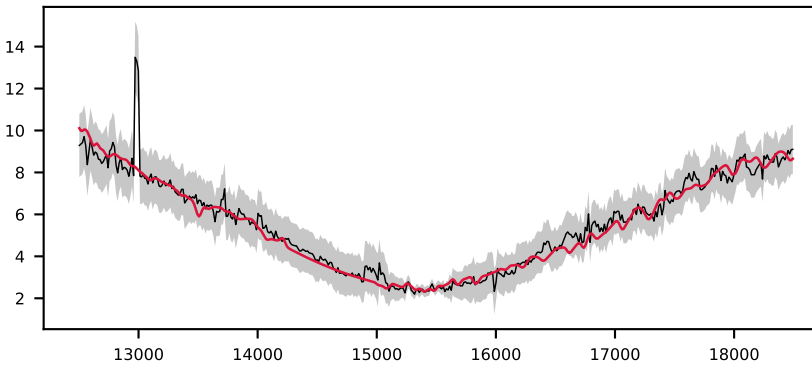
-621472677479482244, 3.6' S/N 54, LSF 13 Å, STAR, v = +0 km/s, \Delta\chi^2=\text{inf} , \chi^2_r=0.3
