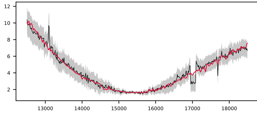
-618554149479065090, 9.9' S/N 38, LSF 31 Å, GALAXY, z = 0.245 , \Delta\chi^2=7 , \chi^2_{\text{r}}=0.5
