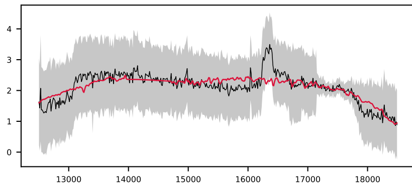
-623395478478862411, 9.6' S/N 20, LSF 10 Å, STAR, v = +600 km/s, \Delta\chi^2=\text{inf} , \chi^2_r=0.3
