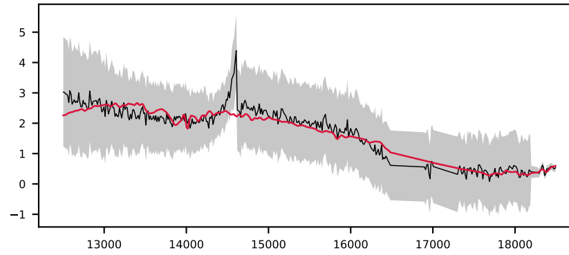
-618909963478906556, 8.4' S/N 16, LSF 12 Å, GALAXY, z = 0.814 , \Delta\chi^2=3 , \chi^2_r=0.4
