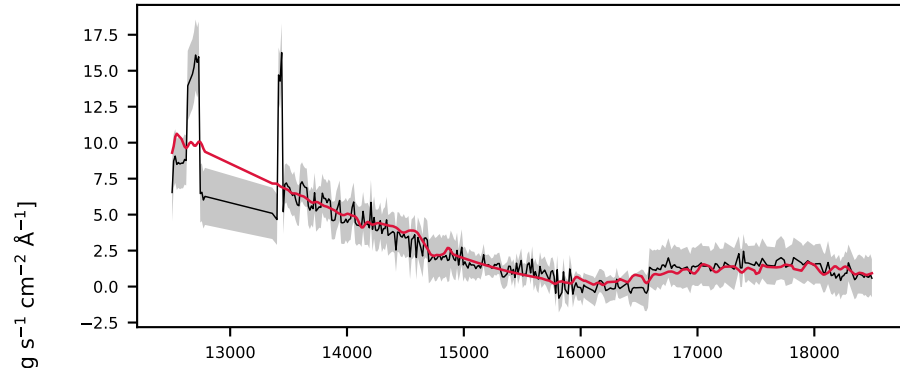
-620703910479506198, 3.4' S/N 13, LSF 12 Å, GALAXY, z = 0.189 , \Delta\chi^2=7 , \chi^2_r=0.8
