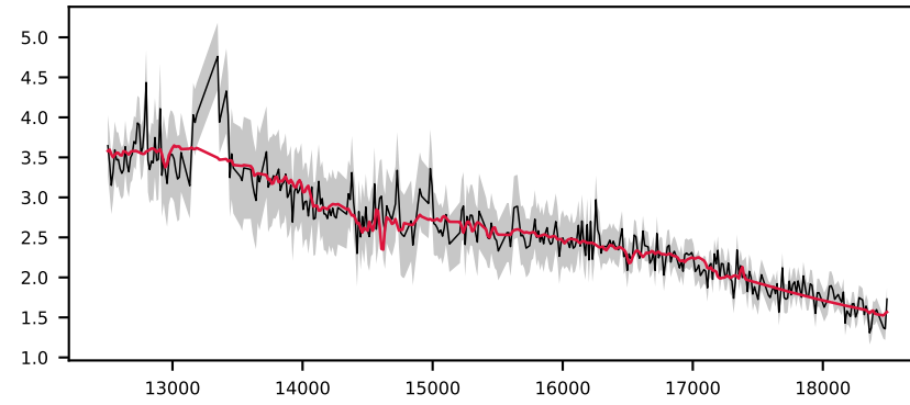
-619677277479249039, 5.6' S/N 20, LSF 13 Å, STAR, v = +150 km/s, \Delta\chi^2=\text{inf} , \chi^2_r=0.8
