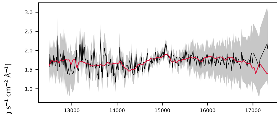
-621751941478768265, 3.2' S/N 14, LSF 13 Å, STAR, v = +300 km/s, \Delta\chi^2=\text{inf} , \chi^2_{\text{r}}=1.2
