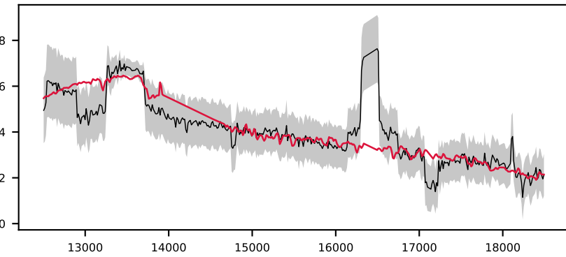
-620434922479046990, 2.3' S/N 38, LSF 14 Å, STAR, v = +450 km/s, \Delta\chi^2=\text{inf} , \chi^2_{\text{r}}=1.5
