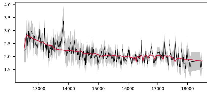
-621985059478303873, 5.6' S/N 17, LSF 28 Å, GALAXY, z = 0.026 , \Delta\chi^2=2 , \chi^2_r=0.4
