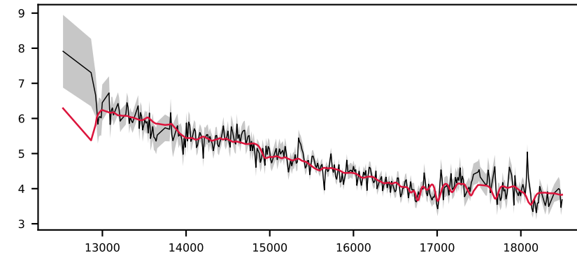
-622532334479612827, 7.3' S/N 25, LSF 24 Å, GALAXY, z = 0.371 , \Delta\chi^2=21 , \chi^2_r=0.4
