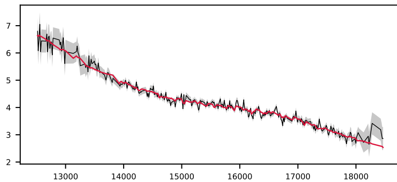
-621371708479623760, 4.2' S/N 39, LSF 14 Å, STAR, v = +0 km/s, \Delta\chi^2=\text{inf} , \chi^2_r=1.1
