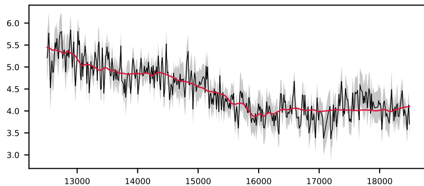
-619164979478871987, 7.4' S/N 22, LSF 22 Å, GALAXY, z = 0.353 , \Delta\chi^2=9 , \chi^2_r=0.4
