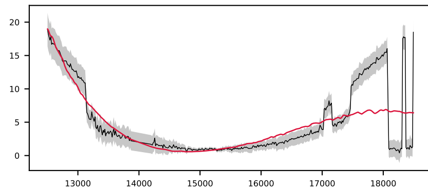
-623311991479524651, 9.9' S/N 22, LSF 12 Å, STAR, v = +0 km/s, \Delta\chi^2=\text{inf} , \chi^2_r=1.3
