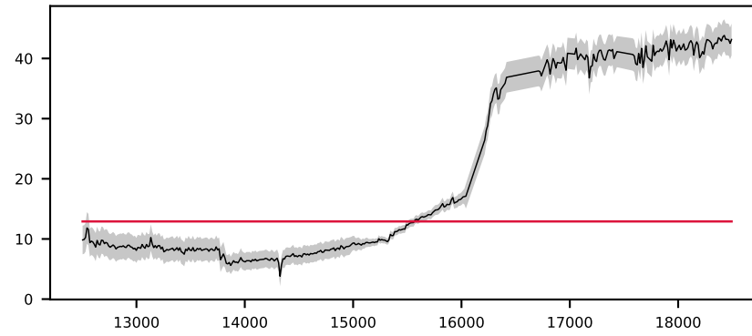
-620763660478692427, 1.9' S/N 60, LSF 14 Å, GALAXY, z = 0.995 , \Delta\chi^2=23 , \chi^2_r=7.8
