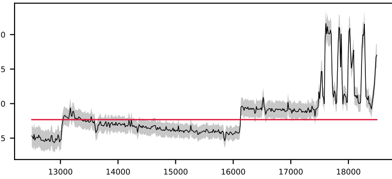
-621179152478672221, 1.9' S/N 60, LSF 9 Å, GALAXY, z = 0.967 , \Delta\chi^2=71 , \chi^2_r=15.0
