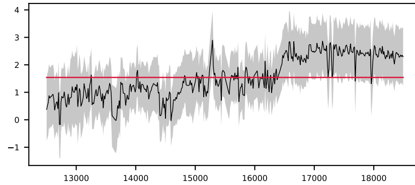
-619626982479764950, 7.3' S/N 15, LSF 35 Å, GALAXY, z = 0.479 , \Delta\chi^2=8 , \chi^2_r=0.7
