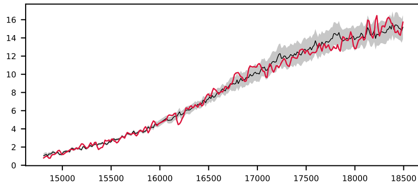
-622803838479977044, 9.4' S/N 55, LSF 13 Å, STAR, v = -300 km/s, \Delta\chi^2=\text{inf} , \chi^2_r=1.6
