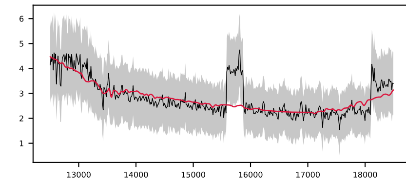
-621054850479308466, 2.0' S/N 24, LSF 18 Å, STAR, v = +450 km/s, \Delta\chi^2=\text{inf} , \chi^2_r=1.8
