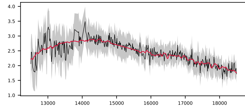
-619892715477807637, 8.3' S/N 23, LSF 13 Å, GALAXY, z = 0.205 , \Delta\chi^2=10 , \chi^2_r=0.9
