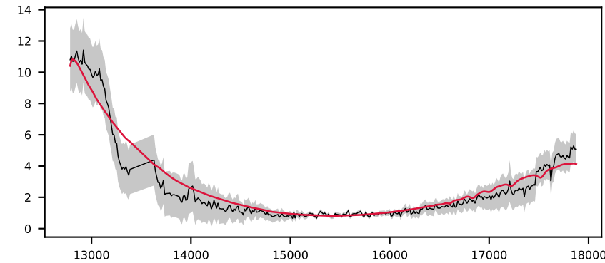
-621239786478571803, 2.6' S/N 15, LSF 18 Å, GALAXY, z = 0.943 , \Delta\chi^2=2 , \chi^2_r=0.6
