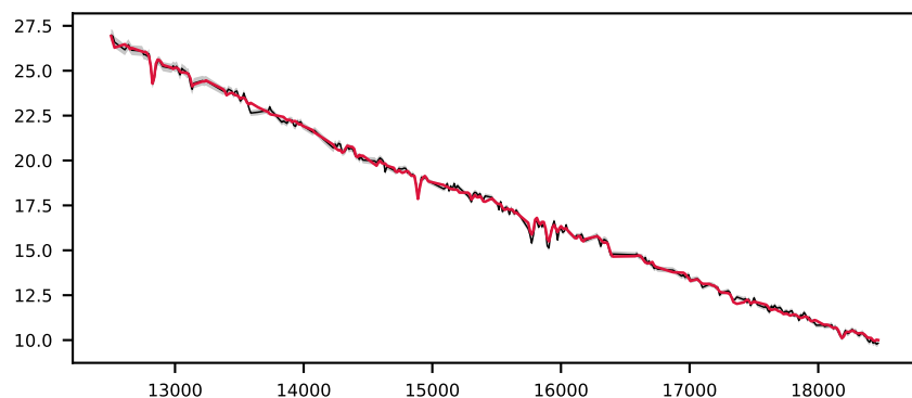
-619563543477678596, 9.7' S/N 124, LSF 15 Å, STAR, v = +150 km/s, \Delta\chi^2=\text{inf} , \chi^2_r=1.3
