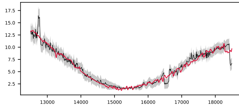
-620903417479280005, 1.9' S/N 51, LSF 19 Å, GALAXY, z = 0.050 , \Delta\chi^2=7 , \chi^2_r=3.3
