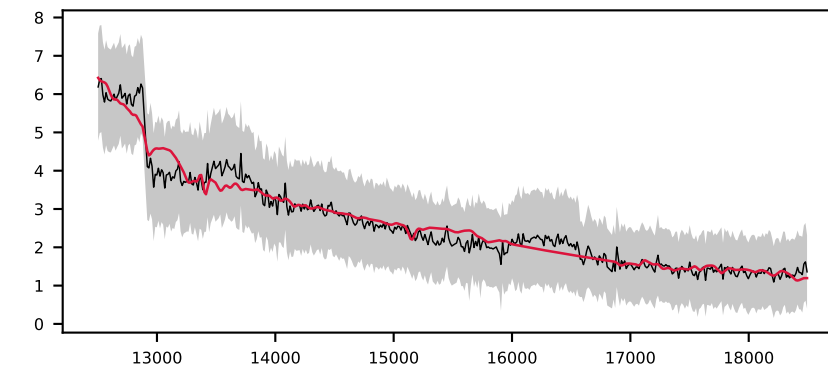
-621491392479121951, 2.2' S/N 20, LSF 16 Å, GALAXY, z = 0.182 , \Delta\chi^2=2 , \chi^2_r=0.1
