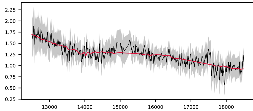
-619907322478310107, 5.9' S/N 13, LSF 18 Å, GALAXY, z = 0.236 , \Delta\chi^2=1 , \chi^2_r=0.2
