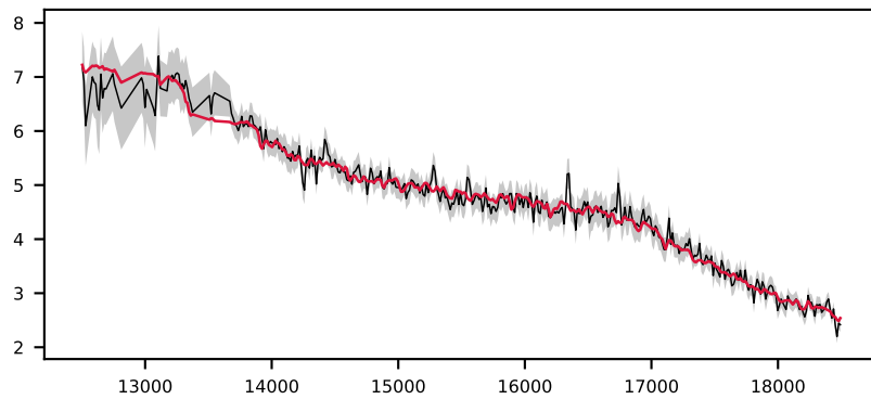
-618929606478865290, 8.4' S/N 40, LSF 34 Å, GALAXY, z = 0.569 , \Delta\chi^2=2 , \chi^2_r=1.0
