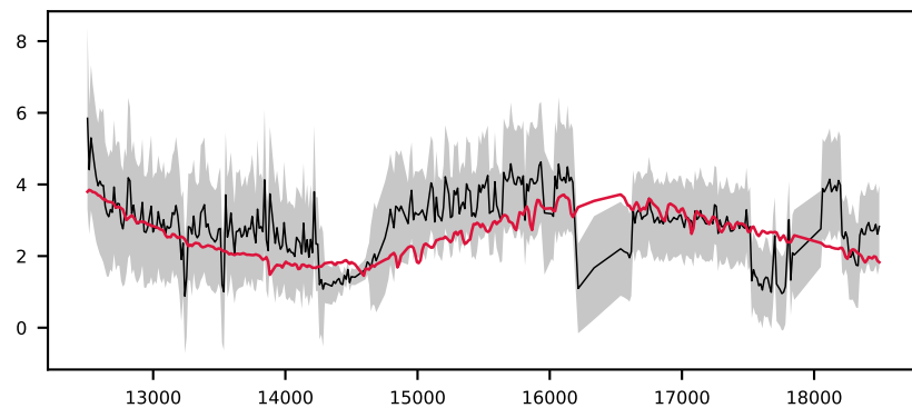
-619256423479092478, 7.1' S/N 22, LSF 13 Å, STAR, v = -150 km/s, \Delta\chi^2=\text{inf} , \chi^2_r=0.6
