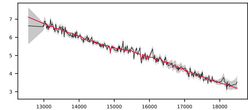
-619023527478186901, 9.3' S/N 40, LSF 26 Å, STAR, v = -600 km/s, \Delta\chi^2=\text{inf} , \chi^2_r=0.5
