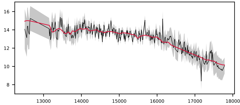
-619035164478305339, 8.9' S/N 34, LSF 12 Å, STAR, v = +600 km/s, \Delta\chi^2=\text{inf} , \chi^2_r=0.7
