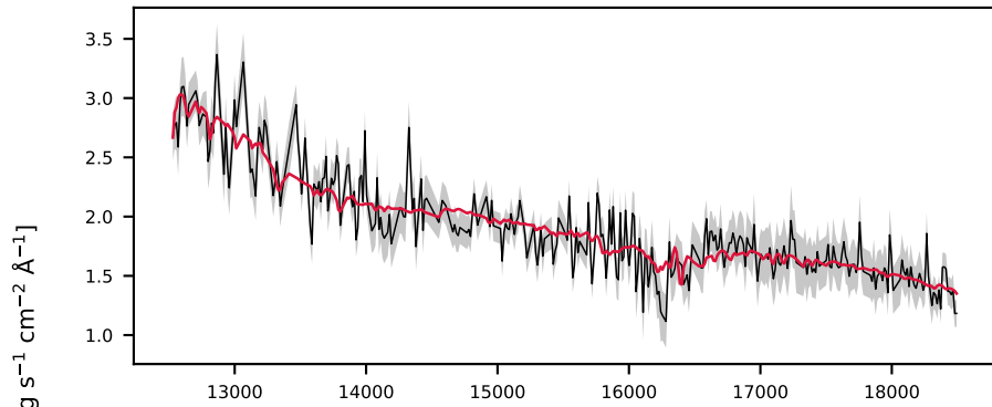
-622345318479373831, 5.9' S/N 15, LSF 12 Å, STAR, v = +300 km/s, \Delta\chi^2=\text{inf} , \chi^2_r=0.8
