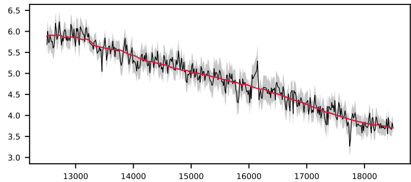
-623038177478682032, 8.4' S/N 39, LSF 13 Å, STAR, v = +0 km/s, \Delta\chi^2=\text{inf} , \chi^2_r=1.5
