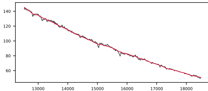
-620816989477562303, 8.5' S/N 260, LSF 63 Å, STAR, v = +0 km/s, \Delta\chi^2=\text{inf} , \chi^2_r=3.5
