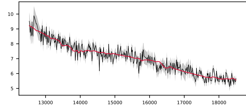
-620470097479765462, 5.2' S/N 26, LSF 13 Å, STAR, v = +0 km/s, \Delta\chi^2=\text{inf} , \chi^2_r=1.3
