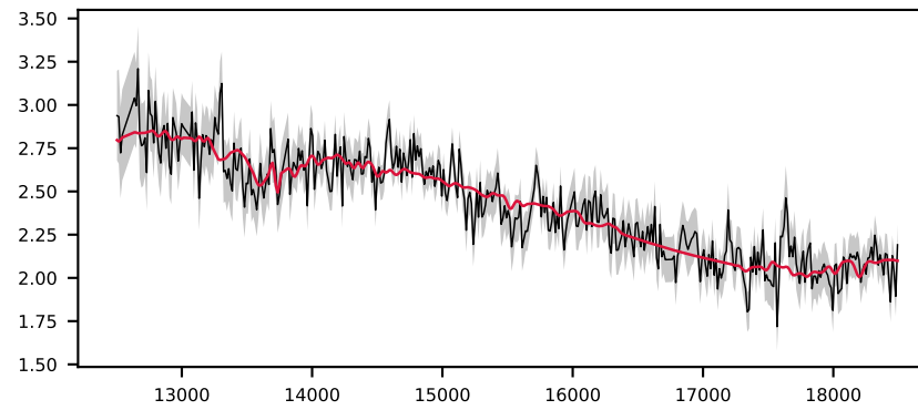
-622307429479044027, 5.3' S/N 24, LSF 13 Å, STAR, v = +150 km/s, \Delta\chi^2=\text{inf} , \chi^2_r=0.9
