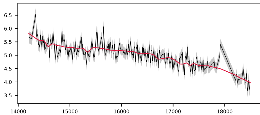
-621510610479074022, 2.1' S/N 24, LSF 16 Å, STAR, v = -300 km/s, \Delta\chi^2=\text{inf} , \chi^2_r=0.1
