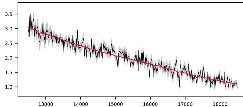
-620965522479394673, 2.6' S/N 18, LSF 11 Å, GALAXY, z = 0.070 , \Delta\chi^2=6 , \chi^2_r=0.5
