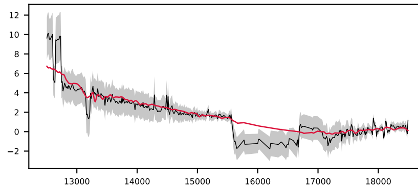
-620548088478658608, 2.6' S/N 14, LSF 22 Å, GALAXY, z = 0.445 , \Delta\chi^2=0 , \chi^2_{\text{r}}=0.4
