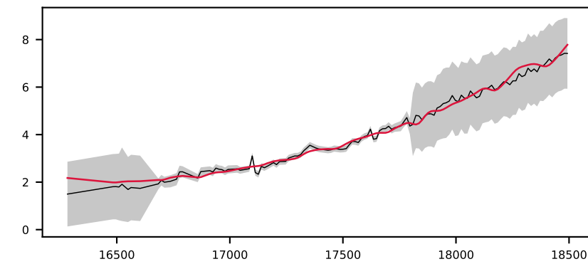
-620643150478765697, 1.9' S/N 30, LSF 43 Å, GALAXY, z = 0.025 , \Delta\chi^2=25 , \chi^2_r=0.7
