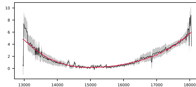
-621060990479645371, 4.1' S/N 18, LSF 24 Å, GALAXY, z = 0.177 , \Delta\chi^2=4 , \chi^2_r=0.2
