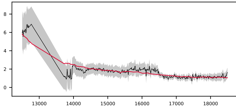
-619663433479166864, 5.5' S/N 15, LSF 14 Å, GALAXY, z = 0.301 , \Delta\chi^2=4 , \chi^2_{\text{r}}=0.2
