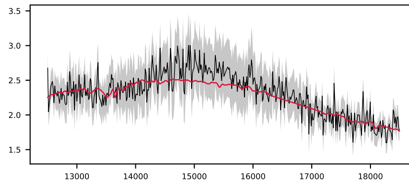
-619715355478476221, 6.0' S/N 18, LSF 11 Å, STAR, v = -450 km/s, \Delta\chi^2=\text{inf} , \chi^2_r=1.2
