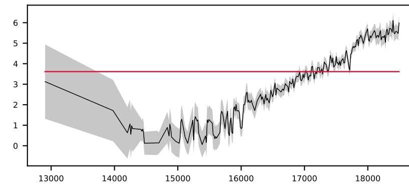
-620507657478751064, 2.4' S/N 23, LSF 16 Å, GALAXY, v = +0 km/s, \Delta\chi^2=0 , \chi^2_r=16.1
