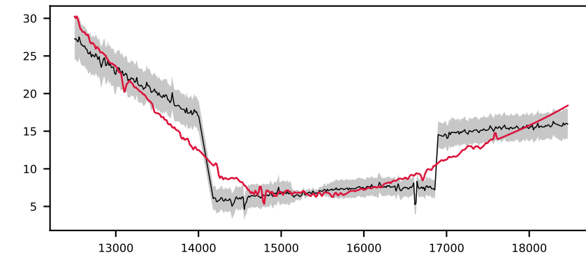
-618722043478606204, 9.4' S/N 79, LSF 44 Å, GALAXY, z = 0.182 , \Delta\chi^2=7 , \chi^2_r=1.7
