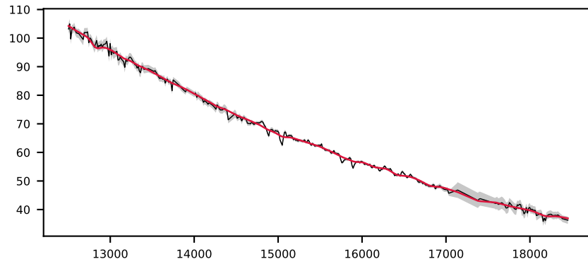
-621559968479961993, 6.4' S/N 205, LSF 61 Å, STAR, v = +150 km/s, \Delta\chi^2=\text{inf} , \chi^2_r=1.3
