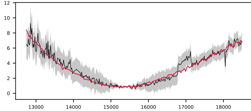
-621229455478613006, 2.3' S/N 25, LSF 12 Å, GALAXY, z = 0.069 , \Delta\chi^2=6 , \chi^2_r=0.2
