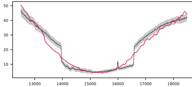
-620850488478751002, 1.5' S/N 109, LSF 14 Å, GALAXY, z = 0.093 , \Delta\chi^2=17 , \chi^2_r=15.7
