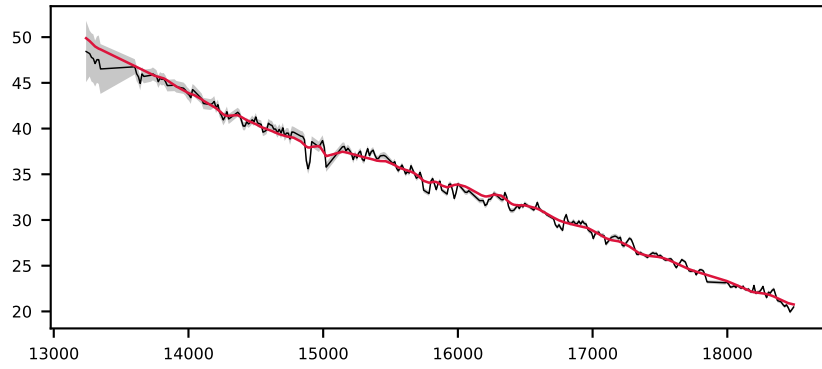
-623253550479453354, 9.5' S/N 167, LSF 70 Å, STAR, v = +450 km/s, \Delta\chi^2=\text{inf} , \chi^2_r=0.4
