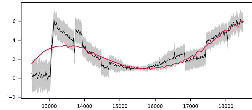
-620689211477771774, 7.3' S/N 22, LSF 12 Å, STAR, v = +0 km/s, \Delta\chi^2=\text{inf} , \chi^2_r=0.8
