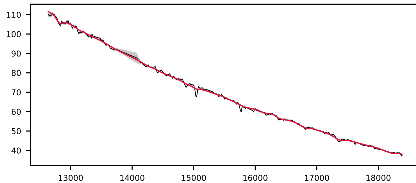
-620879551479596400, 3.8' S/N 232, LSF 45 Å, STAR, v = +0 km/s, \Delta\chi^2=\text{inf} , \chi^2_r=3.0
