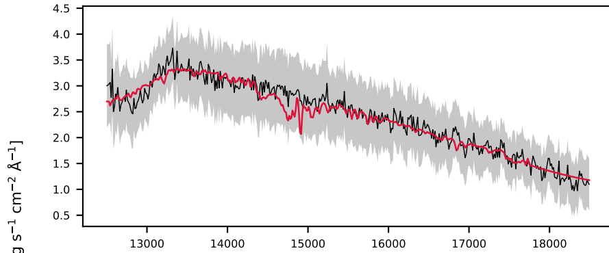
-621259315477750892, 7.4' S/N 24, LSF 13 Å, STAR, v = +0 km/s, \Delta\chi^2=\text{inf} , \chi^2_r=1.6
