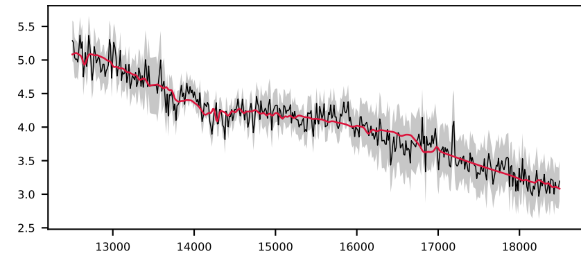
-619795069479477170, 5.7' S/N 34, LSF 12 Å, STAR, v = +150 km/s, \Delta\chi^2=\text{inf} , \chi^2_r=0.8
