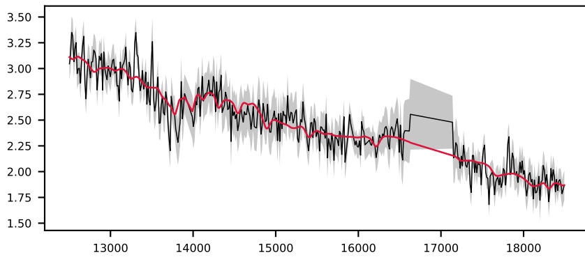
-620846516478398277, 3.5' S/N 20, LSF 12 Å, GALAXY, v = +0 km/s, \Delta\chi^2=0 , \chi^2_r=39.0 ✗ unfittable
