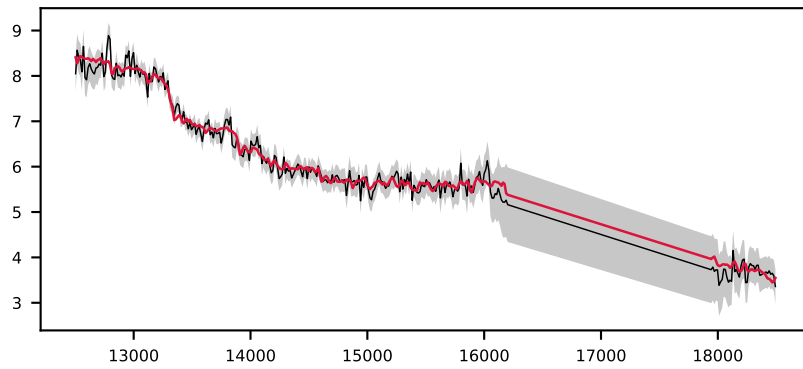
-619924857479205031, 4.6' S/N 52, LSF 13 Å, STAR, v = +0 km/s, \Delta\chi^2=\text{inf} , \chi^2_r=1.0
