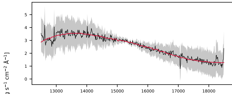
-621175732477663186, 7.9' S/N 24, LSF 17 Å, GALAXY, z = 0.068 , \Delta\chi^2=6 , \chi^2_r=0.4
