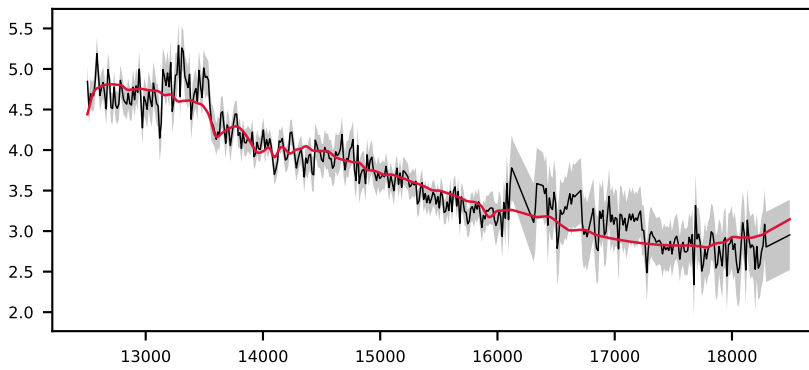
-620942435478631852, 2.0' S/N 30, LSF 12 Å, STAR, v = +300 km/s, \Delta\chi^2=\text{inf} , \chi^2_r=5.7
