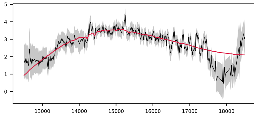
-621596416478346160, 4.4' S/N 20, LSF 19 Å, GALAXY, z = 0.664 , \Delta\chi^2=0 , \chi^2_r=0.7
