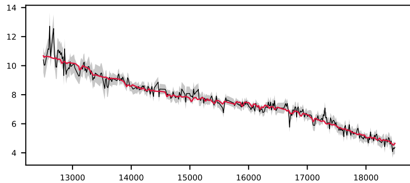
-621637533479939991, 6.4' S/N 57, LSF 13 Å, STAR, v = +0 km/s, \Delta\chi^2=\text{inf} , \chi^2_r=0.7
