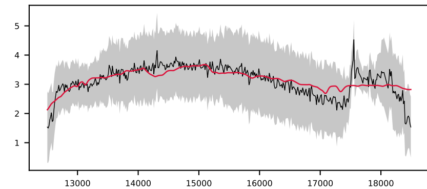
-620893614478413240, 3.4' S/N 24, LSF 27 Å, GALAXY, z = 1.001 , \Delta\chi^2=2 , \chi^2_r=0.1
