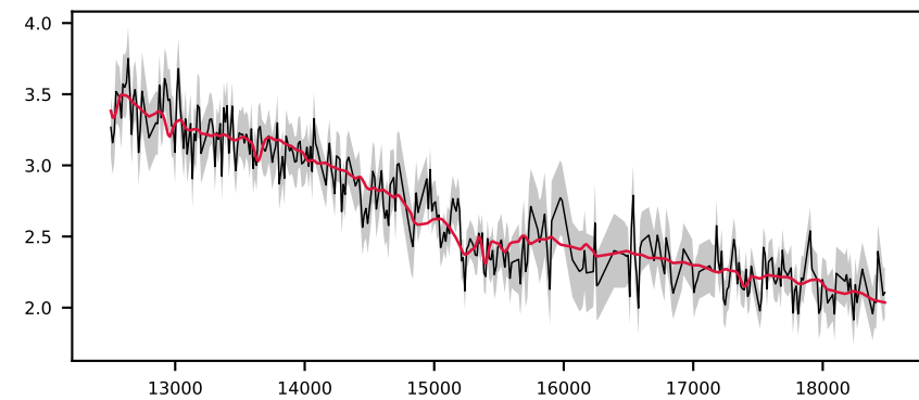
-623429068478939945, 9.8' S/N 20, LSF 20 Å, GALAXY, z = 0.492 , \Delta\chi^2=17 , \chi^2_r=1.1
