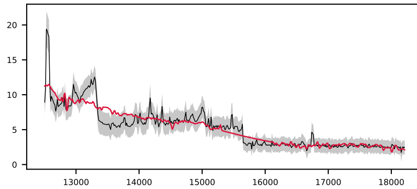
-620748704478690788, 2.0' S/N 34, LSF 15 Å, GALAXY, z = 0.036 , \Delta\chi^2=26 , \chi^2_r=8.6
