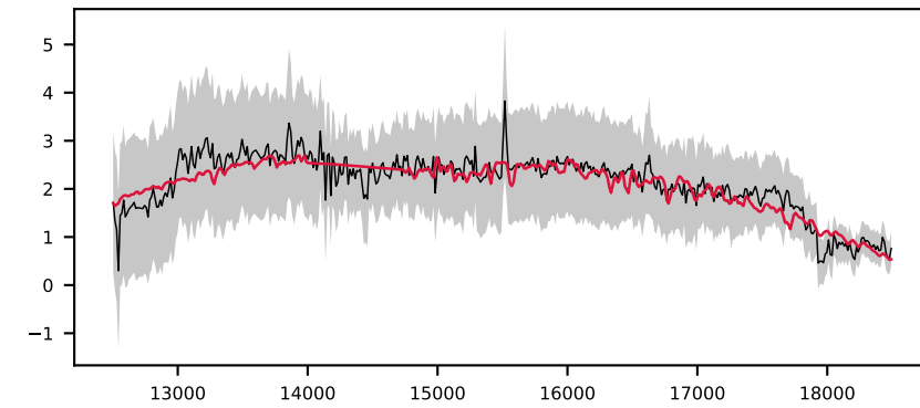
-621549597479034131, 2.2' S/N 19, LSF 14 Å, GALAXY, z = 0.479 , \Delta\chi^2=1 , \chi^2_r=0.1
