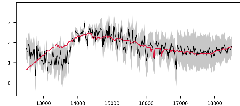
-622318100478703497, 5.5' S/N 12, LSF 13 Å, STAR, v = +600 km/s, \Delta\chi^2=\text{inf} , \chi^2_r=1.0
