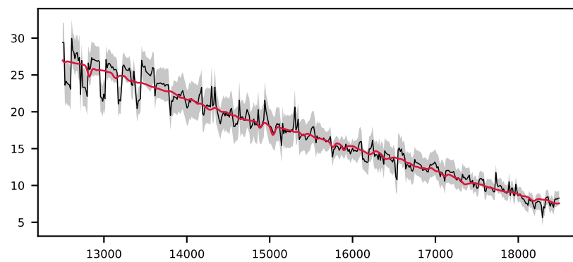
-621334953478735189, 1.9' S/N 78, LSF 19 Å, GALAXY, z = 0.029 , \Delta\chi^2=12 , \chi^2_r=0.6
