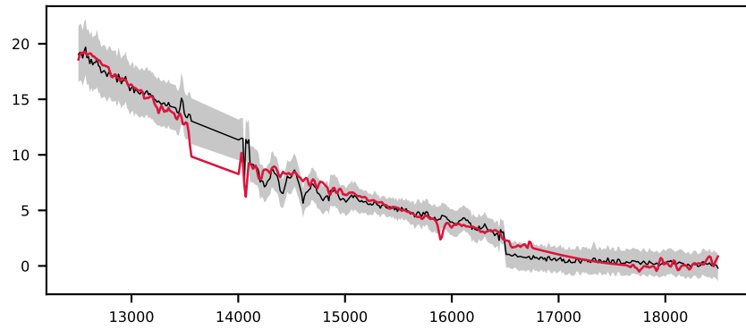
-620769600479330374, 2.4' S/N 38, LSF 12 Å, GALAXY, z = 0.092 , \Delta\chi^2=14 , \chi^2_{\text{r}}=0.2
