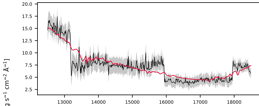
-619069080479719103, 9.0' S/N 44, LSF 13 Å, STAR, v = +150 km/s, \Delta\chi^2=\text{inf} , \chi^2_r=1.0
