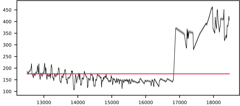
-618925920478984815, 8.4' S/N 245, LSF 56 Å, STAR, v = +0 km/s, \Delta\chi^2=\text{inf} , \chi^2_r=4.2
