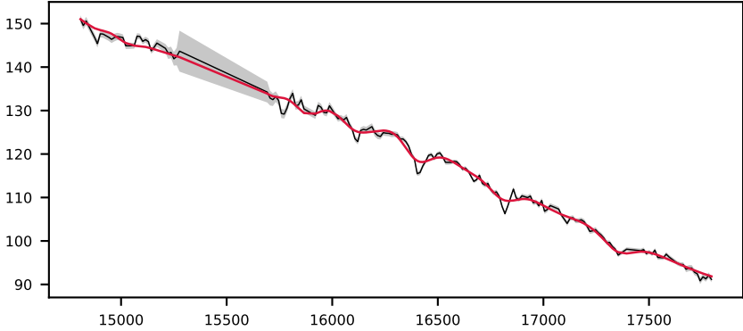
-621038417478028123, 5.7' S/N 250, LSF 65 Å, STAR, v = +0 km/s, \Delta\chi^2=\text{inf} , \chi^2_r=0.9
