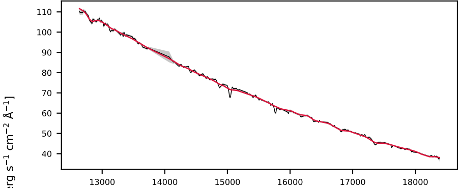
-620816989477562303, 8.5' S/N 260, LSF 63 Å, STAR, v = +0 km/s, \Delta\chi^2=\text{inf} , \chi^2_r=3.5
