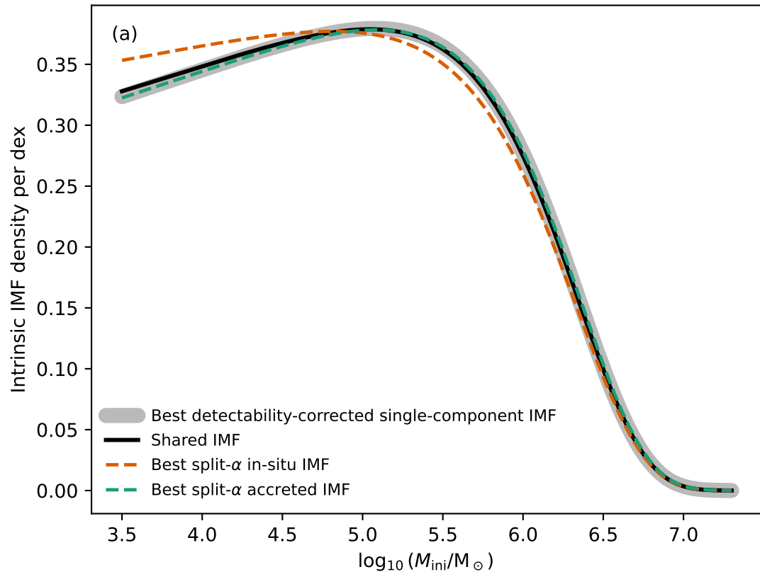
Shared versus split- \alpha IMF fits
