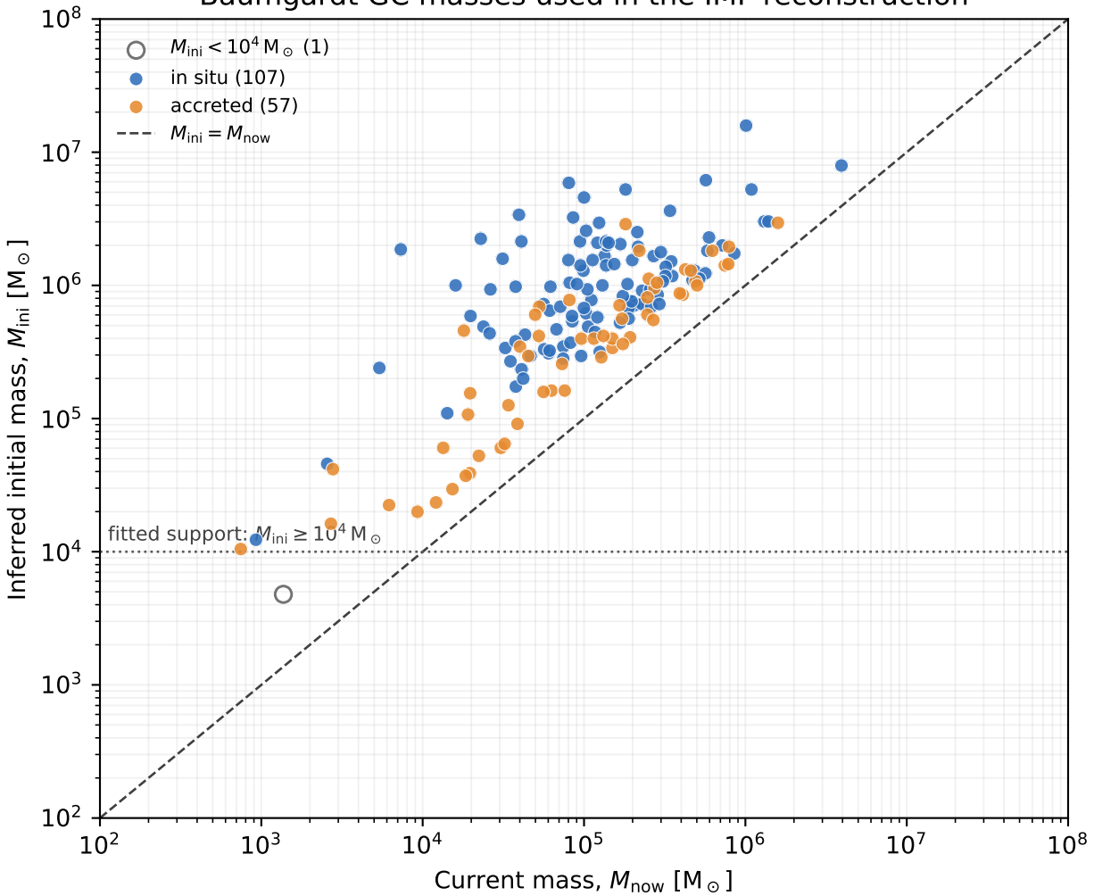
Baumgardt GC masses used in the IMF reconstruction
