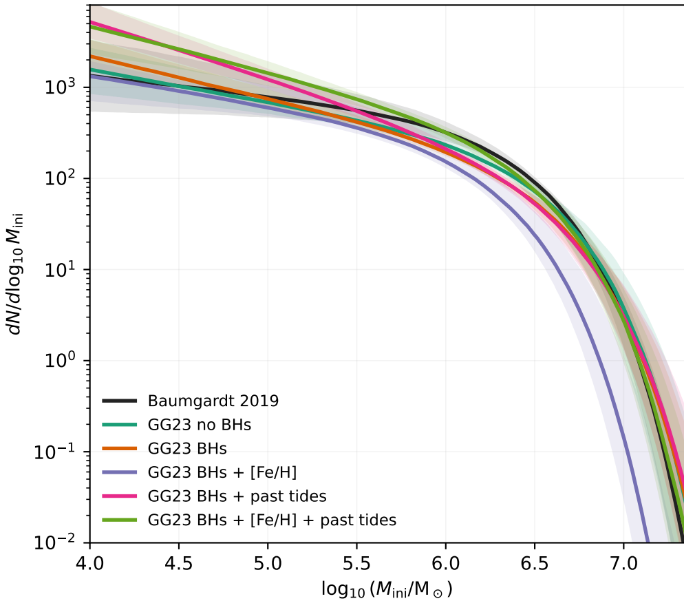
Differential IMF
