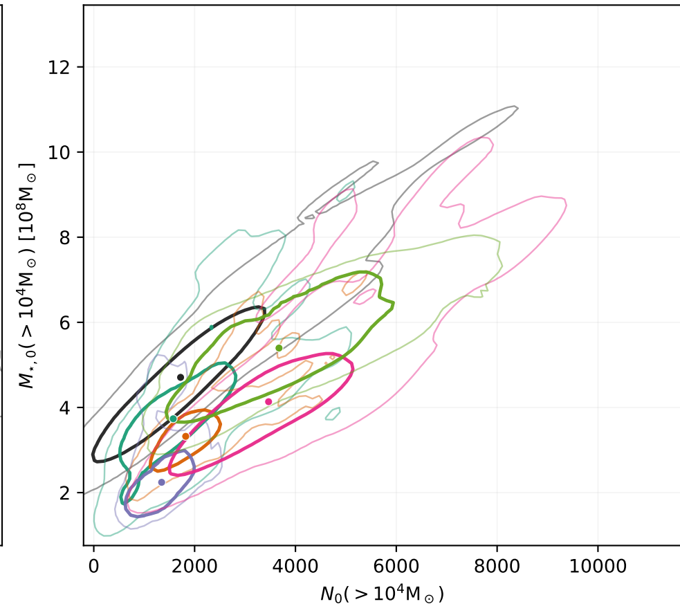
Birth population
