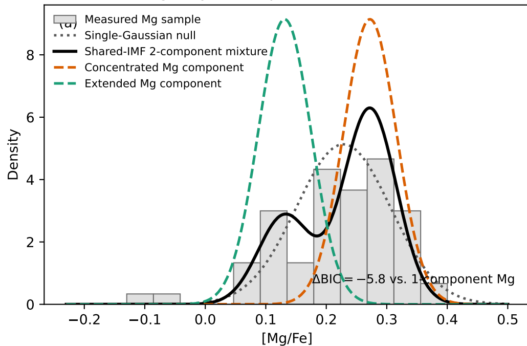
Mg-only blind split with shared IMF
