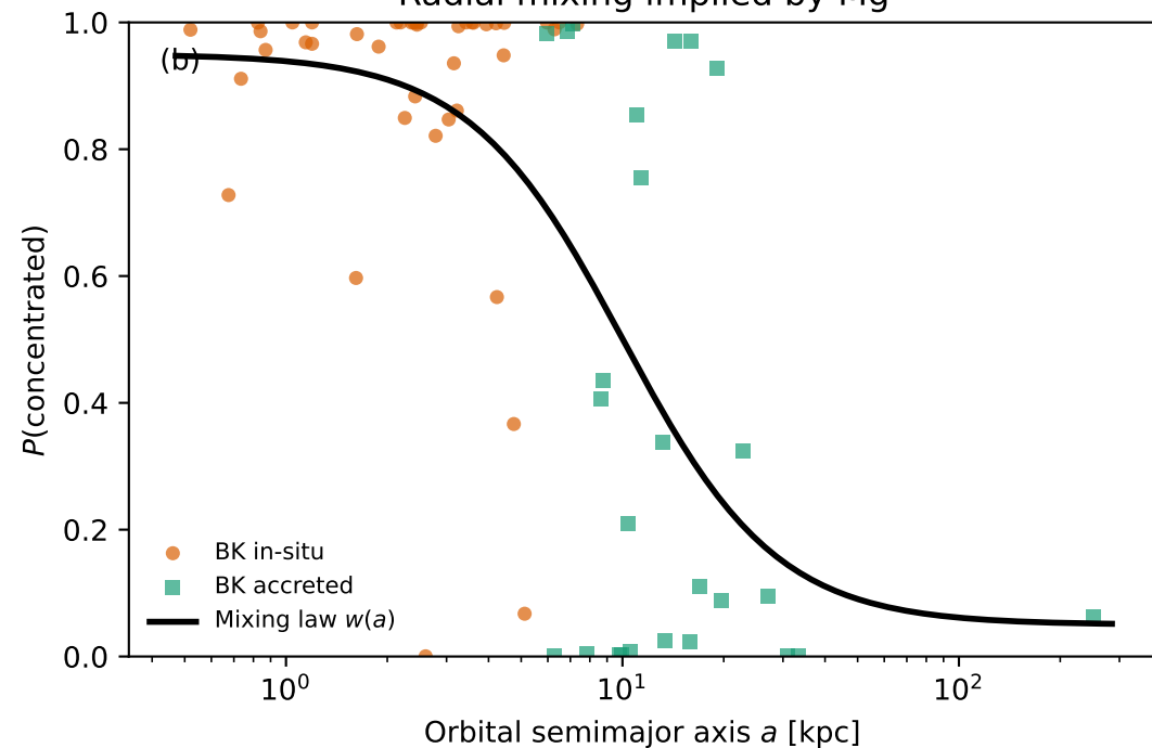
Radial mixing implied by Mg
