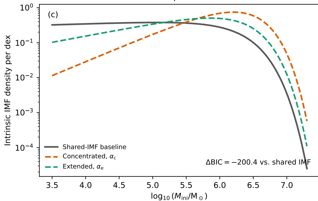
Conditional split- \alpha extension
