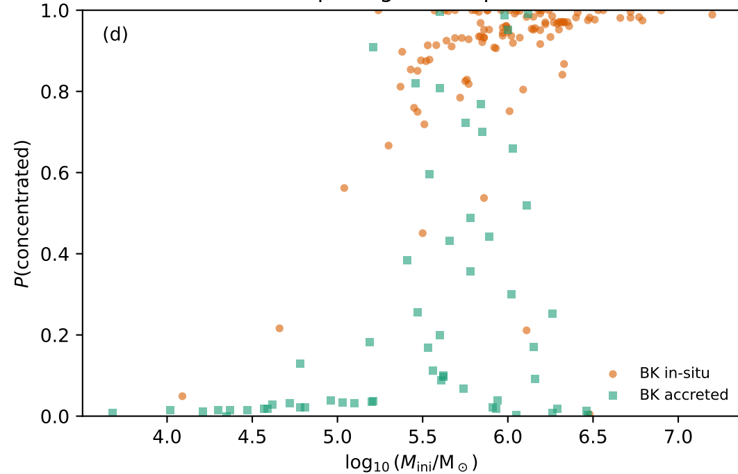
Mass sharpening in the split- \alpha model
