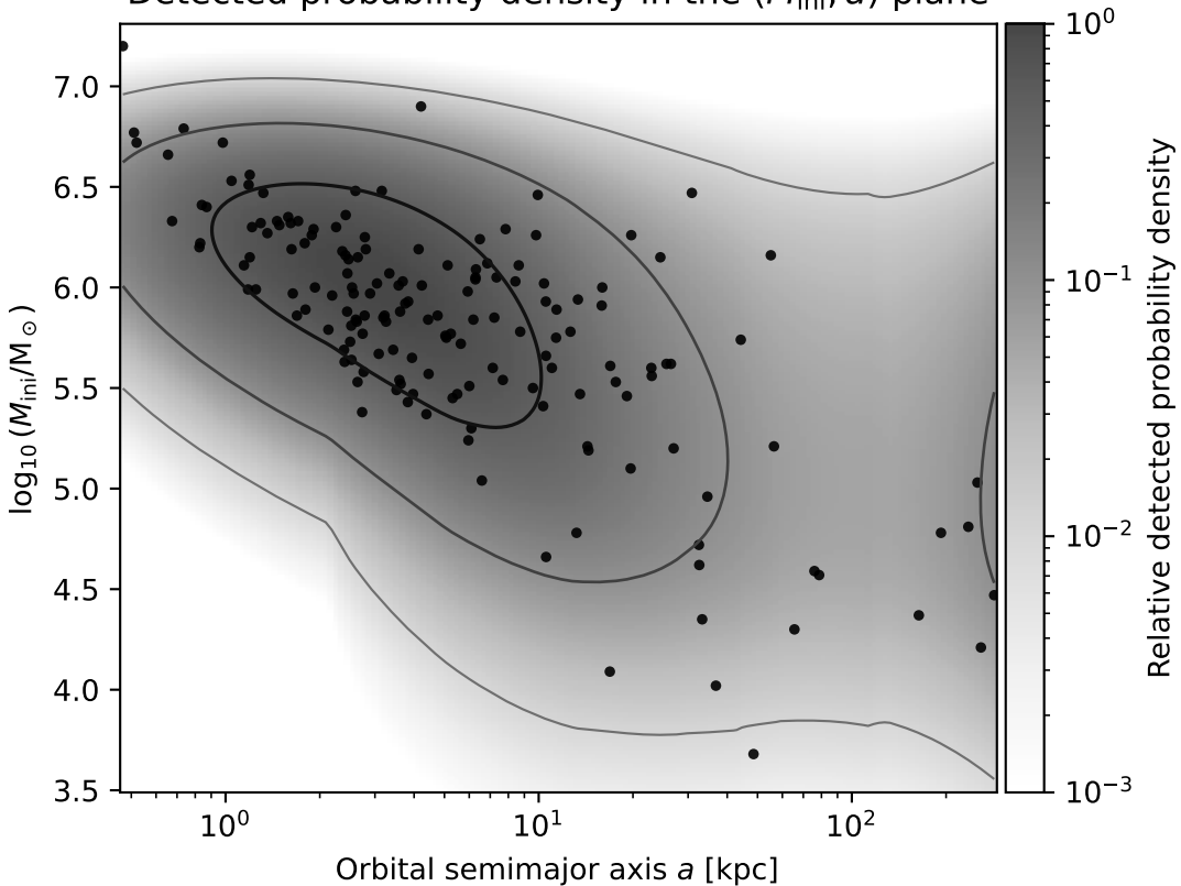
Detected probability density in the ( M_{\text{ini}}, a ) plane
