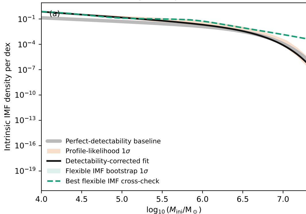
Single-component IMF
