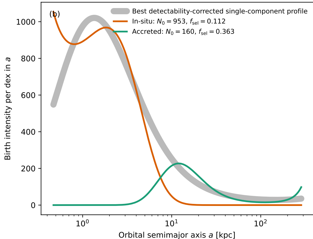
Best shared-IMF two-component model
