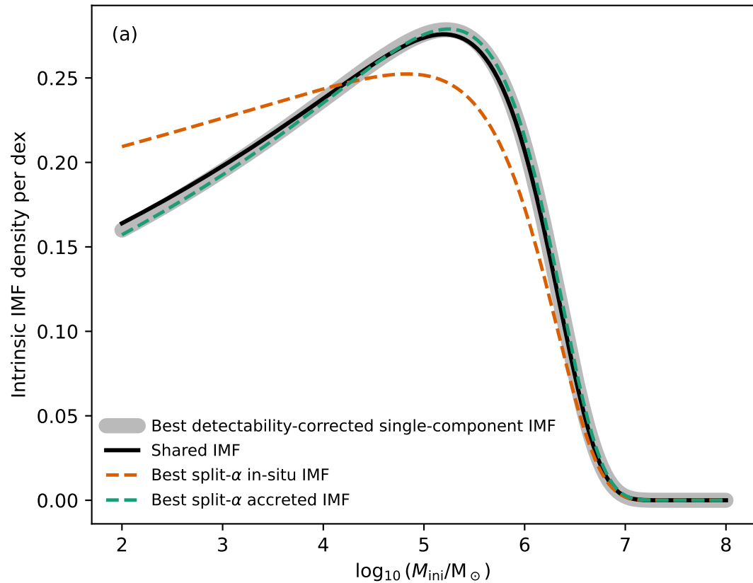
Shared versus split- \alpha IMF fits
