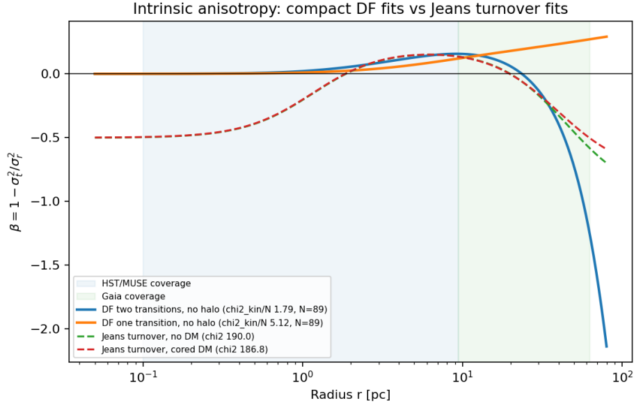
Figure 5: Intrinsic anisotropy of the two-transition fit (no halo) against the one-transition fit and the Jeans turnover fits.
