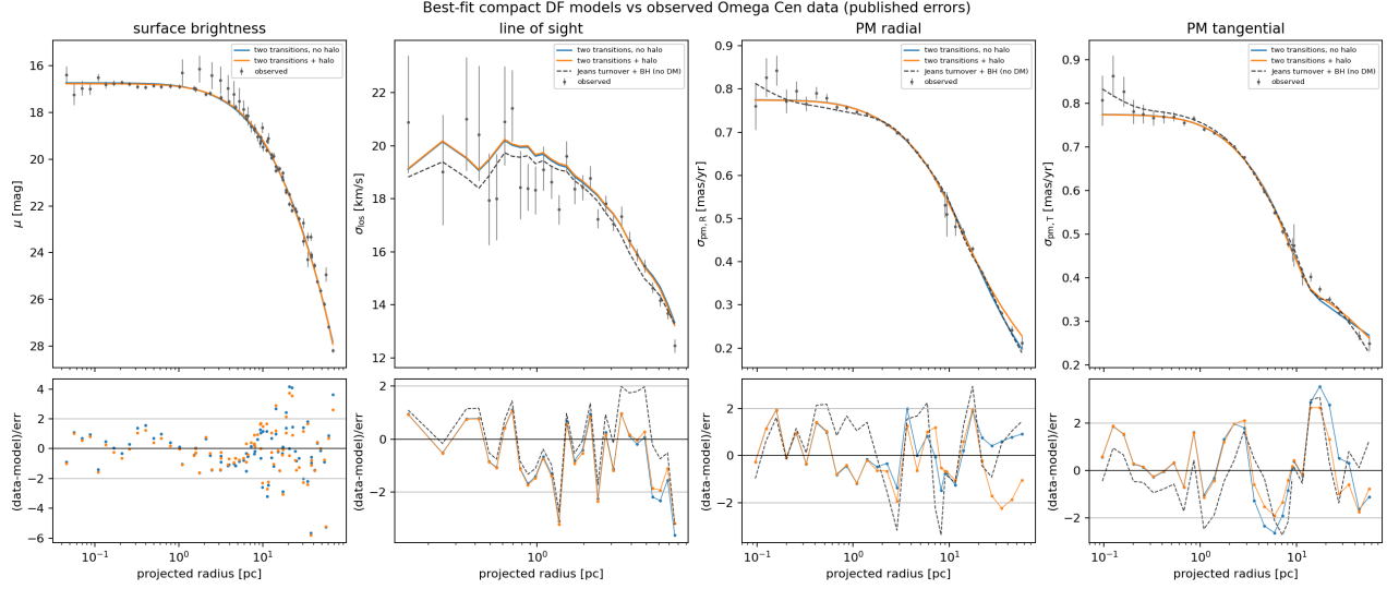
Figure 7: Best two-transition fits without (blue) and with (orange) a halo, and the rung-2 Jeans turnover fit (dashed; kinematics only). Bottom: (data–model)/error, with \pm 2 lines.
