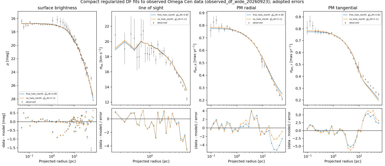
Figure 2: Best one-transition fits (wide bounds) with and without a halo. Top: surface brightness, LOS and PM dispersions with published errors. Bottom: normalized residuals (data–model)/error.
