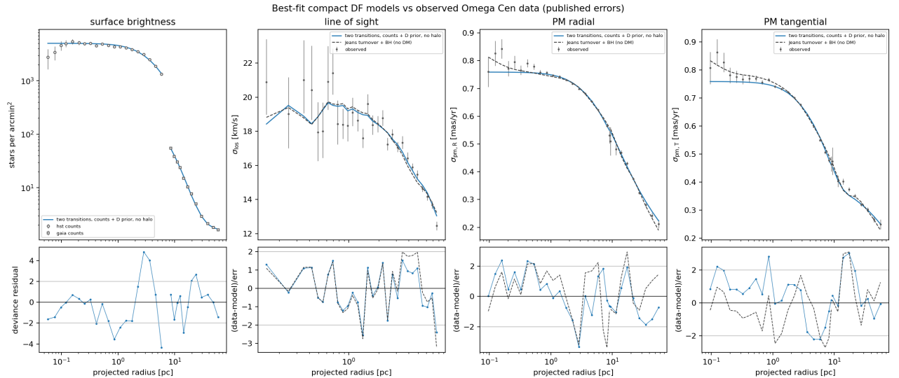
Figure 9: The counts-based two-transition fit (no halo). Left: HST and Gaia surface number densities with Poisson errors and the model \mu_i/A_i ; bottom row: deviance residuals for the counts, (\text{data} - \text{model})/\text{error} for the kinematics. Dashed: the rung-2 Jeans turnover fit (kinematics only).
