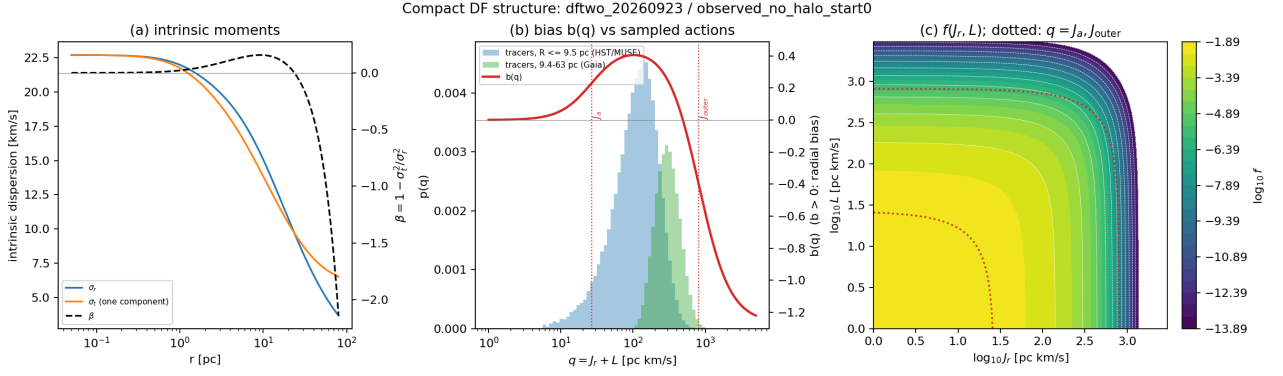
Figure 6: Structure of the two-transition fit (no halo). (a) Intrinsic \sigma_r , one-component \sigma_t and \beta(r) . (b) The bias b(q) over the q distributions of tracers in the HST/MUSE and Gaia projected ranges. (c) \log_{10} f in the (J_r, L) plane ( J_z = 0 ); dotted lines mark q = J_a and q = J_{\text{outer}} .
