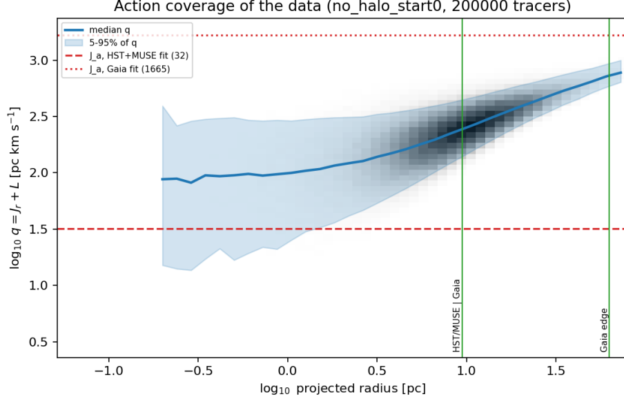
Figure 4: Distribution of q = J_r + L of DF tracers against projected radius, with 5–95% quantiles. Horizontal lines mark the J_a of the HST+MUSE-only (32) and Gaia-only (1665) fits.
