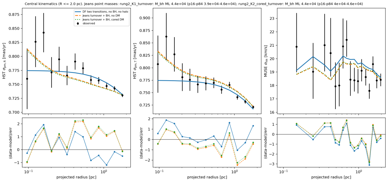
Figure 10: Central kinematics ( R \leq 2 \text{ pc} ) with the no-BH two-transition DF and the Jeans turnover fits with a point mass. Bottom: (data–model)/error.
