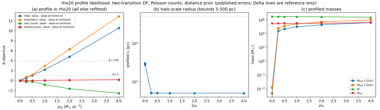
Figure 11: (a) The objective and its components relative to the minimum against \rho_{20} ; the \Delta = 1 and 3.84 lines are reference values, not calibrated intervals. (b) The profiled r_s . (c) Profiled masses.
