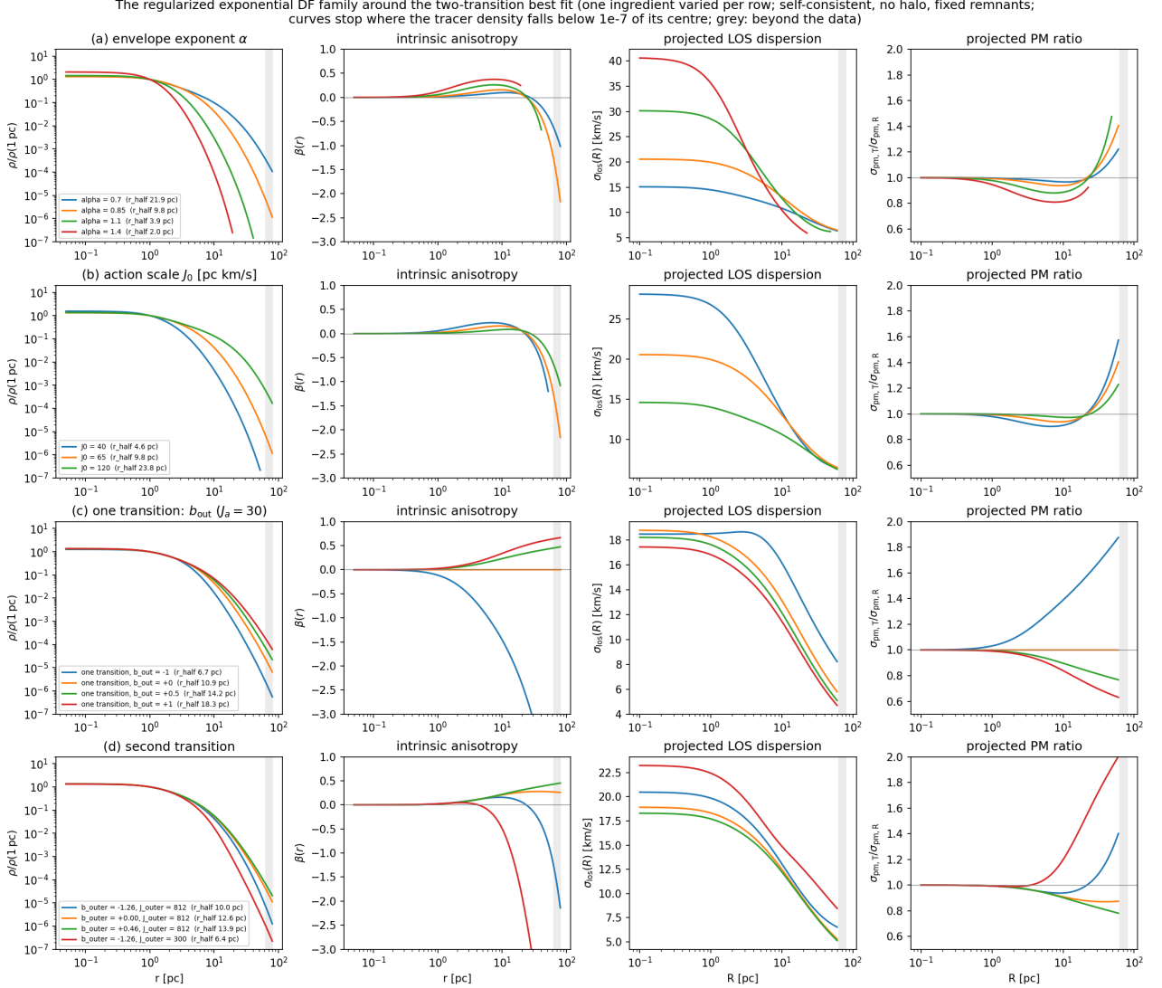
Figure 1: The regularized exponential DF family around the two-transition best fit. Rows vary (a) \alpha , (b) J_0 , (c) a single anisotropy transition with amplitude b_{\text{out}} at J_a = 30 \text{ pc km s}^{-1} , and (d) the second transition ( b_{\text{outer}}, J_{\text{outer}} ). All other parameters stay at the best-fit values. Columns: intrinsic density normalized at 1 pc (legend: half-mass radius); intrinsic \beta(r) ; projected \sigma_{\text{los}}(R) ; projected \sigma_{\text{pm},T}/\sigma_{\text{pm},R} . Every model is a self-consistent equilibrium in the fitted remnant potential (no halo, no point mass). Curves stop where the tracer density falls below 10^{-7} of its central value. Grey marks radii beyond the data. These are illustrations, not fits (script bin/plot_df_family_gallery.py ).
