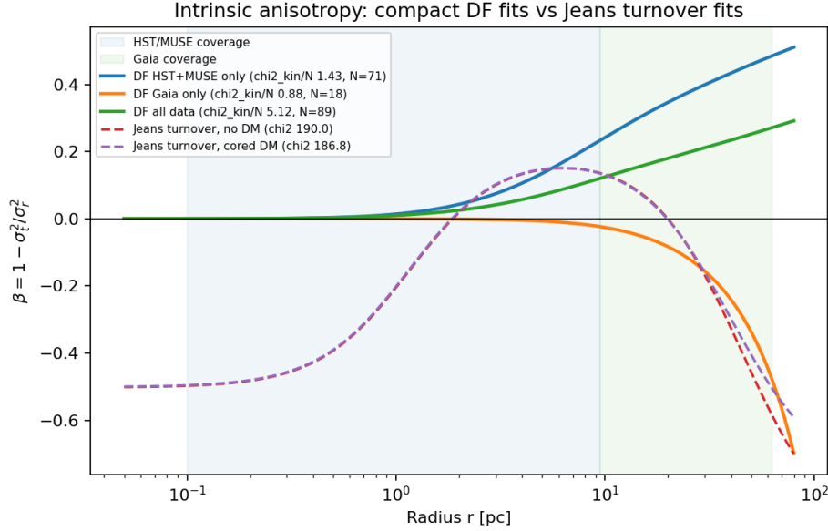
Figure 3: Intrinsic anisotropy \beta(r) of the one-transition DF fitted to HST+MUSE only, to Gaia only, and to all data, compared with the rung-2 Jeans turnover fits. Shading marks the radial coverage of the two surveys.
