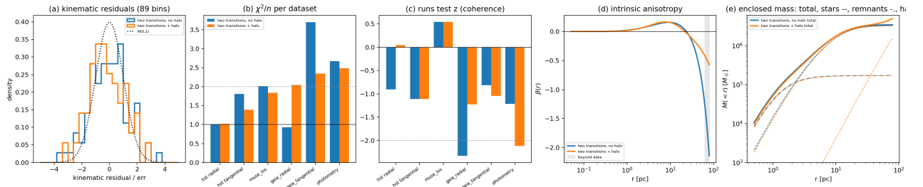
Figure 8: Diagnostics of the two best fits: (a) kinematic residuals against N(0,1) ; (b) \chi^2/n per dataset; (c) runs-test z per dataset; (d) intrinsic \beta(r) ; (e) enclosed mass by component (total, stars, remnants, halo).
