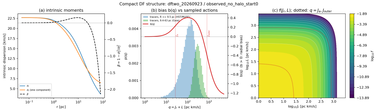
Figure 5: Structure of the two-transition fit (no halo). (a) Intrinsic \sigma_r , one-component \sigma_t and \beta(r) . (b) The bias b(q) over the q distributions of tracers in the HST/MUSE and Gaia projected ranges. (c) \log_{10} f in the (J_r, L) plane ( J_z = 0 ); dotted lines mark q = J_a and q = J_{outer} .
