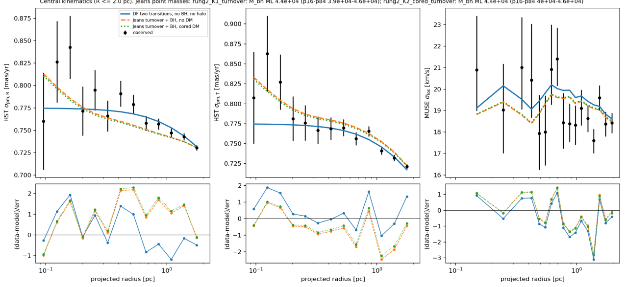
Figure 8: Central kinematics ( R \leq 2 pc) with the no-BH two-transition DF and the Jeans turnover fits with a point mass. Bottom: (\text{data} - \text{model})/\text{error} .
