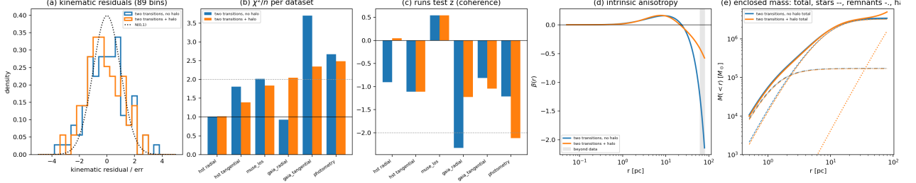
Figure 7: Diagnostics of the two best fits: (a) kinematic residuals against N(0,1) ; (b) \chi^2/n per dataset; (c) runs-test z per dataset; (d) intrinsic \beta(r) ; (e) enclosed mass by component (total, stars, remnants, halo).
