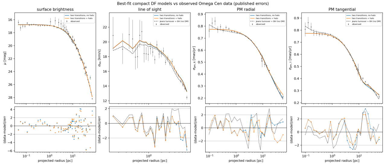
Figure 6: Best two-transition fits without (blue) and with (orange) a halo, and the rung-2 Jeans turnover fit (dashed; kinematics only). Bottom: (data–model)/error, with \pm 2 lines.
