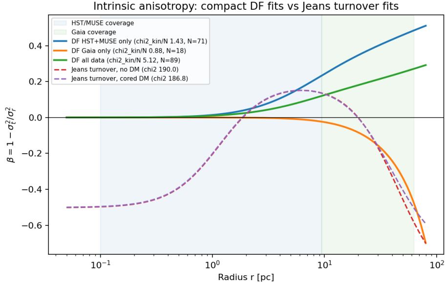
Figure 2: Intrinsic anisotropy \beta(r) of the one-transition DF fitted to HST+MUSE only, to Gaia only, and to all data, compared with the rung-2 Jeans turnover fits. Shading marks the radial coverage of the two surveys.
