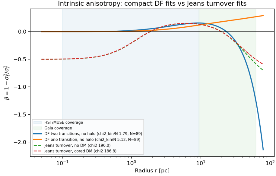
Figure 4: Intrinsic anisotropy of the two-transition fit (no halo) against the one-transition fit and the Jeans turnover fits.
