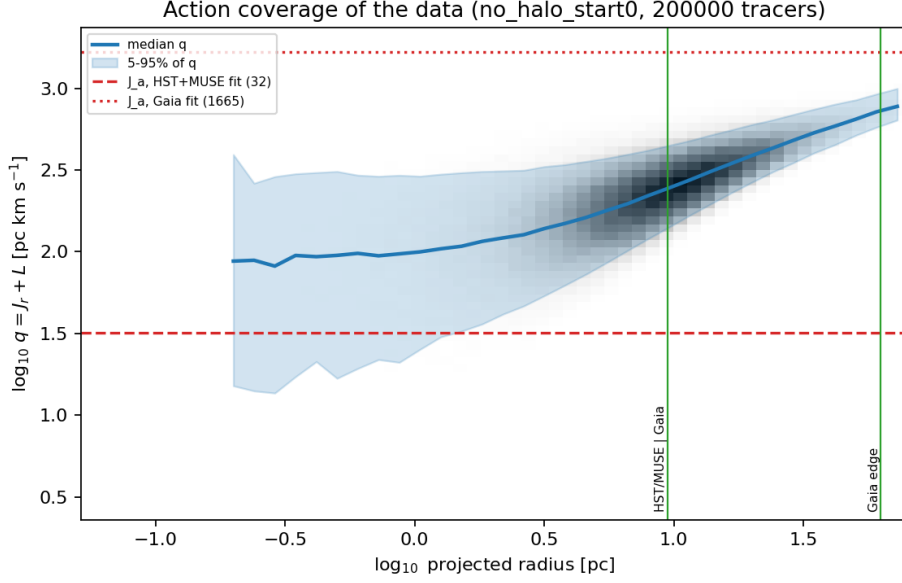
Figure 3: Distribution of q = J_r + L of DF tracers against projected radius, with 5–95% quantiles. Horizontal lines mark the J_a of the HST+MUSE-only (32) and Gaia-only (1665) fits.
