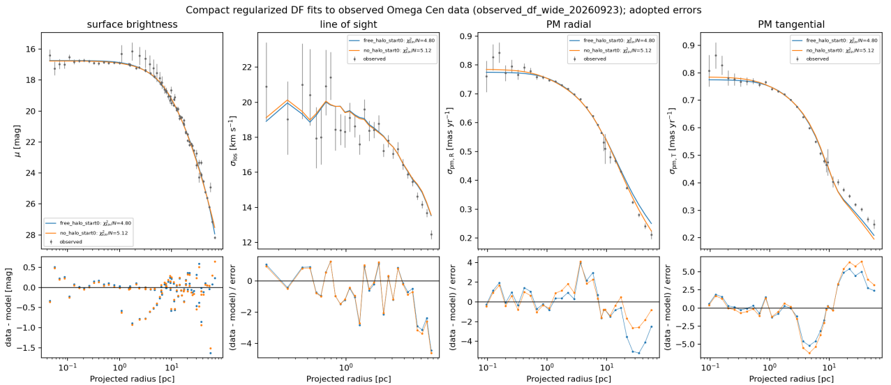
Figure 1: Best one-transition fits (wide bounds) with and without a halo. Top: surface brightness, LOS and PM dispersions with published errors. Bottom: normalized residuals (data−model)/error.
