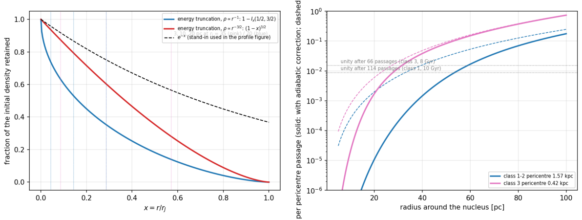
Figure 2: Left: fraction of the initial density retained after energy truncation at \Phi(r_J) in a Kepler potential for \rho \propto r^{-1} and r^{-3/2} tracers, against the e^{-x} stand-in; dotted lines mark 3, 10, 20 pc for r_J = 35 and 70 pc. Right: heating per pericentre passage versus radius around the nucleus for the class-1/2 and class-3 pericentres, with (solid) and without (dashed) the adiabatic correction; the horizontal lines mark the level at which the cumulative heating over the reconstructed number of passages reaches unity.
