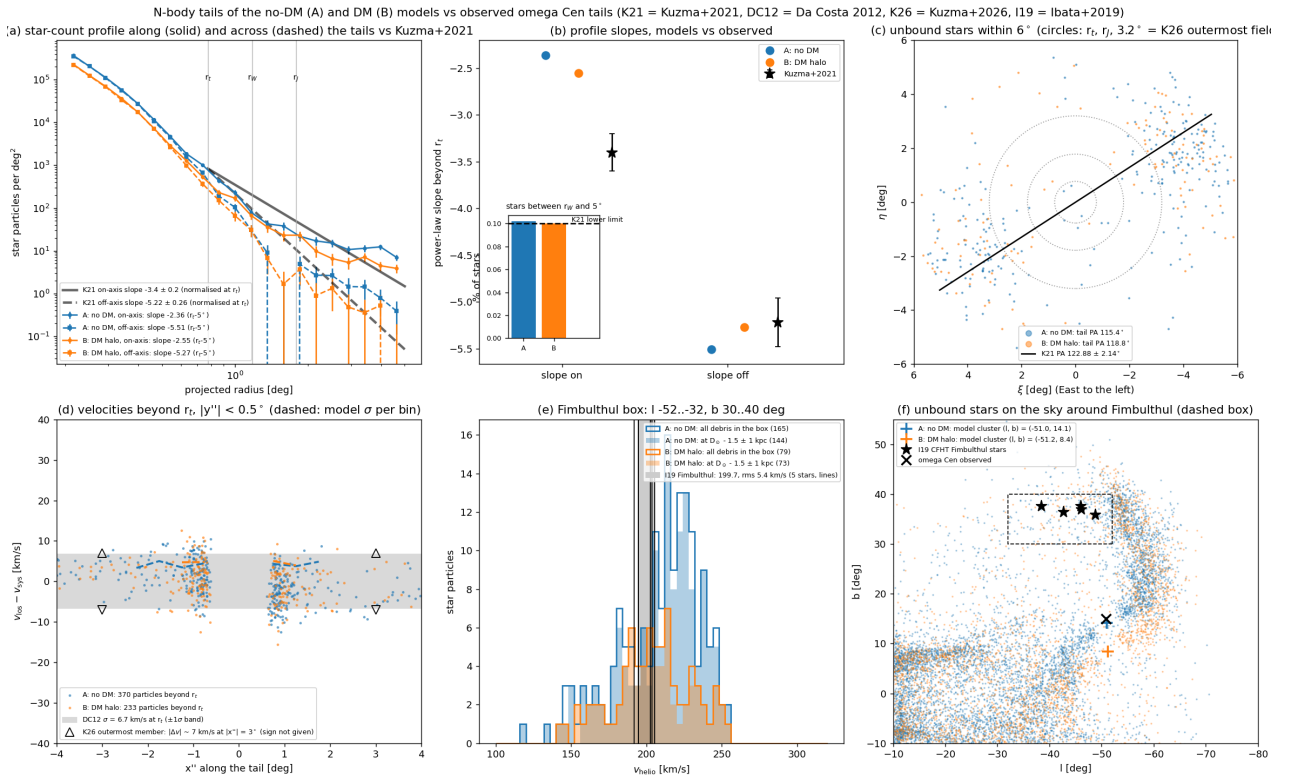
Figure 25: Models against the observed tails: (a,b) star-count profiles along and across the tails and their slopes beyond r_t with the Kuzma et al. (2021) values, and the stellar fraction between the Wilson radius and 5^\circ ; (c) unbound stars in the tangent plane with the observed tail direction; (d) line-of-sight velocities beyond r_t with the Da Costa (2012) dispersion and the outermost Kuzma et al. (2026) member; (e,f) the Fimbulthul box ( l = -52^\circ to -32^\circ , b = 30^\circ\text{--}40^\circ ) with the five Ibata et al. (2019) velocities. Panel (e) compares unlike populations (see Figure 26).
