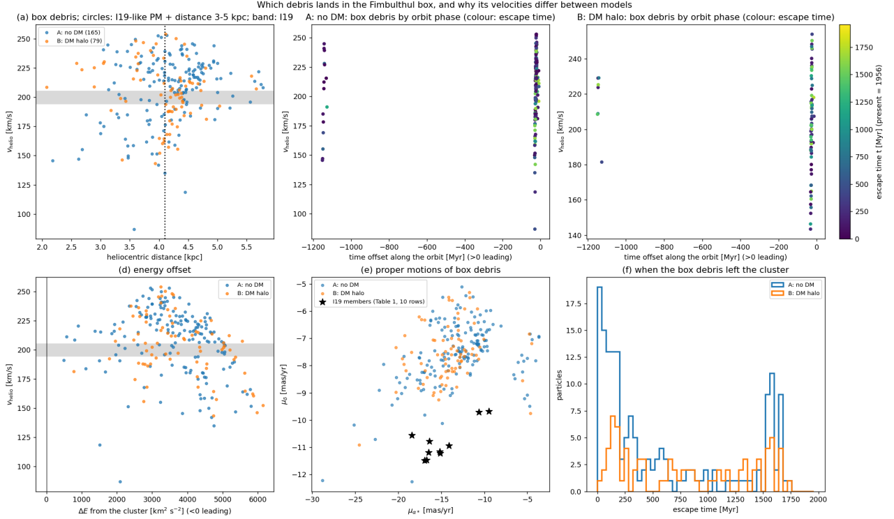
Figure 26: Model debris in the Fimbulthul box: velocity against distance (circles would mark particles passing an Ibata-like selection; there are none), against orbit phase coloured by escape time, and against energy offset; proper motions with the observed members (stars); escape-time distributions.
