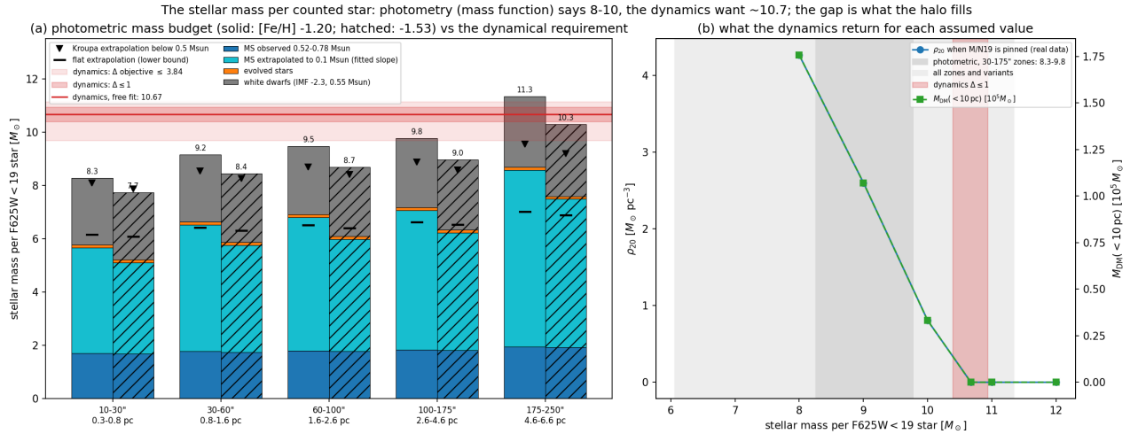
Figure 14: (a) Photometric mass per F625W < 19 star by component and zone (solid: [\text{Fe}/\text{H}] = -1.20 ; hatched: -1.53 ; markers: Kroupa and flat extrapolations) against the dynamical value (red line: free fit 10.67; bands: \Delta \leq 1 [10.39, 10.94] and \Delta \leq 3.84 [9.68, 11.14] from the scan of Section 6.5). (b) \rho_{20} and M_{\text{DM}}(< 10 \text{ pc}) returned by the real-data scan for each pinned value, with the photometric ranges shaded.
