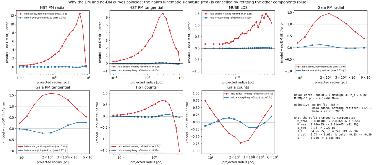
Figure 17: (Model – no-DM fit)/error per bin for a \rho_{20} = 1 , r_s = 5 pc halo added with nothing refitted (red) and with every other parameter refitted (blue). The text panel lists the compensating changes.
