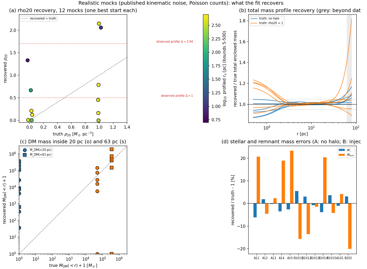
Figure 12: Recovery in twelve realistic mocks. (a) Recovered against true \rho_{20} (colour: profiled r_s ); the red lines mark where the observed profile crosses \Delta = 1 and 3.84. (b) Recovered/true total enclosed mass against radius (grey: beyond the data). (c) Recovered against true DM mass inside 20 and 63 pc. (d) Fractional errors of the stellar and remnant masses.
