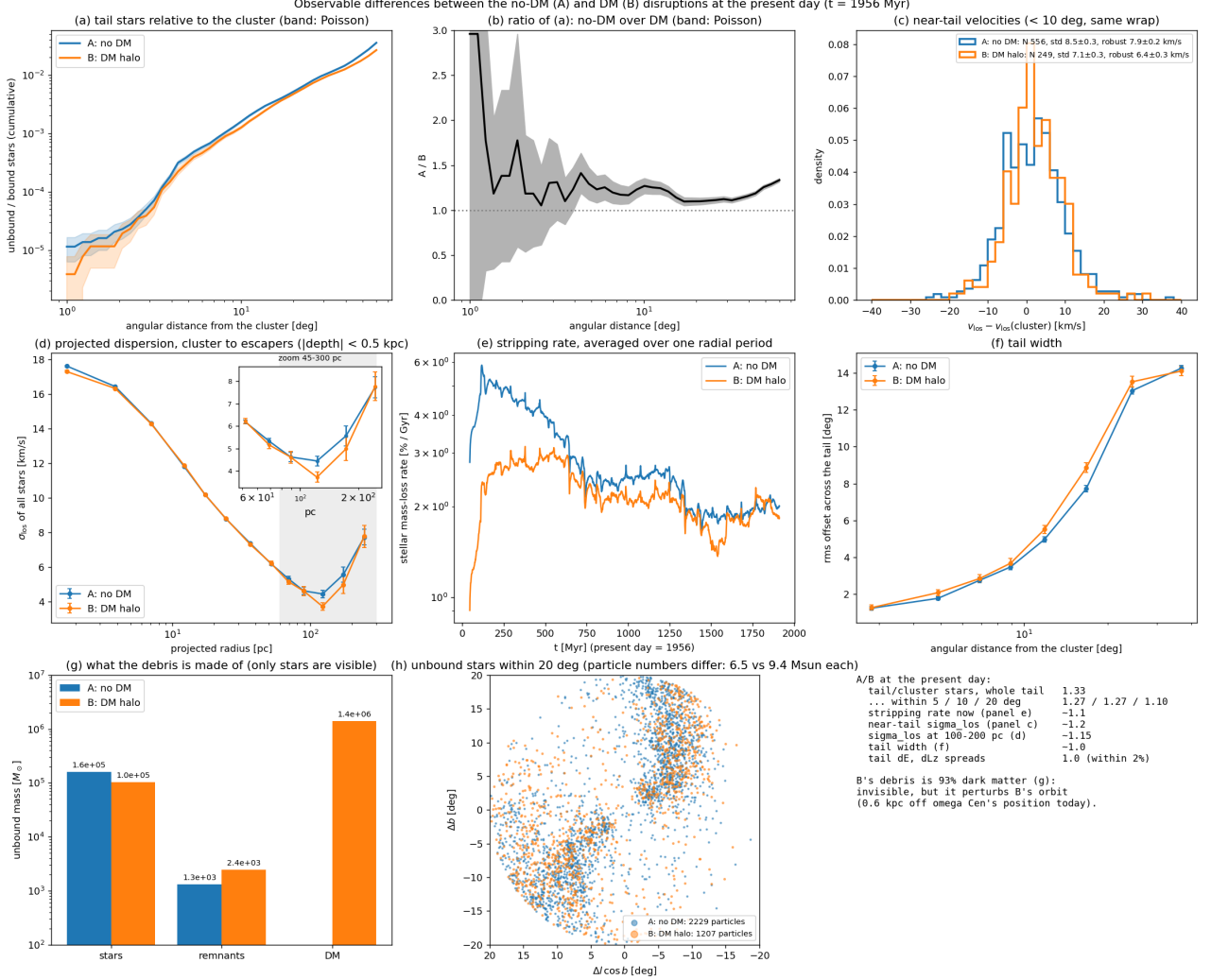
Figure 23: Observable differences today: (a,b) cumulative tail/cluster star ratio and its A/B ratio against angular distance (Poisson bands); (c) near-tail line-of-sight velocities (same wrap, < 10^\circ ); (d) projected dispersion from the cluster to the escapers; (e) stripping rate per radial period; (f) tail width; (g) debris composition; (h) near-tail sky map; (i) summary of the ratios.
