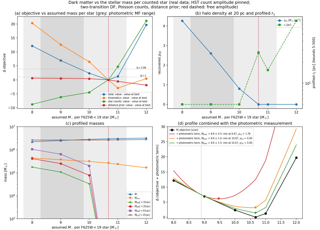
Figure 16: Real data against the assumed stellar mass per counted star. (a) Objective and components relative to the minimum (grey: photometric range). (b) \rho_{20} and the profiled r_s . (c) Profiled masses. (d) The scan combined with the photometric term for \sigma_{\text{phot}} = 0.5, 1.0 and 1.5 (triangles: minima).
