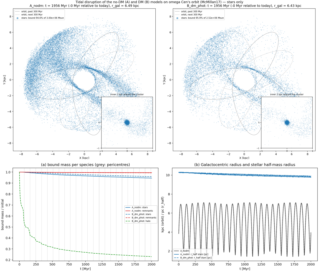
Figure 22: Top: stars of model A (left) and B (right) today in the Galactocentric X - Y plane, with the orbit over \pm 300 Myr and the inner 2 kpc as an inset. Bottom: bound mass per species against time (grey: pericentres; the present day is t = 1955.6 Myr) and the Galactocentric radius and stellar half-mass radius.
