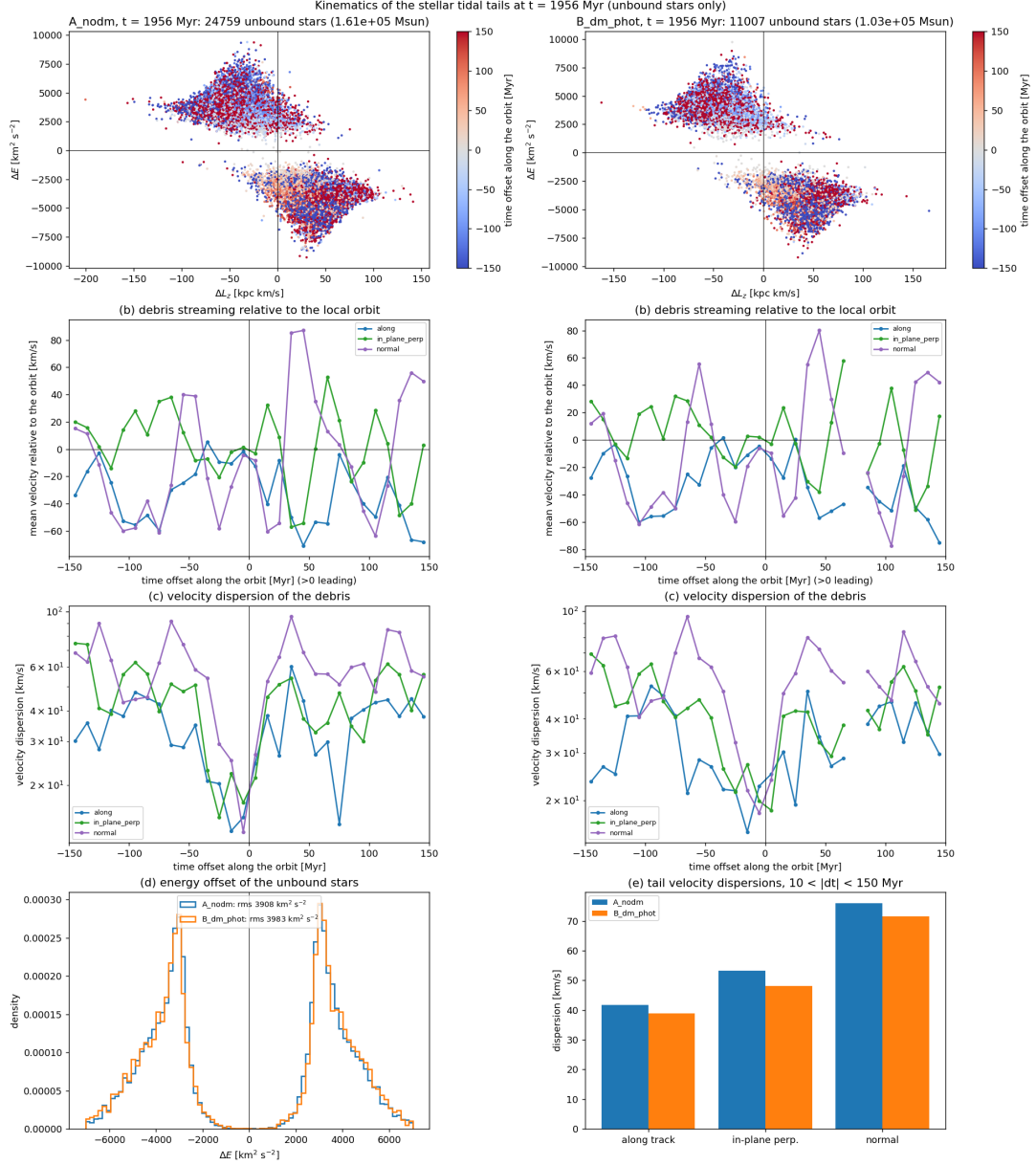
Figure 24: Kinematics of the unbound stars today: energy against L_z offset from the cluster (colour: time offset along the orbit), streaming and dispersions relative to the local orbit along the tails, the \Delta E distributions of both models and the tail dispersions per component (these mix orbital wraps within \pm 150 Myr and are therefore large).
