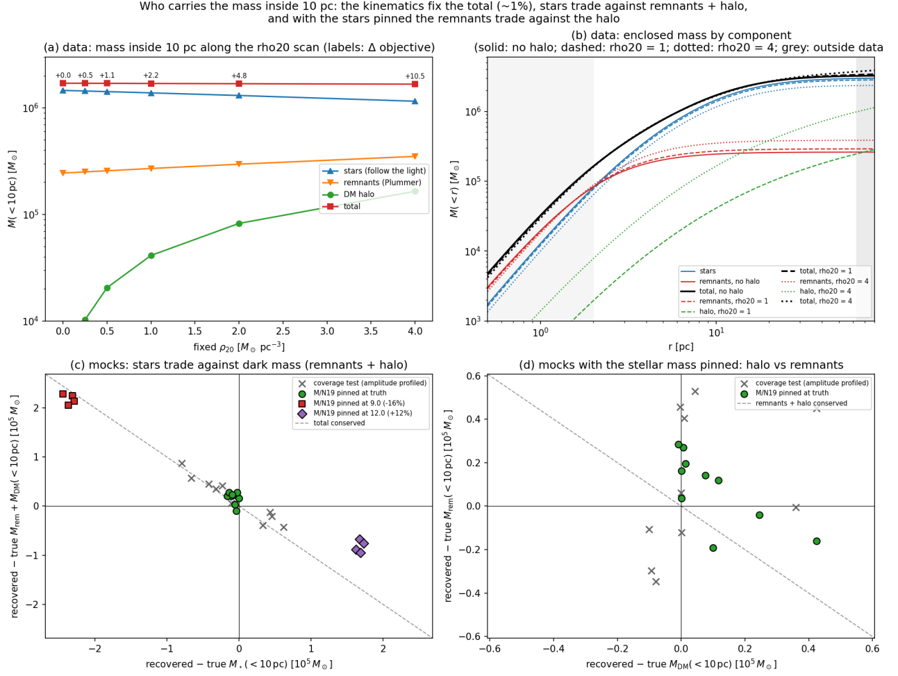
Figure 18: (a) Data: mass inside 10 pc per component along the \rho_{20} scan (labels: \Delta objective). (b) Enclosed-mass profiles for \rho_{20} = 0, 1 and 4 . (c) Mocks: error of the stellar mass against the error of remnants plus halo inside 10 pc. (d) Mocks with the stars pinned: halo against remnant error.
