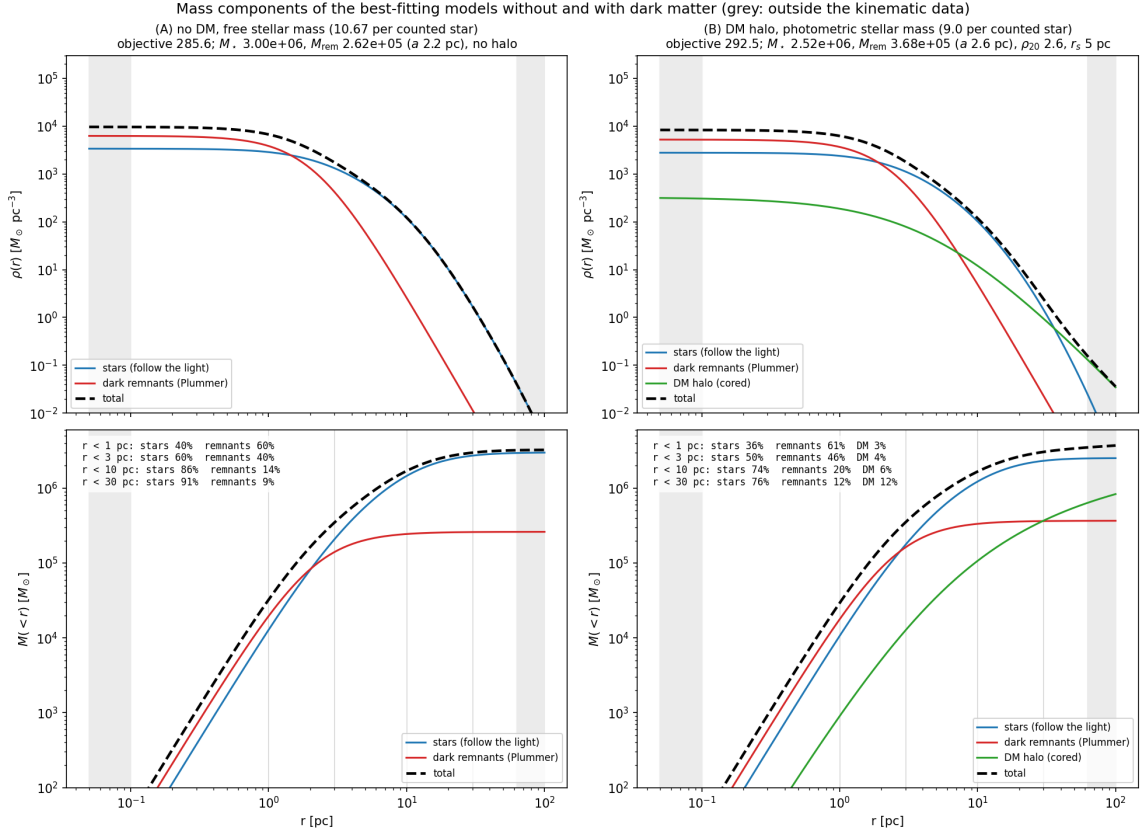
Figure 20: Density (top) and enclosed mass (bottom) of stars, remnants and halo for model A (left) and model B (right). Grey: outside the kinematic data (inside 0.1 pc and beyond 63 pc).
