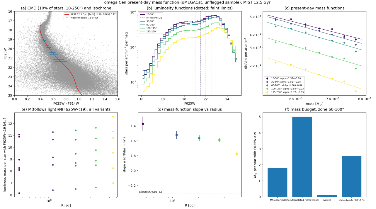
Figure 13: Present-day mass function from oMEGACat: colour–magnitude diagram with the adopted isochrone, luminosity and mass functions per zone, slope against radius (common faint limit F625W < 21 ), and the mass per counted star for the extrapolation and white-dwarf variants.
