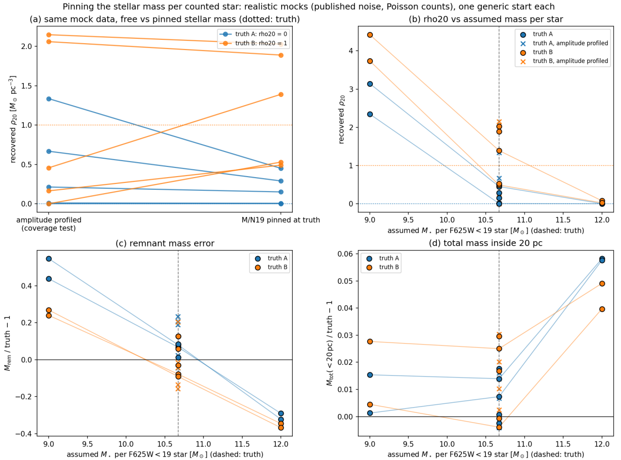
Figure 15: Mocks with the stellar mass per counted star pinned. (a) Same mock data, amplitude profiled (coverage test) against pinned at the truth. (b)–(d) Recovered \rho_{20} , remnant-mass error and M(< 20 \text{ pc}) error against the assumed M/N_{19} (truth 10.67, dashed).
