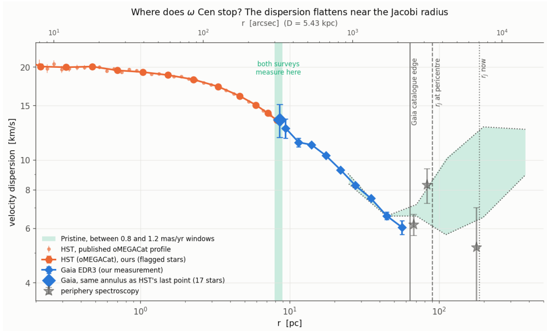
Figure 5: The profile from the centre to 400 pc. The dispersion stops falling near 50–100 pc, where the pericentric Jacobian radius lies.
