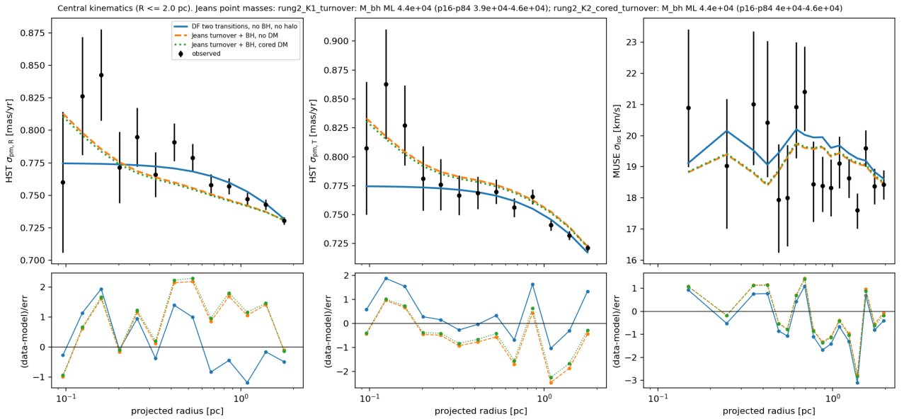
Figure 9: Central kinematics ( R \leq 2 pc) with the no-BH two-transition DF and the Jeans turnover fits with a point mass. Bottom: (data–model)/error.
