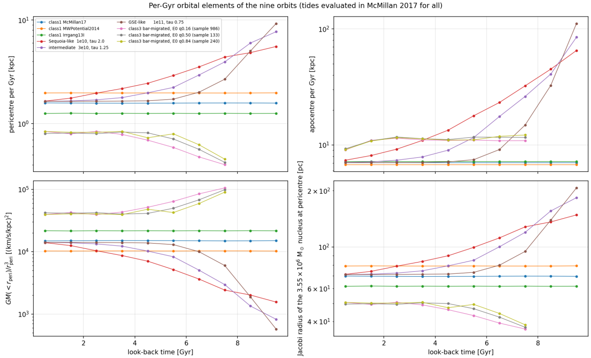
Figure 10: Per-Gyr orbital elements of the nine orbits: pericentre, apocentre, tidal-field strength GM(< r_{\text{peri}})/r_{\text{peri}}^3 at pericentre, and the Jacobi radius a 3.55 \times 10^6 M_\odot nucleus would have there. Enclosed masses from McMillan (2017) for all orbits, including class 3 (integrated in Hunter et al. 2024), for a uniform proxy.
