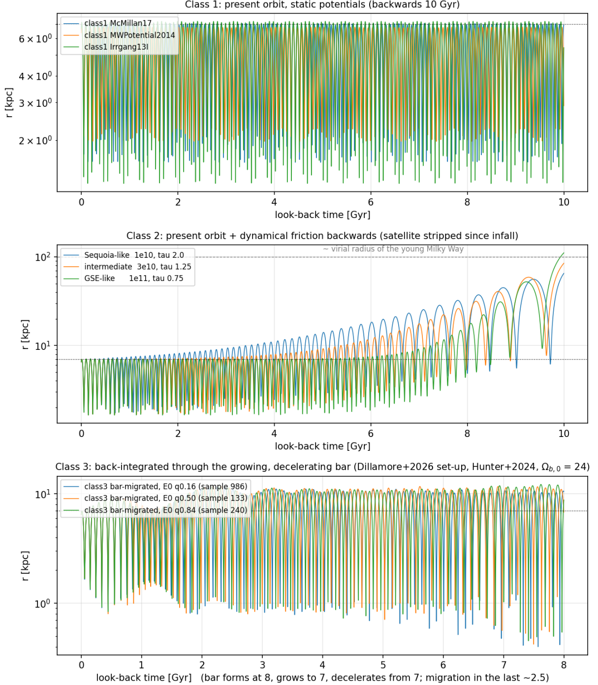
Figure 8: Overview of the nine orbits: galactocentric radius against look-back time for classes 1 (top), 2 (middle; dashed line 100 kpc) and 3 (bottom). Dotted line: today's apocentre, 7 kpc.
