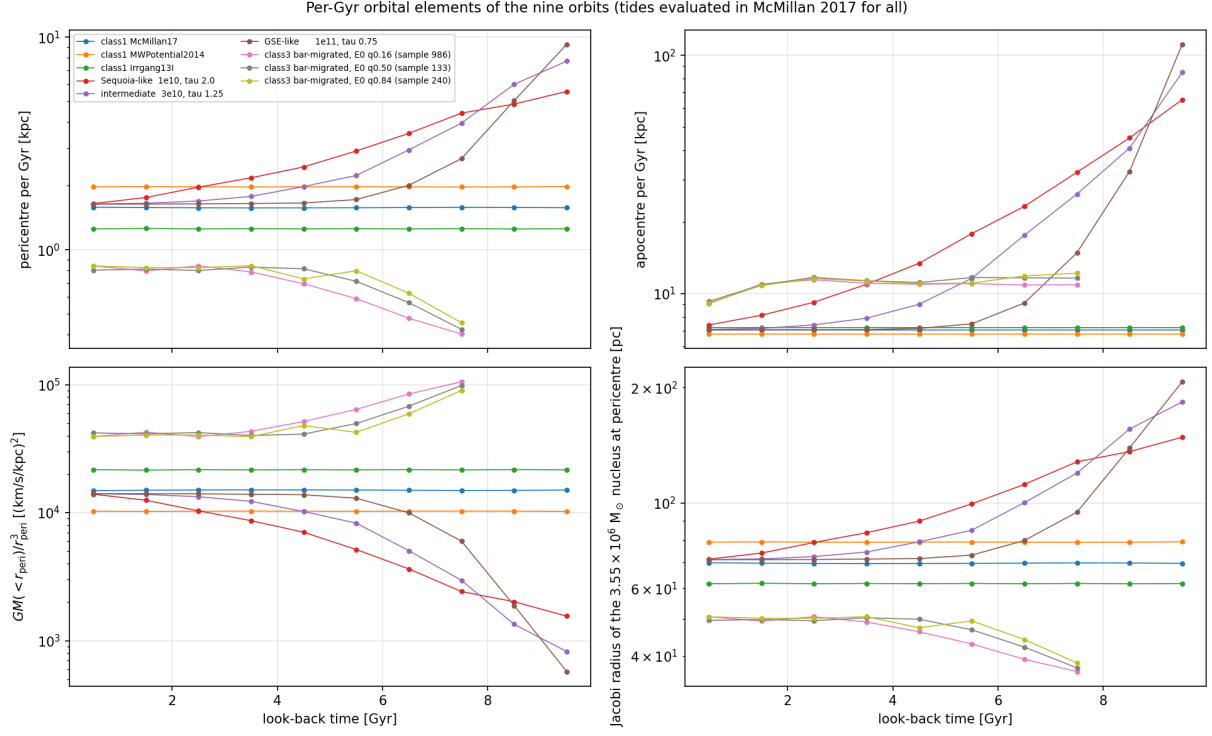
Figure 9: Per-Gyr orbital elements of the nine orbits: pericentre, apocentre, tidal-field strength GM(< r_{\text{peri}})/r_{\text{peri}}^3 at pericentre, and the Jacobi radius a 3.55 \times 10^6 M_{\odot} nucleus would have there. Enclosed masses from McMillan (2017) for all orbits, including class 3 (integrated in Hunter et al. 2024), for a uniform proxy.
