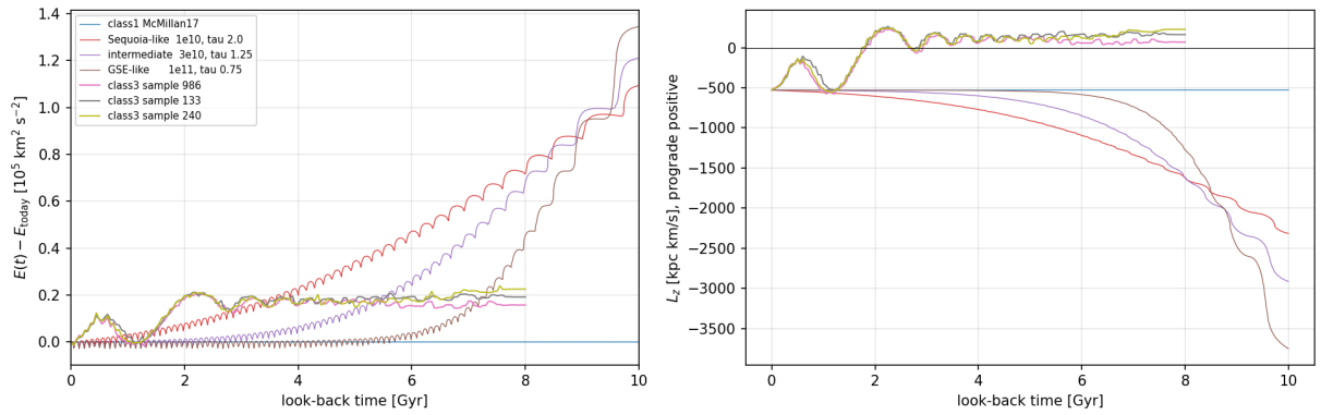
Figure 10: Energy relative to today (left; each orbit in its own host potential) and L_z (right, prograde-positive) against look-back time. Class 1 (McMillan 2017 only) is flat by construction; class 2 climbs steadily as friction is undone; class 3 is flat at GSE values until the resonance moves it in the last 2.5 Gyr. Note the opposite directions of the L_z change: friction makes the early orbit more retrograde, the bar makes it less .
