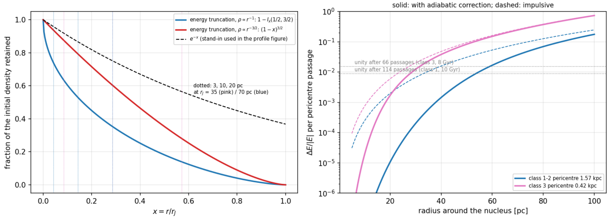
Figure 2: Left: fraction of the initial density retained after energy truncation at \Phi(r_J) in a Kepler potential for \rho \propto r^{-1} and r^{-3/2} tracers, against the e^{-x} stand-in; dotted lines mark 3, 10, 20 pc for r_J = 35 and 70 pc. Right: heating per pericentre passage versus radius around the nucleus for the class-1/2 and class-3 pericentres, with (solid) and without (dashed) the adiabatic correction; the horizontal lines mark the level at which the cumulative heating over the reconstructed number of passages reaches unity.
