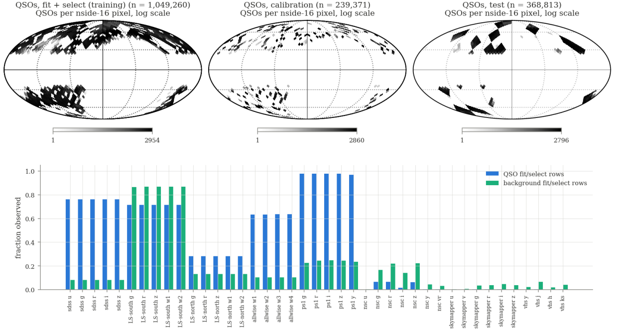
Figure 3: Top: sky distribution of quasars by role, Galactic Mollweide projection, counts per HEALPix nside-16 pixel (log scale). Bottom: fraction of fit/select rows with each band observed, for quasars (blue) and the background (aqua).
