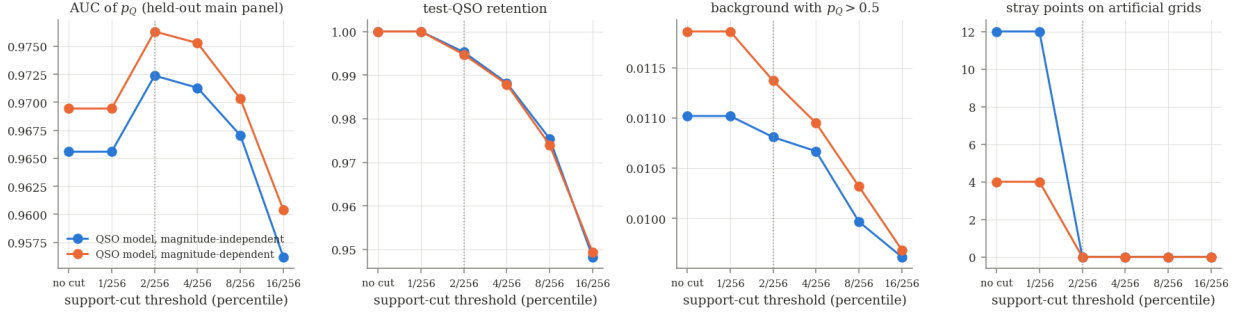
Figure 10: Support-cut threshold (percentile; dotted: the calibrated 2/256 ) on the held-out main panels of Section 10.3 and the artificial grids of Section 10.4: AUC of p_{\text{quasar}} (the scorer does not compute \log \mathcal{R} for rejected objects, so p_{\text{quasar}} ranks all thresholds alike; unranked objects at the bottom), fraction of test quasars kept, fraction of background objects with p_{\text{quasar}} > 0.5 , and grid points with p_{\text{quasar}} > 0.5 in the low-density mask.
