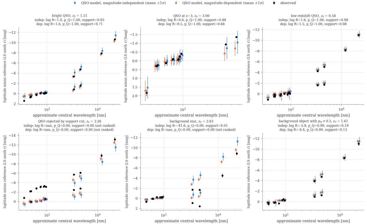
Figure 19: Worked examples: observed luptitude minus reference-band luptitude (black) and each model's conditional prediction at the object's redshift (mean \pm 1\sigma ; blue magnitude-independent, or orange magnitude-dependent). Horizontal positions are approximate central wavelengths, for display only. Titles give \log \mathcal{R} , p_{\text{quasar}} and the support percentile from both models. Object identifiers are in docs/method_unified/examples.json.
