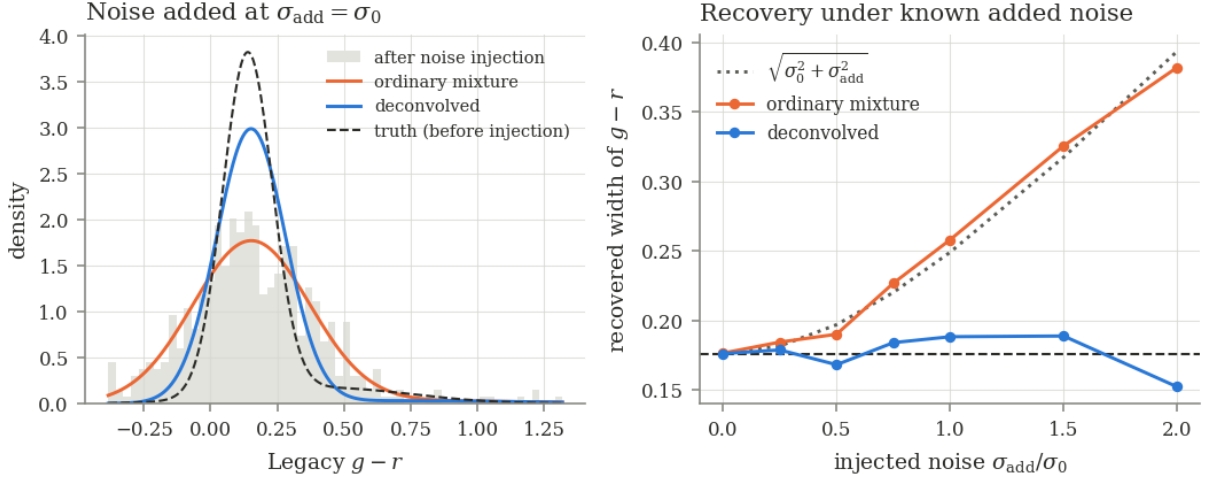
Figure 2: Deconvolution tested by controlled noise injection on real quasar colours: Legacy g - r of the 473 bright quasars ( u_r < 20 , |z - 1.8| < 0.15 ) of the training draw, whose measurement errors are small; fitted width \sigma_0 = 0.176 . Gaussian noise of known size is added and a two-component mixture refitted. Left : at \sigma_{\text{add}} = \sigma_0 the deconvolved mixture (blue) stays close to the pre-injection truth (dashed) while the ordinary mixture (orange) is broadened. Right : the ordinary mixture follows \sqrt{\sigma_0^2 + \sigma_{\text{add}}^2} , reaching 0.382 at \sigma_{\text{add}} = 2\sigma_0 ; extreme deconvolution stays within 8% of \sigma_0 up to 1.5\sigma_0 and returns 0.152 (14% low) at 2\sigma_0 , where the sample of 473 is small for the added noise.
