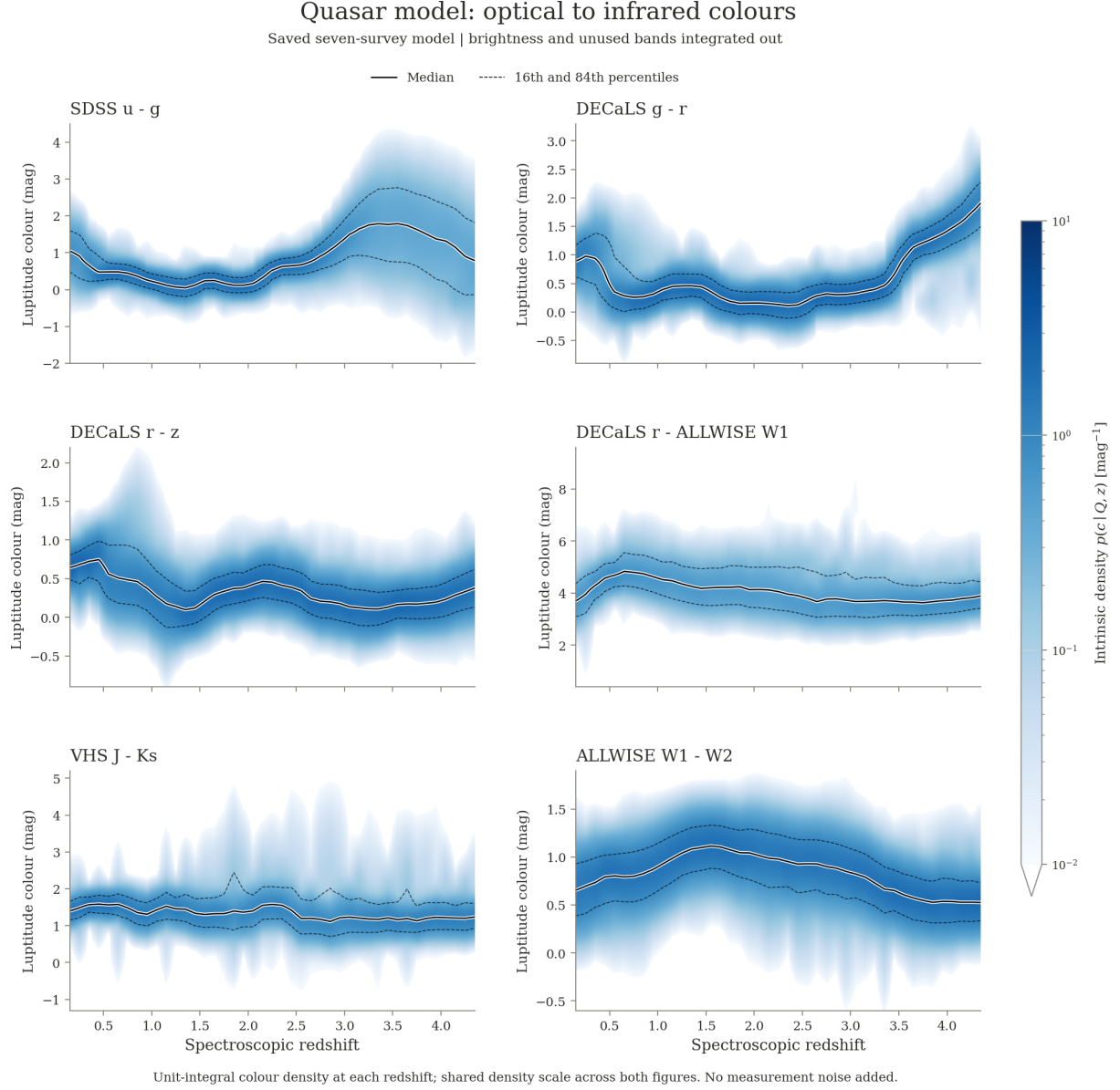
Figure 5: Intrinsic quasar colour densities from the model: SDSS u - g , Legacy g - r and r - z , Legacy r - \text{AllWISE } W1 , VHS J - K_s and AllWISE W1 - W2 . Brightness and all unused bands are marginalised; no measurement noise is added. Each redshift column is a unit-integral colour density, per magnitude; solid curves are medians and dashed curves the 16th and 84th percentiles. The density scale is shared with Figure 6.
