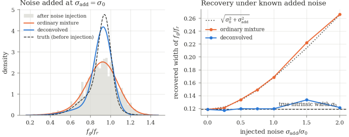
Figure 1: Deconvolution tested by controlled noise injection on real quasar colours (Legacy f_g/f_r of bright quasars near z = 1.8 , N = 1536 , r < 20 , whose measurement errors are negligible; fitted width \sigma_0 = 0.119 ). Gaussian noise of known size is added and the models refitted. Left: at \sigma_{\text{add}} = \sigma_0 the deconvolved mixture (blue) recovers the pre-injection truth (dashed) while the ordinary mixture (orange) is broadened. Right: the ordinary mixture follows \sqrt{\sigma_0^2 + \sigma_{\text{add}}^2} , reaching 0.266 at \sigma_{\text{add}} = 2\sigma_0 ; extreme deconvolution returns 0.122. The test is of the algorithm, and was run in the predecessor’s flux-ratio coordinates (Appendix C).
