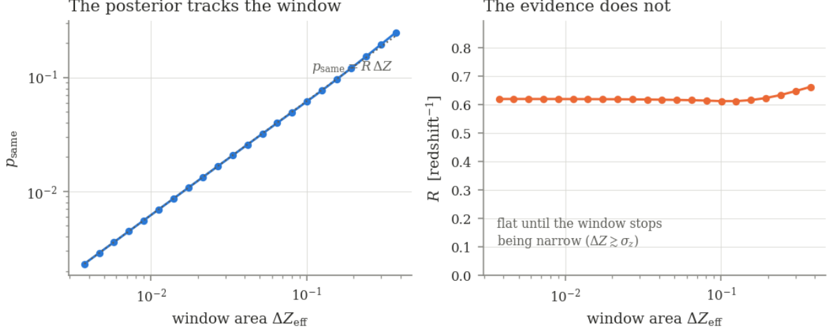
Figure 5: The factorisation on a real quasar. Left : p_{\text{same}} is proportional to the window area over more than a decade, as (17) requires; the dotted line is R \Delta Z with R from the narrowest window. Right : R is flat until the window stops being narrow compared with \sigma_z . Computed with the predecessor model; the factorisation is a property of (1)–(15), not of a particular density.
