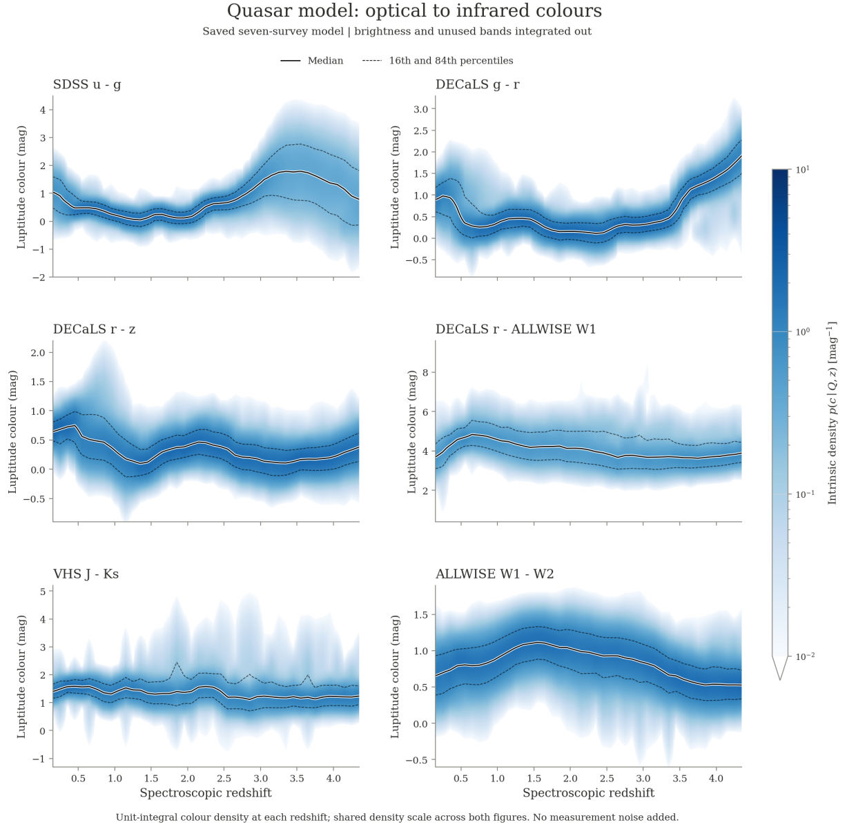
Figure 2: Intrinsic quasar colour densities from the model: SDSS u - g , Legacy g - r and r - z , Legacy r - \text{AllWISE } W1 , VHS J - K_s and AllWISE W1 - W2 . Brightness and all unused bands are marginalised; no measurement noise is added. Each redshift column is a unit-integral colour density, per magnitude; solid curves are medians and dashed curves the 16th and 84th percentiles. The density scale is shared with Figure 3.
