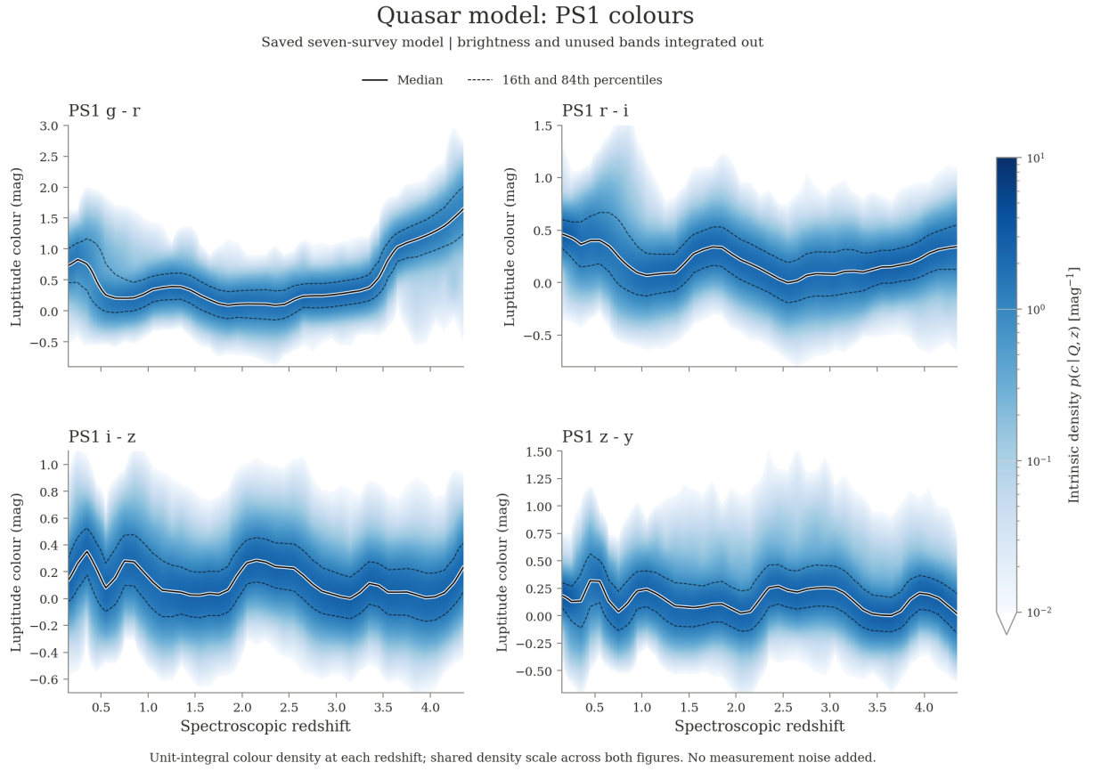
Figure 3: The four adjacent PS1 colours, g - r , r - i , i - z and z - y , against redshift, drawn as in Figure 2. These use the separately labelled PS1 bands; they are not Legacy colours relabelled.
