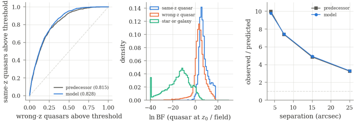
Figure 7: The labelled pairs, scored from Legacy g, r, z, W1, W2 . Left : ROC for same- against wrong-redshift quasar companions in the reserved sky blocks, ranked by \ln R , for the model and its predecessor (AUC in brackets). Centre : the Bayes factor for the three classes (values below -40 are piled at -40 ); the non-quasar class mixes stars with the galaxies DESI targeted. Right : the observed same-redshift fraction among quasar companions divided by the mean predicted p(z \in W \mid \mathbf{u}, Q) , by separation. A defect in the scorer would give a flat ratio; physical clustering gives one that falls with separation.
