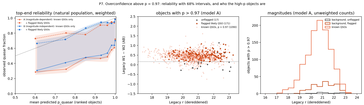
Figure 9: Left: observed quasar fraction against mean predicted p_{\text{quasar}} for ranked objects of the natural test-cone population, counting known quasars only (solid, lower bound) or also flagged likely quasars (dashed, upper bound); shading: 68% Wilson intervals of the two bounds. Middle: Legacy W1 - W2 (AB) against r for objects with p_{\text{quasar}} > 0.97 under model A: known quasars (light), flagged background objects (dark orange) and unflagged ones (black). Dotted: the WISE AGN threshold ( W1 - W2 = 0.8 Vega). Right: their r distributions (unweighted).
