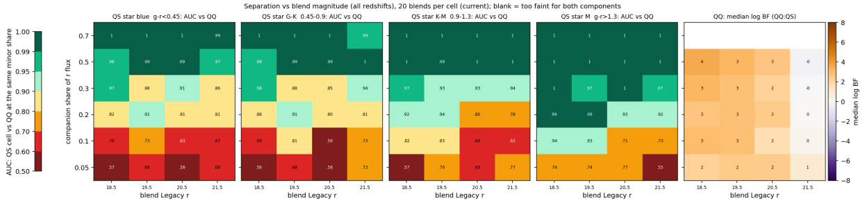
Figure 24: As Fig. 23, against blend Legacy r , with quasar redshifts drawn from the whole test sample.
