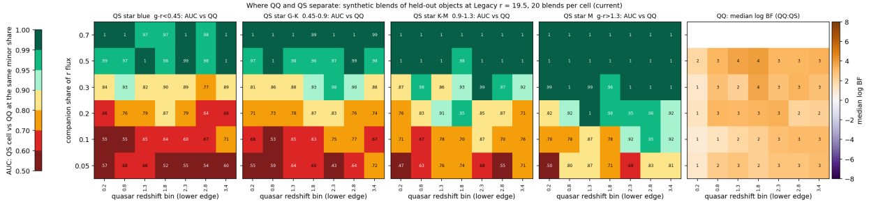
Figure 23: Where QQ and QS separate, at blend Legacy r = 19.5 . First four panels: AUC of log BF between QS blends with a companion of the given g-r stratum and QQ blends at the same minor share, by quasar redshift and companion share of the r flux (20 blends per class per cell, current). Last panel: median log BF of the QQ blends (minor shares up to 0.5).
